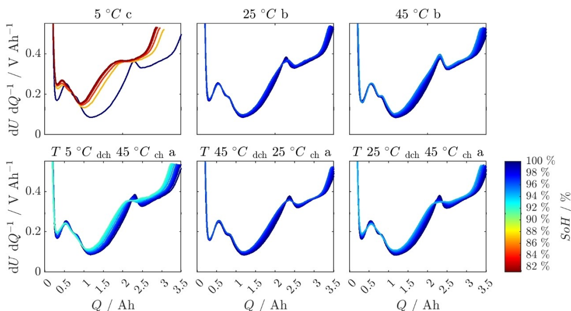
Figure 3. DVA in charge direction over SoH for the steady-state cells (5 °C c, 25 °C b and 45 °C b), the potential aging acceleration condition ( T 5\text{ }^{\circ}\text{C}_{\text{dch}} 45\text{ }^{\circ}\text{C}_{\text{ch}} a) and the transient cells T 45\text{ }^{\circ}\text{C}_{\text{dch}} 25\text{ }^{\circ}\text{C}_{\text{ch}} a and T 25\text{ }^{\circ}\text{C}_{\text{dch}} 45\text{ }^{\circ}\text{C}_{\text{ch}} a with an equivalent aging temperature higher than 25 °C.
