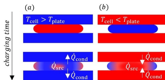
Figure 5. Schematic illustration of the temperature field during the temperature change for two scenarios; cell has a higher (red) (a) or lower (blue) (b) temperature than the cooling plate.
