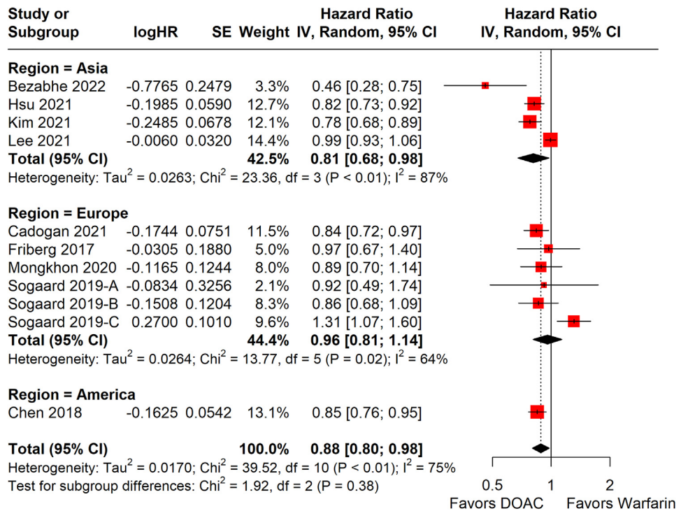
FIGURE 2 Random-Effects Meta-Analysis of HR for Dementia Development
