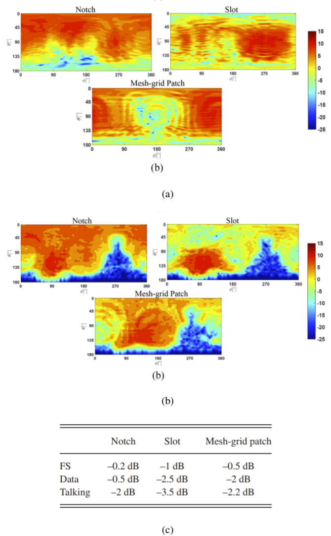
FIGURE 8: Radiation pattern of antennas in free space in (a), with the user in (b), and the measured body loss of different antennas in (c). [30]
