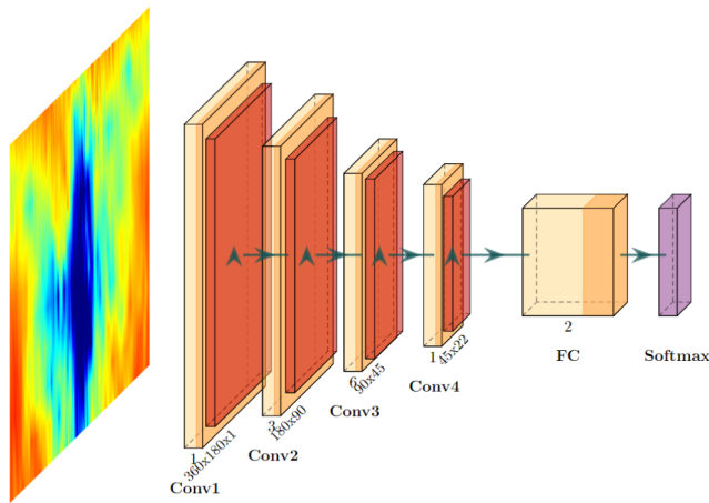
FIGURE 15: A simple deep learning network architecture.
