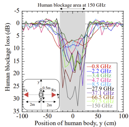
FIGURE 13: The user blockage measured in the anechoic chamber. [35]
