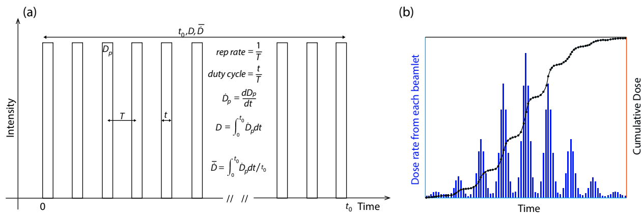
Fig. 1. (a) Schematic of electron temporal pulse structures of extracted beams with key parameters defined. (b) Dose rates and cumulative doses from each spot on a square field of proton pencil beam scanning delivery to the Bragg peak (central axis). The spots are of the same intensity and energy and are uniformly spaced. See Table 1 for variable definitions.
