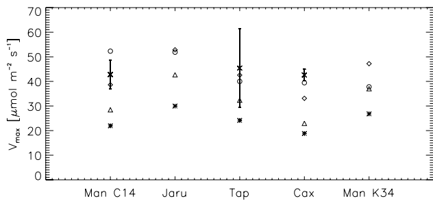
Fig. 6. Top leaf V_{max} . Obtained from numerical fitting in this study are circles, measured at Manaus C14, Tapajos and Caxiuana, crosses, calculated from linear regression between measured V_{max} and leaf N at 3 at different canopy levels at 3 of the studied sites: Manaus C14 (Carswell et al., 2000), Caxiuana (Vale et al., 2000) and Tapajos (Domingues et al., 2005) (asterisks, triangles and rhombuses sign, respectively). See linear regressions used for calculations of V_{max} in Table B1.
