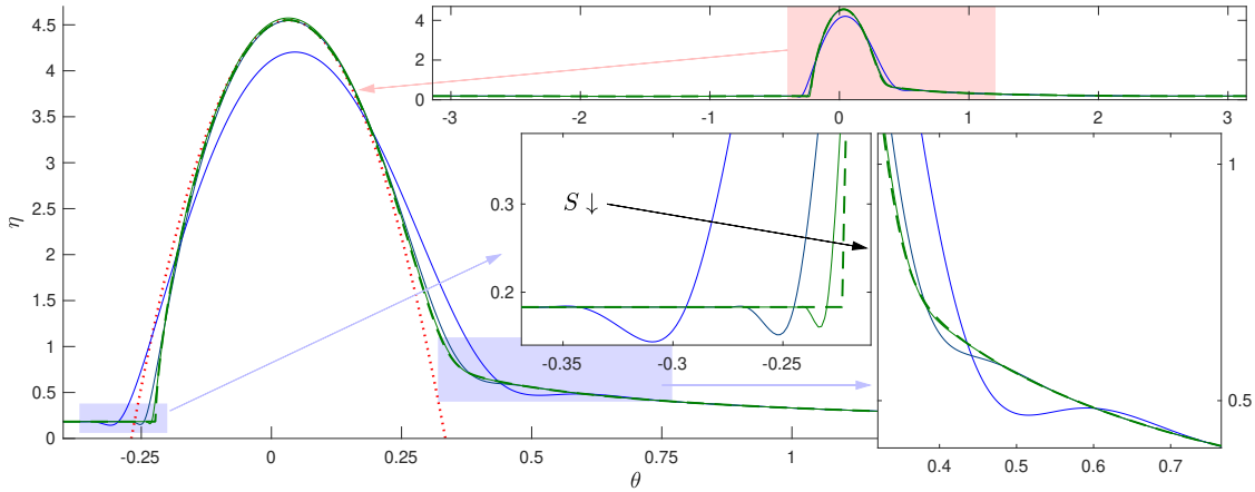
FIG. 5. Steady solutions with S = 10^{-4}, 10^{-5} and 10^{-6} (solid, from blue to green), for (\Lambda, \text{Bi}, n, f) = (10, 0.1, 1, 0.01) . The dashed line shows the construction of the Appendix for S = 0 . The dotted line shows the approximation (38). The main panel shows the pool solutions; the insets show the entire solutions and magnifications near the borders of the pool (as indicated by the shading and arrows).
