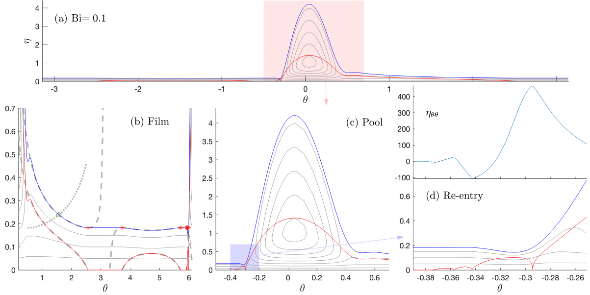
FIG. 6. Anatomy of the solution with (\Lambda, f, \text{Bi}, n, S) = (10, 0.01, 0.1, 1, 10^{-4}) . Plotted are \eta (blue) and \mathcal{Y} (red), along with a selection of streamlines (light grey solid lines). In (b), the residual film is shown in more detail. The dashed grey lines show the root of the cubic q = \text{constant} with \Gamma = \sin \theta , to which the solution converges over the film; the grey dotted line shows a second root, which intersects the first at the green circle at \theta = \frac{1}{2}\pi . A magnification of the pool is shown in (c). Details of where the film re-enters the pool are plotted in (d), along with \eta_{\theta\theta} .
