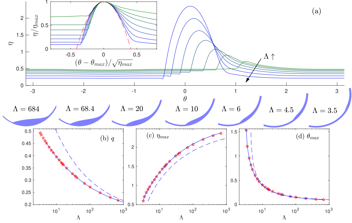
FIG. 4. Steady solutions with increasing \Lambda (from green to blue) for (f, \text{Bi}, n, S) = (0.0838, 0.158, 0.38, 10^{-4}) . In (a) the free surface profile is shown for the values of \Lambda indicated. The upper left inset shows a collapse of these profiles over the pool, along with the prediction in (38). In (b)-(d), the flux q , and the peak height and position, \eta_{max} and \theta_{max} , are plotted against \Lambda for a wider set of solutions (stars). The solid lines in (b) shows the predictions from (41), and the solid lines in (c,d) indicate the results from the S = 0 analysis of the Appendix. The dashed lines in (b,c,d) show the predictions from (42), (44) and (46).
