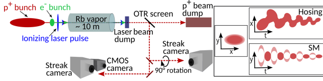
FIG. 1. Schematic of the experimental setup (not to scale) showing main components used for the measurements. Inset: sketch of the images recorded—time-integrated (x, y) , time-resolved (x, t) , (y, t) images when hosing and SM develop simultaneously.
