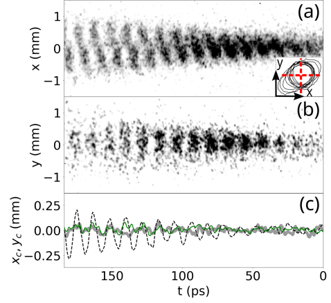
FIG. 2. Time-resolved images of the proton bunch ( n_{pe} = 0.96 \times 10^{14} \text{ cm}^{-3} , Q_p = (14.9 \pm 0.1) nC, \Delta x = (0.95 \pm 0.16) c/\omega_{pe} ). (a) x plane, hosing; (b) y plane, SM. Images—averages of ten consecutive single events recorded simultaneously, same color scale. Inset (a): single-event 3\sigma contours of time-integrated proton bunch charge distribution for the same ten events. Dashed red lines: position of the slit of the streak cameras. Elongation of the distribution indicates the plane of hosing. (c) Centroid position along the bunch in vacuum (gray line), undergoing SM (solid green line) and hosing (dashed black line).
