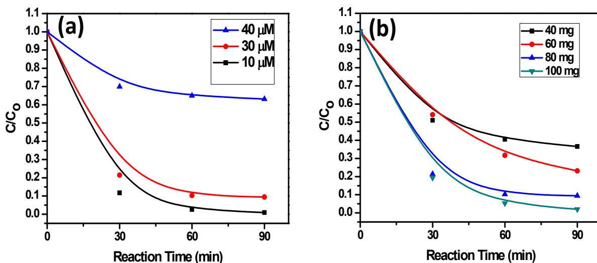
Fig. S1 (a) Effect of different initial concentration of MO under visible light irradiation and (b) different catalyst loading.
