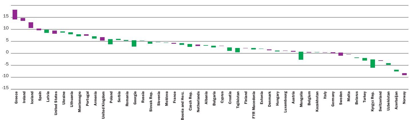
Chart 2.9b Consolidation needs, 2009 2
