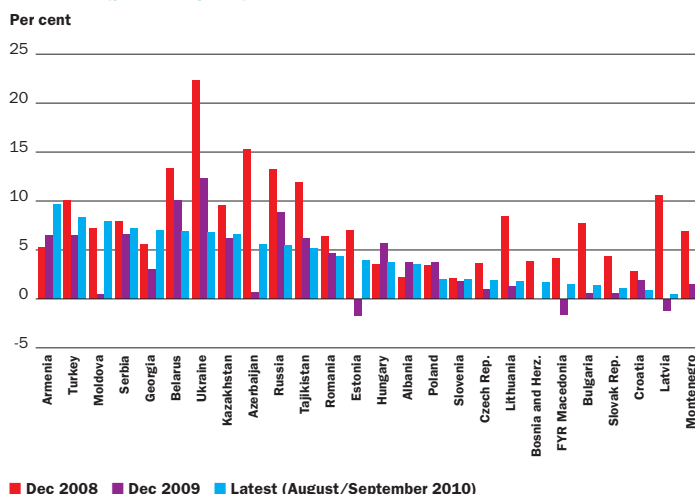
Chart 2.7a Inflation (year-on-year)
