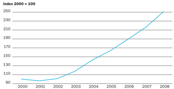
Chart 4.2a World exports
