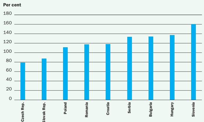
Chart 2.5.2 Loan-to-deposit ratios
