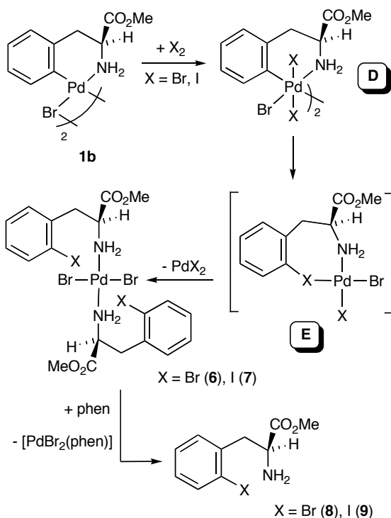
Scheme 4. Proposed reaction pathway for the synthesis of 2-halo derivatives of phenylalanine methyl ester 8 and 9 .
