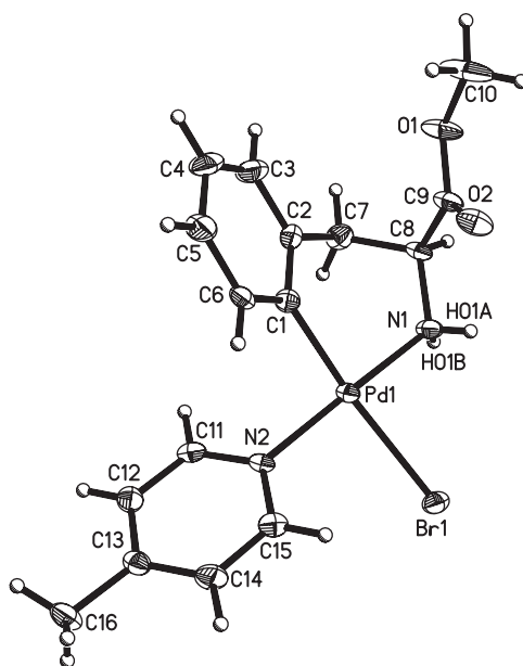
Figure 1. Thermal ellipsoid plot (50% probability) of 2 along with the labeling scheme. Selected bond lengths (Å) and angles (°): Pd(1)–Br(1) 2.5458(6), Pd(1)–N(1) 2.066(4), Pd(1)–C(1) 1.999(5), Pd(1)–N(2) 2.054(4), Br(1)–Pd(1)–N(1) 85.39(12), N(1)–Pd(1)–C(1) 92.19(18), C(1)–Pd(1)–N(2) 90.22(17), N(2)–Pd(1)–Br(1) 92.81(11).
