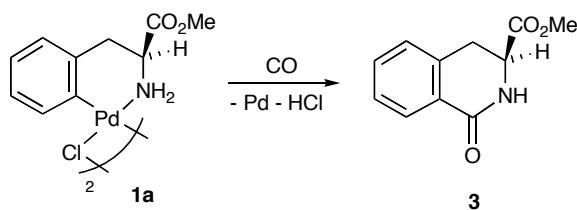
Scheme 2. Synthesis of ( S )-1-oxo-3-methoxycarbonyl-1,2,3,4-tetrahydroisoquinoline ( 3 ).
