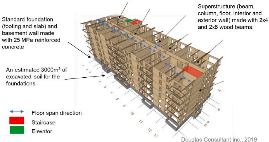
Fig. 3. PAL6 multi-residential building made of a light wood frame structure.
