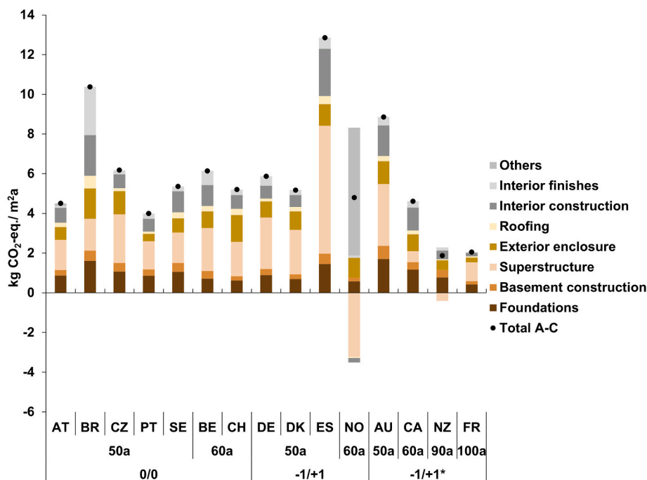
Fig. 5. Multi-residential building assessment of greenhouse gas emissions, grouped according to the biogenic carbon modeling approach and the service life (Modules A-C included, B6 excluded; Norway divided the life cycle stages A1-A3 into the elements, while the impacts of the other life cycle stages are summarized as “others”).
