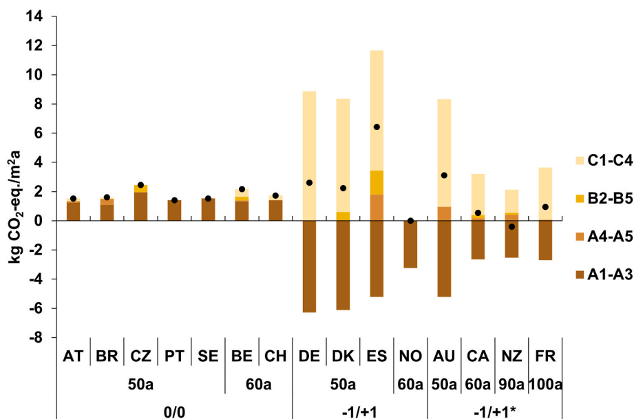
Fig. 4. Greenhouse gas emissions of the superstructure of the PAL 6 building assessed.
