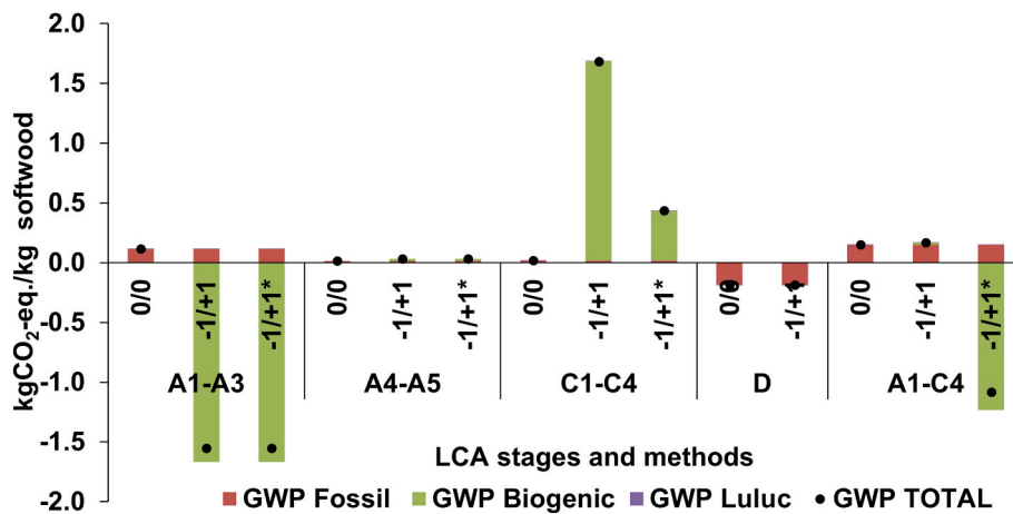
Fig. 2. Life cycle GWP of 1 m 3 planed, dried (MC = 10%) softwood beam (density (wet) = 465 kg/m 3 , carbon content 0.494 kg/kg dry wood) according to the life cycle stages using the 0/0, -1/+1 and the -1/+1* methodologies.
