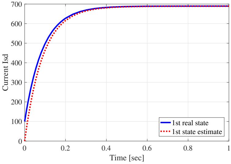
Fig. 4. x_1 and its estimation \hat{x}_1 .
