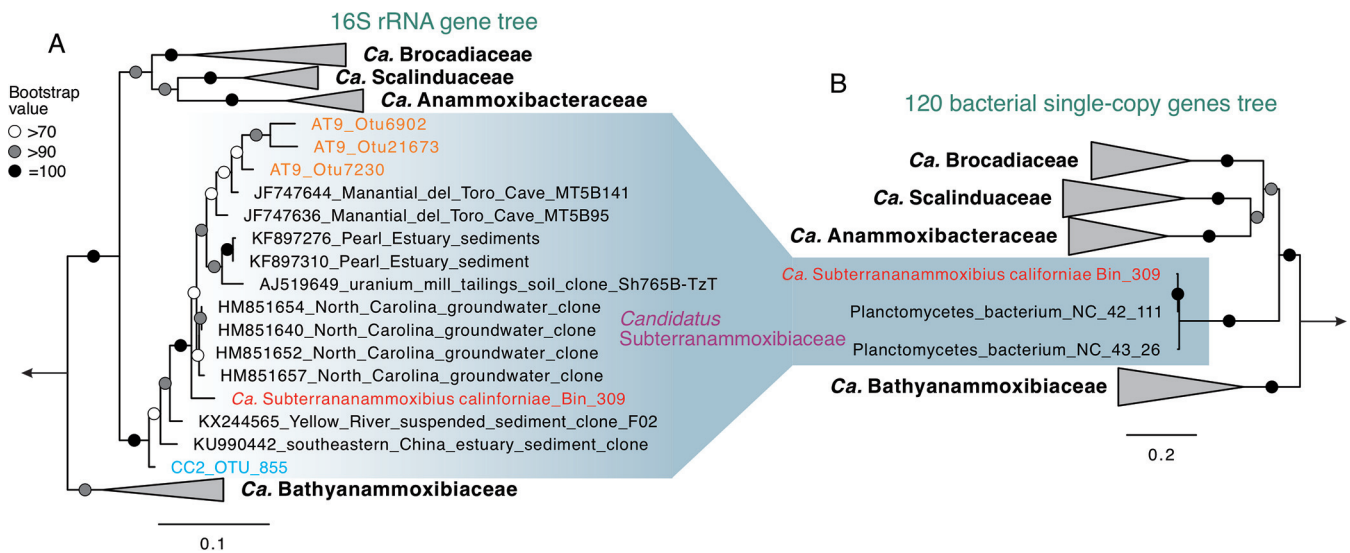
FIG 1 Phylogenetic relationship between “ Candidatus Subterraneanammonoxibiaceae ” and other known anammox bacteria. (A) Maximum-likelihood phylogenetic trees of bacteria in the Brocadiales order based on the 16S rRNA gene. The tree was inferred using IQ-TREE with GTR+F+R5 as the best-fit evolutionary model and 1,000 iterations of ultrafast bootstrap analysis. The three OTUs from Atacama Trench sediments are shown in orange, while the OTU from the Arctic core GS13-CC2 is highlighted in blue. (B) Maximum-likelihood phylogenetic trees of bacteria in the Brocadiales order based on 120 concatenated bacterial single-copy genes. The tree was inferred using IQ-TREE with LG+F+R8 as the best-fit evolutionary model, and 1,000 iterations of ultrafast bootstrap, to assess the robustness of both trees. For both trees, the phylogenetic analyses were done for all major lineages of the Planctomycetota phylum, but only branches within the Brocadiales order are shown here. The metagenome-assembled genomes (MAGs) recovered in this study from California groundwater samples are highlighted in red. Bootstrap values of >70 are shown with symbols listed in the legend. The scale bars show estimated sequence substitutions per residue.
