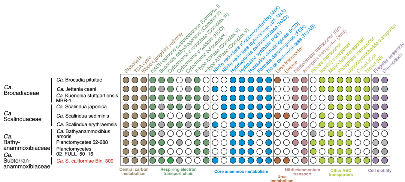
FIG 2 Metabolic potential of anammox bacteria. The family-level affiliations of the representative anammox genomes are shown on the left side. The high-quality MAG of “ Ca. Subterraneanammosibiaceae ” (“ Ca. S. californiae Bin_309”) recovered in this study is highlighted. Annotations of the other anammox genomes are from reference 26. The filled circles indicate the presence of the full metabolic pathway, open ones indicate the absence, and the gray ones indicate the partial presence of the pathway.
