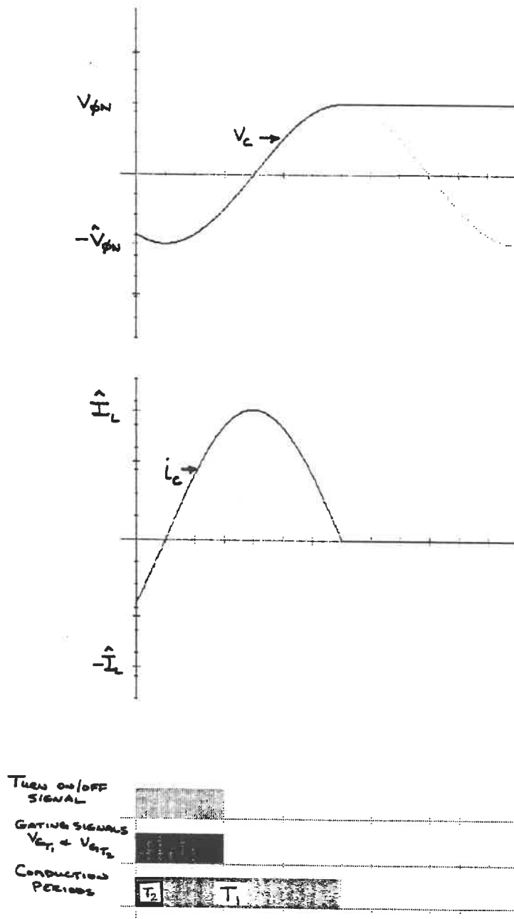
Fig. 2.3 Switching out the Single Phase AC Controller
