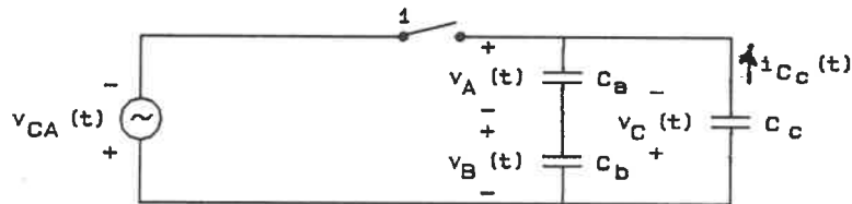
Fig. 5.2 Equivalent circuit of case a where switch 1 is closed
