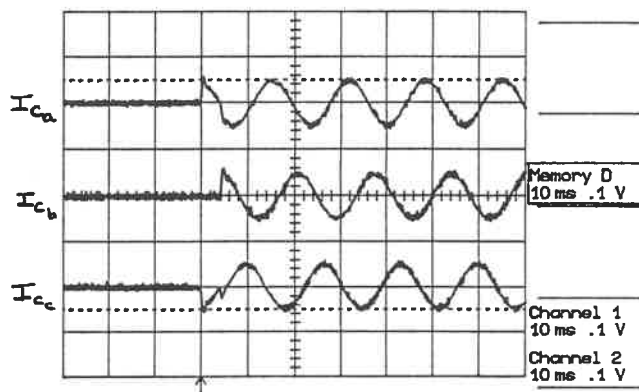
Plot 7.4 Phase currents when switching in a Three-Wire Branch-Controller with a Wye-Connected Load V_{\phi N} = 120V , I_{C_a} = 21.5A
