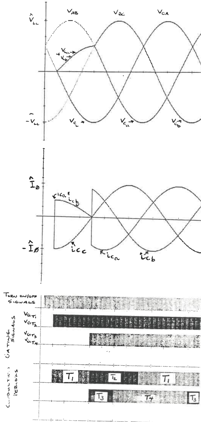
Fig. 5.4 Switching in a Three-Wire Assymetrical Line-Controller with a Delta-Connected Load; the capacitors are discharged
