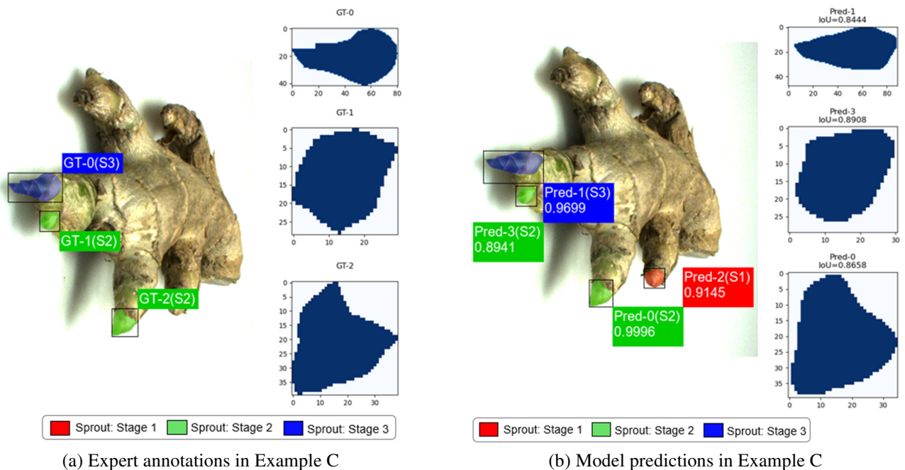
Fig. 15 Annotated Example C in the testing dataset and corresponding predictions using the hybrid model
