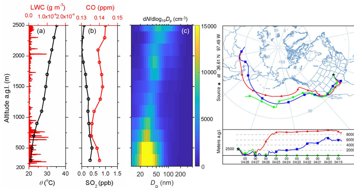
Figure 15. A long-range transport event observed during the research flight on 28 April 2016. (a) Vertical profiles of \theta and LWC. (b) Mixing ratios of CO and SO 2 . (c) Vertical profile of aerosol size distributions as a function of altitude. (d) Ten-day back-trajectories reaching an altitude of 2400 to 2600 m above the SGP on 28 April 2016. The particle concentrations, surface area concentrations, and size distributions are normalized to STP (273.15 K and 101.325 kPa). Note that the SO 2 mixing ratio is corrected by a constant offset so that the minimum mixing ratio value is set to 0.
