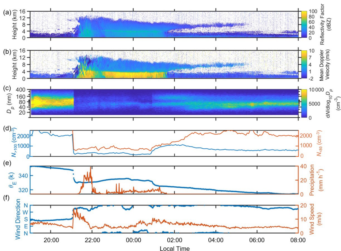
Figure 13. Ground measurements of aerosol, cloud, and meteorological properties during the convective downward transport event from 9 to 10 September 2016. (a) Cloud reflectivity measured by the RWP. (b) Mean Doppler velocities measured by the RWP. A positive value indicates downward motion. (c) Aerosol size distributions measured by a scanning mobility particle sizer (SMPS). (d) Concentration of aerosols with sizes above 100 nm ( N_{>100} ) and below 80 nm ( N_{<80} ). (e) Equivalent potential temperature and precipitation rate measured by the weather station. (f) Wind direction and wind speed measured by the weather station.
