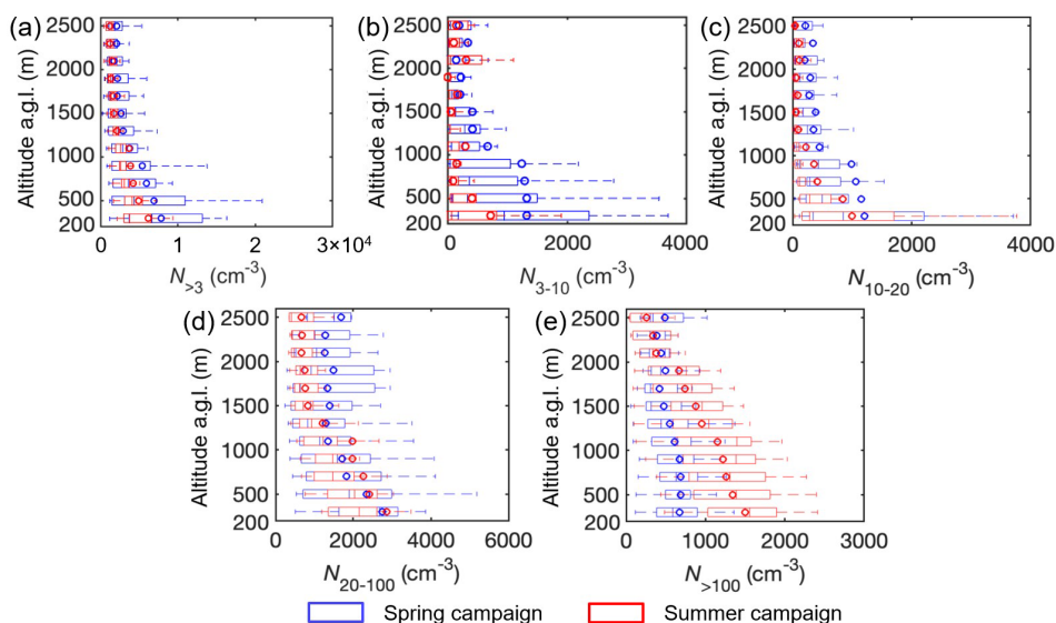
Figure 5. Vertical profiles showing the concentrations of particles (a) larger than 3 nm ( N_{>3} ), (b) with sizes between 3 and 10 nm ( N_{3-10} ), (c) with sizes between 10 and 20 nm ( N_{10-20} ), (d) with sizes between 20 and 100 nm ( N_{20-100} ), and (e) with sizes above 100 nm ( N_{>100} ) over the SGP site during the spring campaign (blue) and summer campaign (red). The line and circle markers represent the median and mean of the data, and the edges of the box indicate the 25th and 75th percentiles, respectively. The concentrations are normalized to STP (273.15 K and 101.325 kPa).
