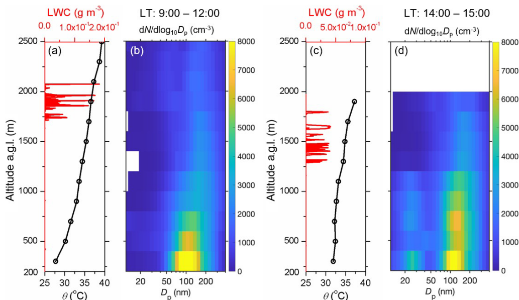
Figure 11. Vertical profiles of parameters over the SGP site on 4 September 2016. Panels (a) and (b) correspond to a local time of 09:00 to 12:00, and panels (c) and (d) correspond to a local time of 14:00 to 15:00. Panels (a) and (c) show \theta and LWC. (b, d) Vertical profile of aerosol size distributions as a function of altitude. The size distributions are normalized to STP (273.15 K and 101.325 kPa).
