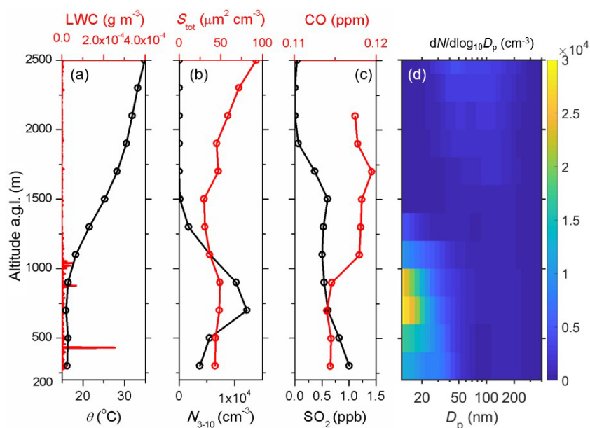
Figure 8. Vertical profiles of parameters during an NPF event occurring at the upper boundary layer over the SGP site on 14 May 2016. (a) \theta and LWC. (b) Concentration of particles between 3 and 10 nm ( N_{3-10} ) and total aerosol surface area concentration. (c) Mixing ratios of carbon monoxide (CO) and sulfur dioxide ( \text{SO}_2 ). (d) Vertical profile of aerosol size distributions as a function of altitude. The particle concentrations, surface area concentrations, and size distributions are normalized to STP (273.15 K and 101.325 kPa). Note that the \text{SO}_2 mixing ratio is corrected by a constant offset so that the minimum mixing ratio value is set to 0.
