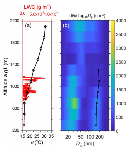
Figure 10. Vertical profiles of parameters during a cloud processing event over the SGP site on 1 May 2016. (a) \theta and LWC. (b) Vertical profile of aerosol size distributions as a function of altitude. The black line shows the mode diameter of the accumulation-mode aerosols. The particle concentrations, surface area concentrations, and size distributions are normalized to STP (273.15 K and 101.325 kPa).
