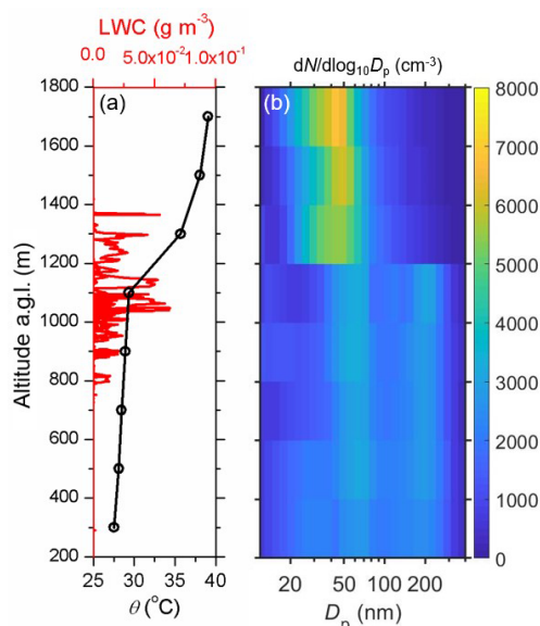
Figure 12. Vertical profiles of parameters during an entrainment event over the SGP site on 25 April 2016. (a) \theta and LWC. (b) Vertical profile of aerosol size distributions as a function of altitude. The particle concentrations, surface area concentrations, and size distributions are normalized to STP (273.15 K and 101.325 kPa).
