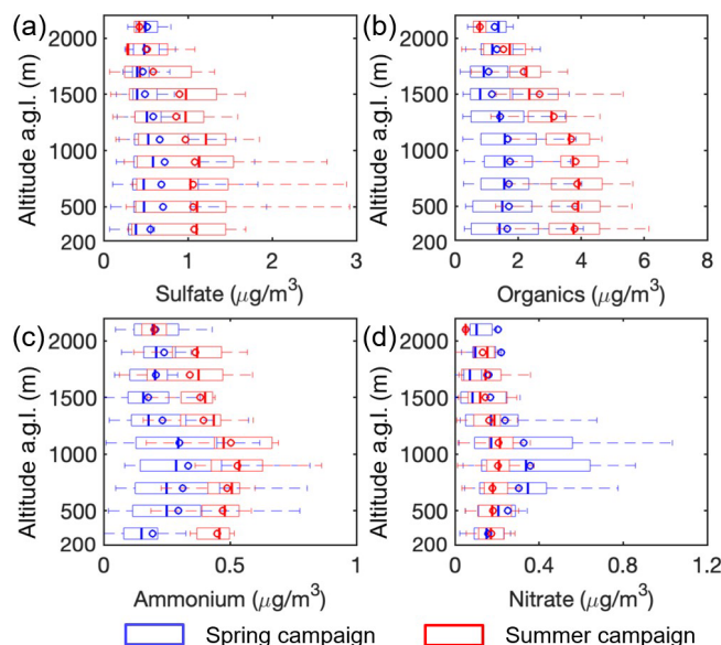
Figure 6. Vertical profiles of the mass concentrations of (a) sulfate, (b) organics, (c) ammonium, and (d) nitrate over the SGP during the spring campaign (blue) and summer campaign (red). The compositions are measured by the HR-ToF-AMS. The concentration of chloride is too low and therefore is not shown in the figure. The line and circle markers represent the median and mean of the data, and the edges of the box indicate the 25th and 75th percentiles, respectively. The concentrations are normalized to STP (273.15 K and 101.325 kPa).
