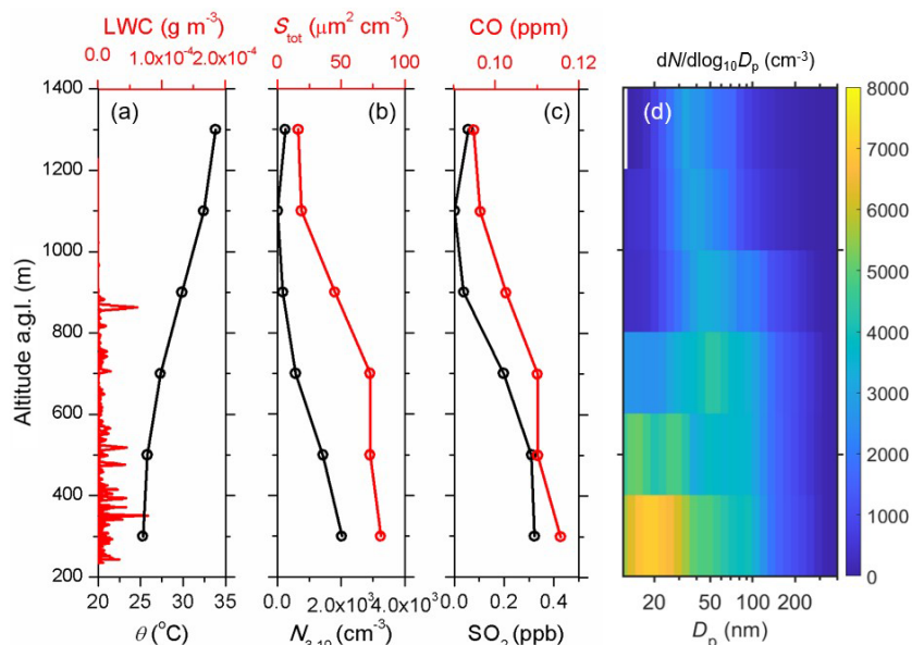
Figure 7. Vertical profiles of parameters during a NPF event occurring at the surface of the SGP site on 11 September 2016. (a) Potential temperature ( \theta ) and liquid water content (LWC). (b) Concentration of particles between 3 and 10 nm ( N_{3-10} ) and total aerosol surface area concentration. (c) Mixing ratios of carbon monoxide (CO) and sulfur dioxide ( \text{SO}_2 ). (d) Vertical profile of aerosol size distributions as a function of altitude. The particle concentrations, surface area concentrations, and size distributions are normalized to STP (273.15 K and 101.325 kPa). Note that the \text{SO}_2 mixing ratio is corrected by a constant offset so that the minimum mixing ratio value is set to 0.
