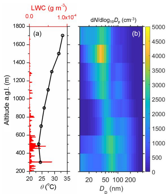
Figure 14. Vertical profiles of parameters during a convective downward transport event over the SGP site on 10 September 2016. (a) \theta and LWC. (b) Vertical profile of aerosol size distributions as a function of altitude. The particle concentrations, surface area concentrations, and size distributions are normalized to STP (273.15 K and 101.325 kPa).
