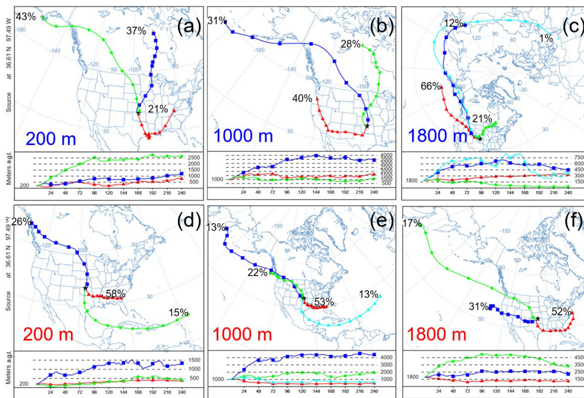
Figure 3. Cluster analysis of 10 d back-trajectories arriving at 200, 1000, and 1800 m above the SGP site during the spring (first row) and summer (second row) campaigns. The average trajectories of the clusters are represented by different colors, and the associated numbers denote the occurrence percentages of the clusters.
