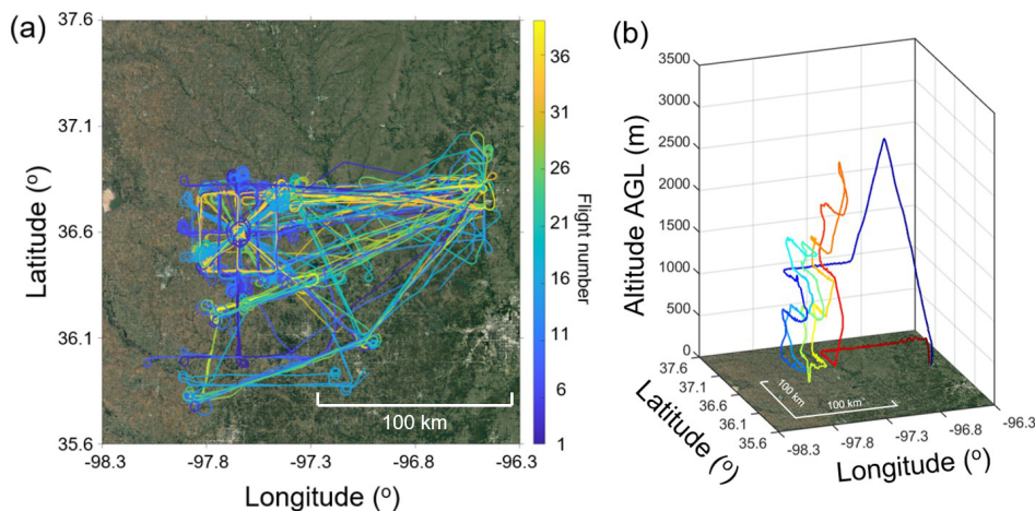
Figure 2. (a) Flight patterns used during the HI-SCALE campaign. A total number of 38 flights were conducted over the SGP observatory. Different colors of the flight patterns represent different flight numbers. (b) An example of the flight pattern on 3 May 2016. The color represents the local time in hours. The maps are obtained from © Google Maps.
