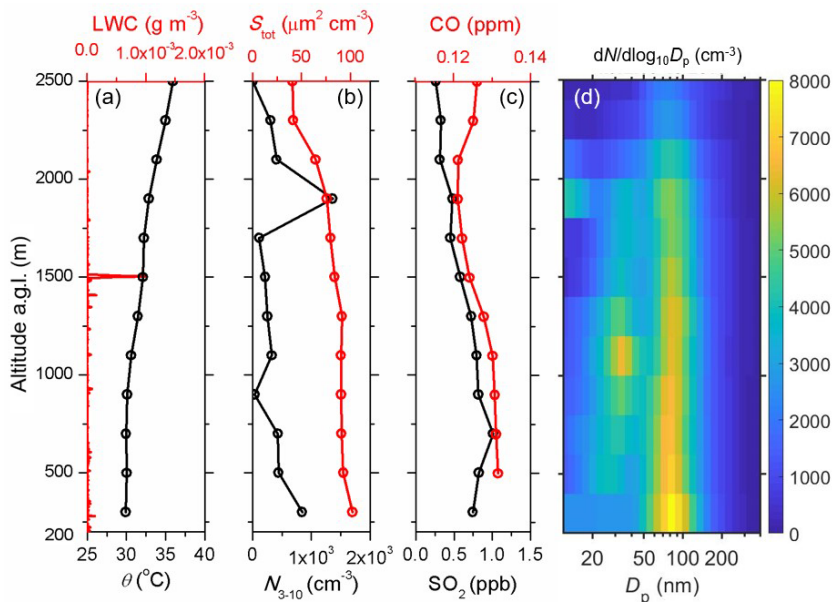
Figure 9. Vertical profiles of parameters during an NPF event occurring in the free troposphere over the SGP site on 13 May 2016. (a) \theta and LWC. (b) Concentration of particles between 3 and 10 nm ( N_{3-10} ) and total aerosol surface area concentration. (c) Mixing ratios of CO and \text{SO}_2 . (d) Vertical profile of aerosol size distributions as a function of altitude. The particle concentrations, surface area concentrations, and size distributions are normalized to STP (273.15 K and 101.325 kPa). Note that the \text{SO}_2 mixing ratio is corrected by a constant offset so that the minimum mixing ratio value is set to 0.
