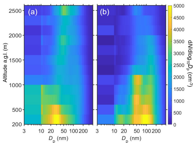
Figure 4. Vertical profiles of the mean aerosol size distributions during the (a) spring campaign and (b) summer campaign. Note that the size distributions between 3 and 10 nm are calculated based on the difference in concentrations monitored by the two CPCs, and the size distributions above 10 nm are obtained by the FIMS. The size distributions are normalized to standard temperature and pressure (273.15 K and 101.325 kPa; STP).
