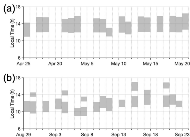
Figure 1. Date and local time of the flights conducted during the HI-SCALE campaign: (a) spring campaign and (b) summer campaign. During the summer campaign, same-day flights were conducted to examine the temporal variation of aerosols over the SGP.
