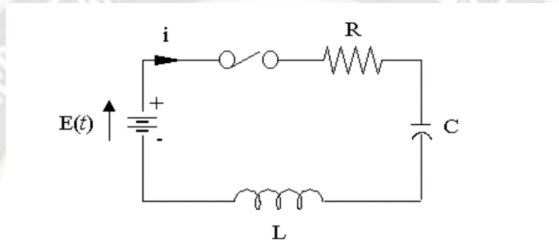
Figure 4.1: Electric Circuits.
