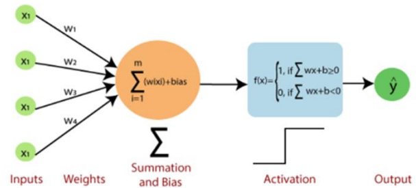
Figure 1: Single Layer Perceptron
