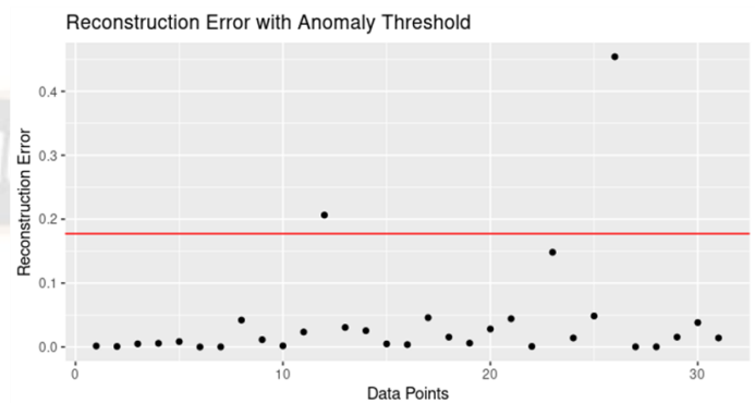
Figure 6: Reconstruction Error with Anomaly Threshold
