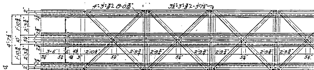
PLAN ON A-A
