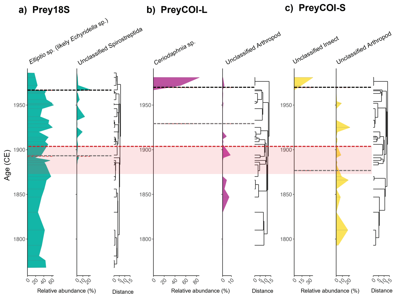
Figure 4. Stigraphic plot of taxonomic groups commonly eaten by Salmo trutta in Aotearoa-New Zealand (Arthropoda, Mollusca and Rotifera). Sequences were retrieved from: (a) 18S rRNA (Prey18S), (b) long COI (PreyCOI-L), and (c) short COI (PreyCOI-S) primers over ~200 yrs in Lake Paringa sediment. CONISS derived dendrograms and assemblage change points (black dashed lines = primary, grey dashed lines = secondary) are shown alongside selected taxa. The red dashed line indicates when S. trutta DNA appeared in the core (1906 [1892–1919 CE]) while the pale red box indicates the period S. trutta are expected to have been introduced (1870–1906 [1892–1919 CE]).
