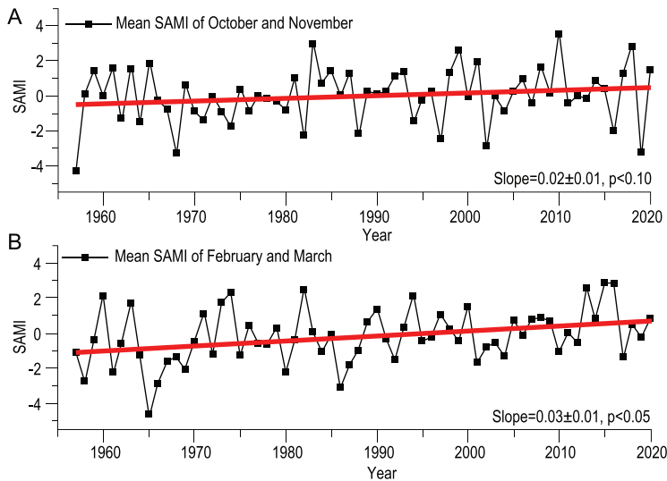
Figure 3. Interannual variation of SAM index (SAMi) (1957.1–2020.12 obtained from https://legacy.bas.ac.uk/met/gjma/sam.html ). (A) Melt onset (October and November) and (B) end date (February and March) with trend lines fitted for 1957–2020 (red line). The estimated slopes and its 95% confidence intervals are shown.
