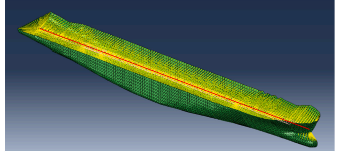
Fig. 4. FEM model of a 6750-TEU containership.
