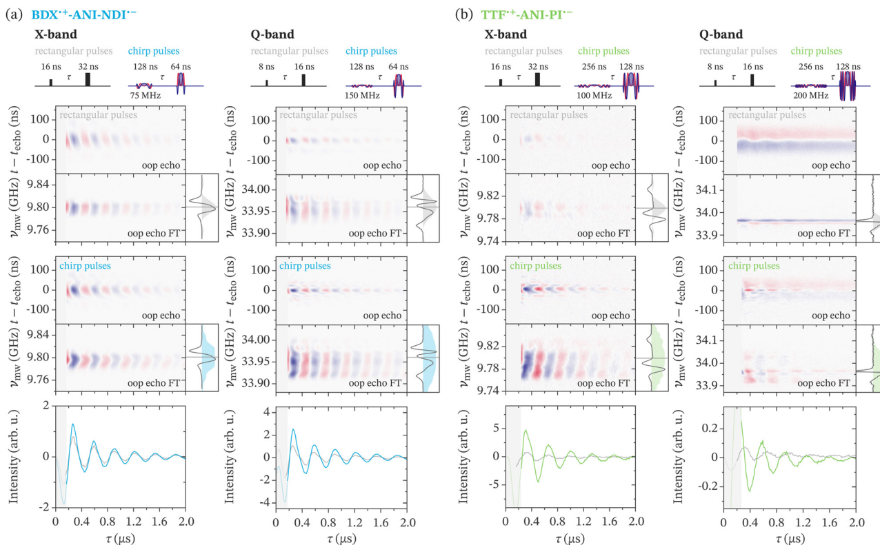
Fig. 7 Comparison of out-of-phase ESEEM experiments with monochromatic rectangular pulses and frequency-swept pulses for \text{BDX}^{\bullet+}-\text{ANI}-\text{NDI}^{\bullet-} and \text{TTF}^{\bullet+}-\text{ANI}-\text{PI}^{\bullet-} at X- and Q-band. The out-of-phase echo recorded as a function of the interpulse delay \tau and the corresponding echo Fourier transforms are shown for both types of pulse sequences and the out-of-phase ESEEM traces resulting from integration in the frequency-domain are compared at the bottom. The calculated pulse excitation profiles are compared to the tREPR spectra of the two integrations. The experiments were performed at magnetic fields of 349.3 mT ( \text{BDX}-\text{ANI}-\text{NDI} ) and 348.7 mT ( \text{TTF}-\text{ANI}-\text{PI} ) at X-band (9.8 GHz), and 1210.5 mT ( \text{BDX}-\text{ANI}-\text{NDI} ) and 1210.4 mT ( \text{TTF}-\text{ANI}-\text{PI} ) at Q-band (33.96 GHz). At X-band, rectangular pulses of 16 ns and 32 ns length and chirp pulses with a bandwidth of 75 MHz and lengths of 128 ns and 64 ns and with a bandwidth of 100 MHz and lengths of 256 ns and 128 ns were used for \text{BDX}^{\bullet+}-\text{ANI}-\text{NDI}^{\bullet-} and \text{TTF}^{\bullet+}-\text{ANI}-\text{PI}^{\bullet-} , respectively. At Q-band, rectangular pulses of 8 ns and 16 ns length and chirp pulses with a bandwidth of 150 MHz and lengths of 128 ns and 64 ns and with a bandwidth of 200 MHz and lengths of 256 ns and 128 ns were used for \text{BDX}^{\bullet+}-\text{ANI}-\text{NDI}^{\bullet-} and \text{TTF}^{\bullet+}-\text{ANI}-\text{PI}^{\bullet-} , respectively. The grey-shaded area corresponds to the initial deadtime and the out-of-phase ESEEM traces in this region were reconstructed as described in Section 2.2.
