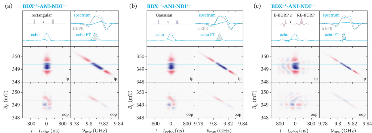
Fig. 4 X-band echo-detected field sweep experiments with narrowband selective pulses on \text{BDX}^{*+}\text{-ANI-NDI}^{*-} . The echo transients were recorded as a function of magnetic field with two-pulse sequences consisting of rectangular 100 ns and 200 ns pulses (a), Gaussian 200 ns ( t_{\text{FWHM}} = 75 ns) and 400 ns ( t_{\text{FWHM}} = 150 ns) pulses (b), and a sequence consisting of an 800 ns E-BURP 2 and a 1600 ns RE-BURP pulse (c). The in- and out-of-phase echo transients and the corresponding Fourier transforms are shown as a function of magnetic field in the 2D plot (blue = positive signal/absorption, red = negative signal/emission). The in-phase (dashed line) and out-of-phase (solid line) contributions to the echo and echo FT extracted at the field position marked by the horizontal line (349.4 mT) are also shown and compared to the calculated excitation profile of the \pi pulse. The spectrum constructed from the sum of the echo FTs at the different magnetic field positions is compared to the trEPR spectrum. The corresponding results obtained for TTF-ANI-PI are shown in Fig. S5 in the ESI.†
