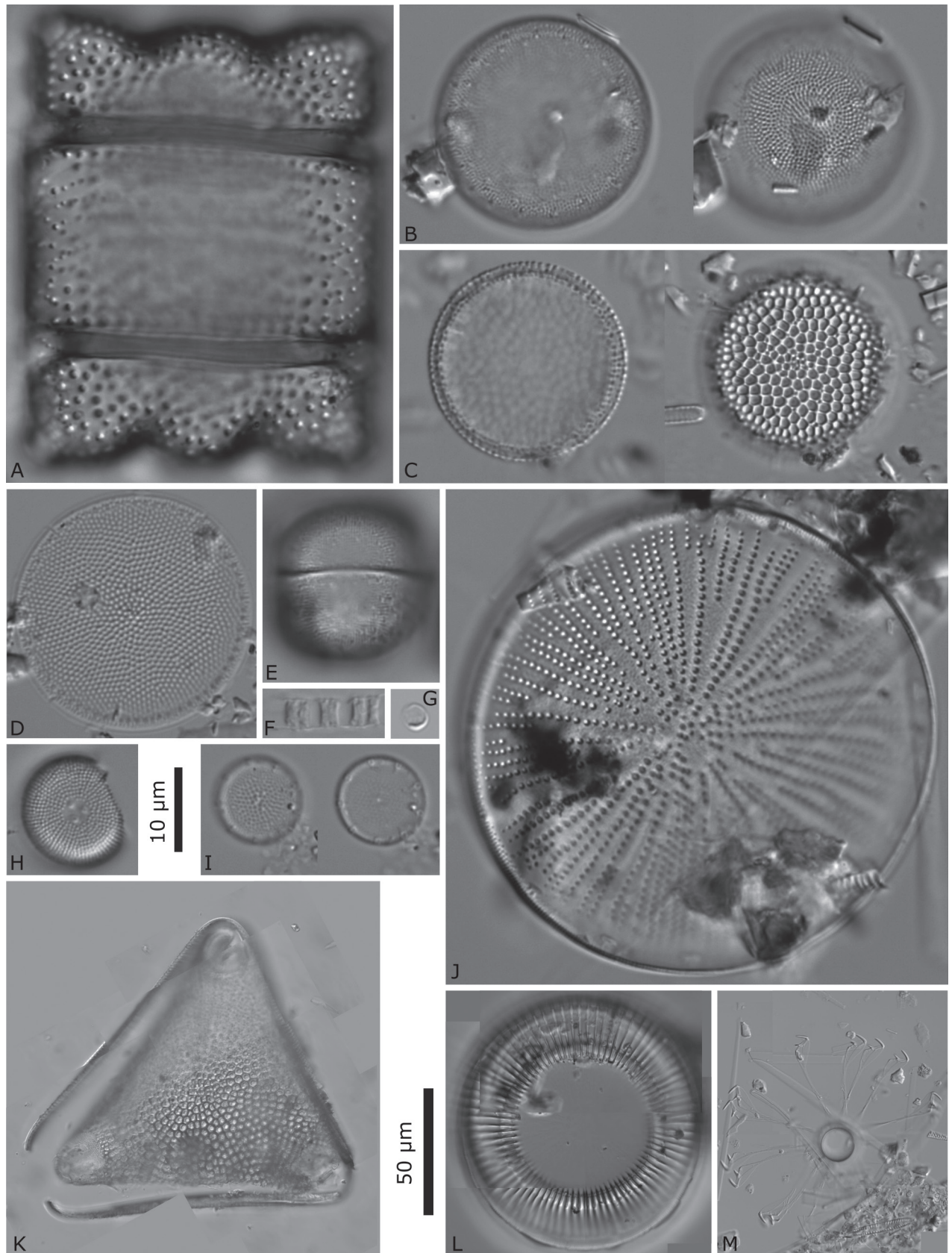
Figure 2. LM pictures of taxa found by morphological analyses. A Odontella litigiosa . B Porosira cf. glacialis . C Thalassiosira scotia . D Thalassiosira antarctica . E Melosira sp. F Unidentified centric diatom. G Minidiscus chilensis . H Orthoseira roeseana . I Shionodiscus gracilis var. expectus . J Actinocyclus actinochilus . K Trigonium arcticum . L Ellerbeckia sol . M Corethron pennatum . Scale bars: 10 µm (A–J); 50 µm (K–M).
