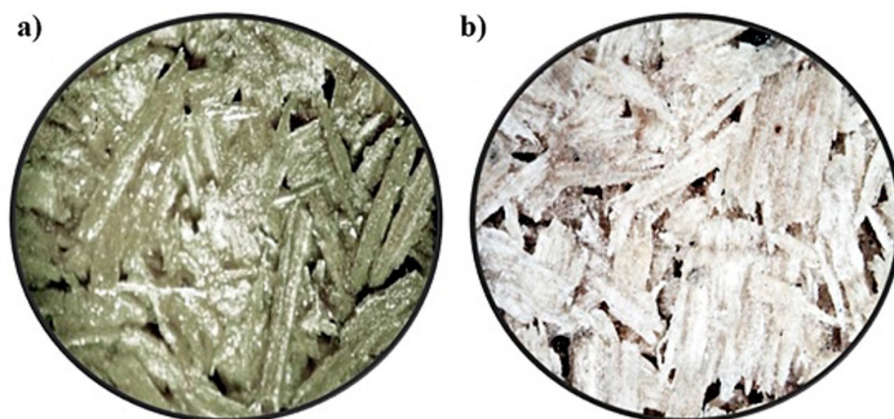
Fig. 3. Stereoscopic Image (40X) of particle composites a) Musa acuminata , b) commercial composites. Source: Authors.
