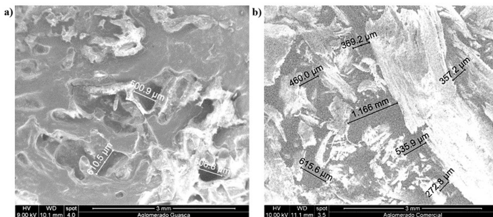
Fig. 4. SEM Image, a) Musa acuminata agglomerate and b) commercial agglomerate. Source: Authors.
