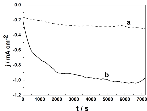
Fig. 9. Chronoamperometric responses recorded at \text{Fe}_2\text{P} upon application of the constant potential of -0.4 V (a) in the absence of nitrogen (i.e. in argon-saturated solution), and (b) in the nitrogen-saturated solution.
