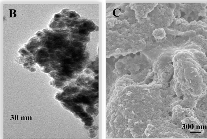
Fig. 2. (A) XRD pattern of the synthesized \text{Fe}_2\text{P} catalyst recorded upon its activation at 450^\circ\text{C} . (B) Transmission electron microscopic and (C) scanning electron microscopic images of \text{Fe}_2\text{P} .
