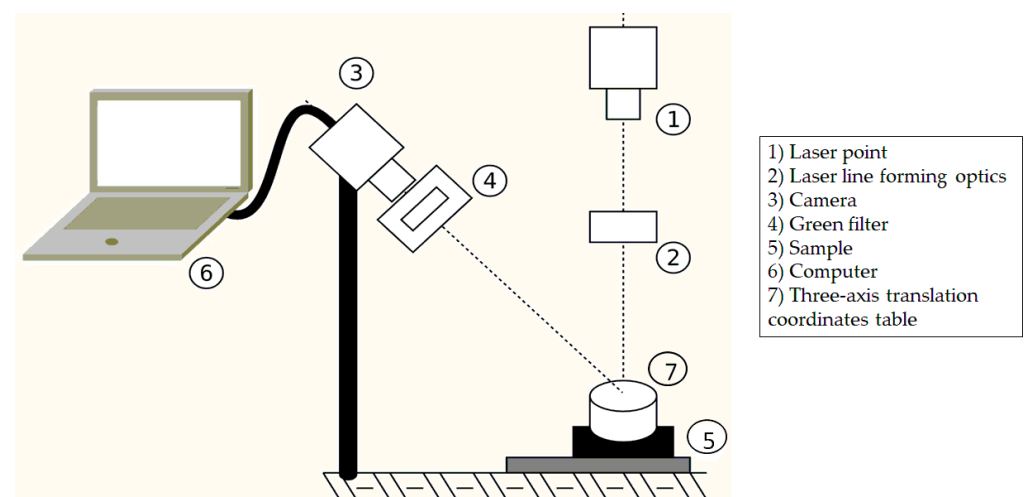
Figure 3. Optical sensor setup with the sample arranged on the three-axis translation coordinates table, composed by: (1) Laser point, (2) Laser line forming optics, (3) Camera, (4) Green filter, (5) Soil sample, (6) Computer, (7) Three-axis translation coordinates table.
