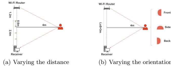
Fig. 11. Experiment setup of different transceiver distances and target orientations
