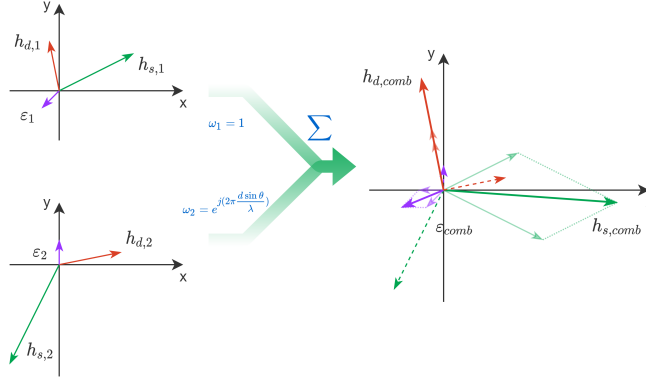
Fig. 2. A simple example of Delay and Sum Beamforming.
