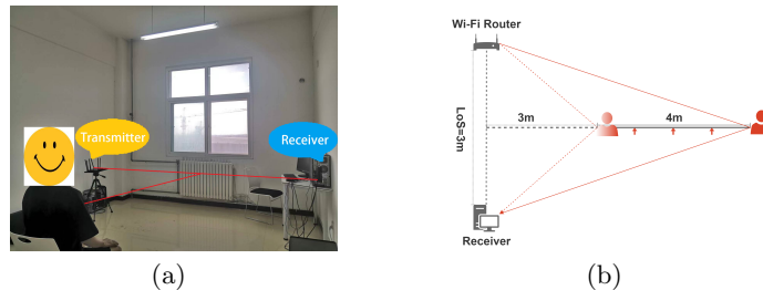
Fig. 9. Experimental scenario and experimental setup for comprehensive experiment.
