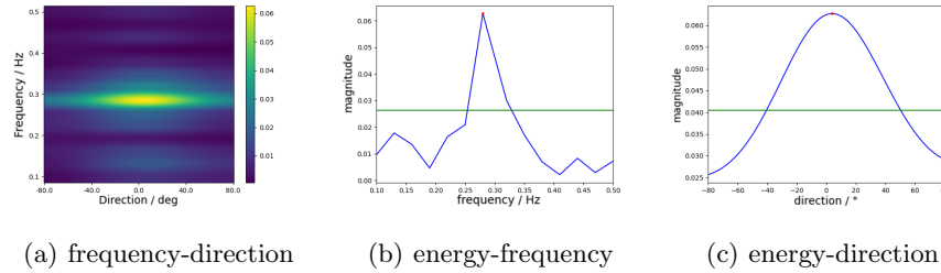
Fig. 8. An spectrum example of respiration sensing.
