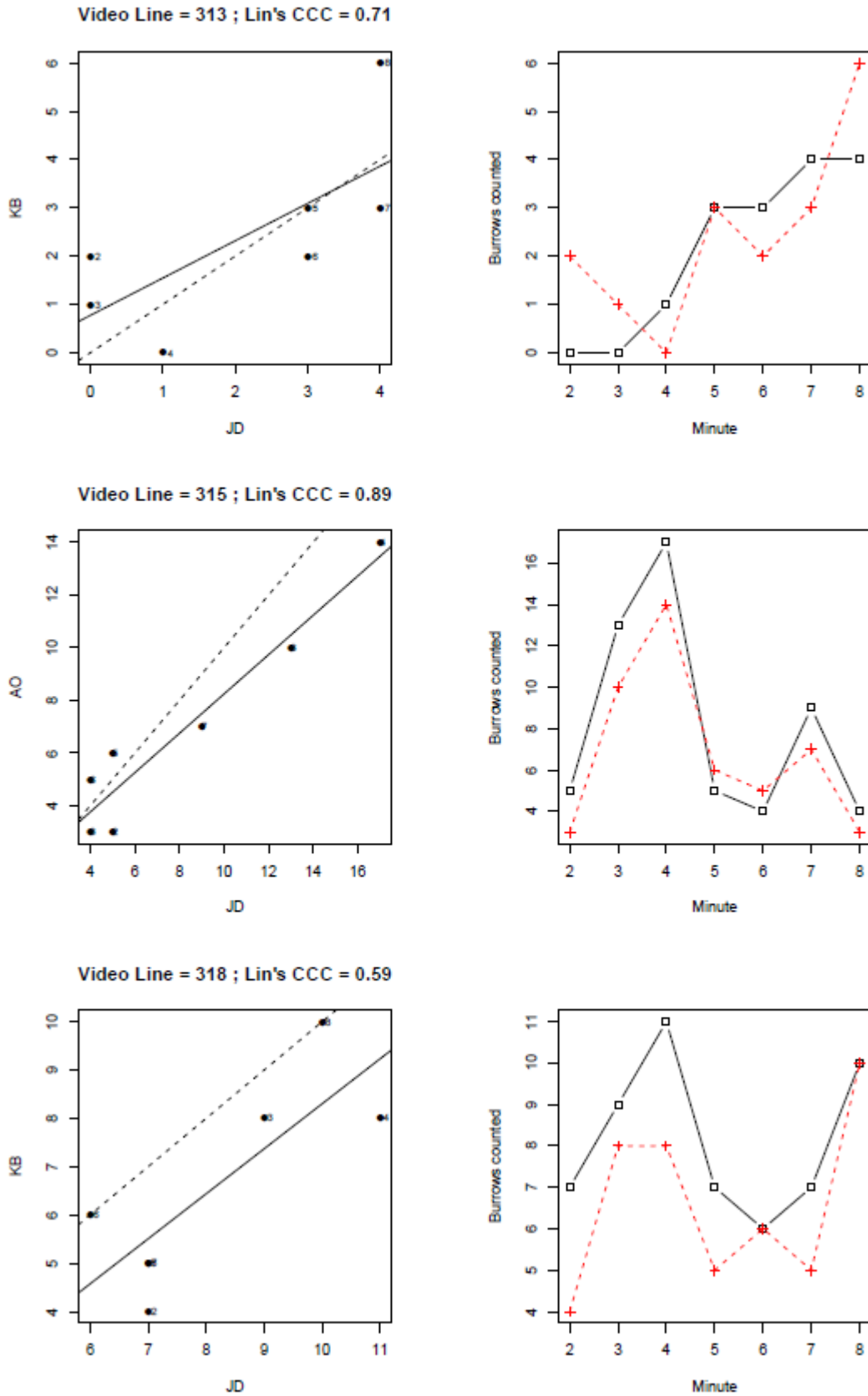
Figure 4: FU19 grounds: Lin's CCC quality control plot of count data for stations 313, 315 and 318 of the 2023 survey.
