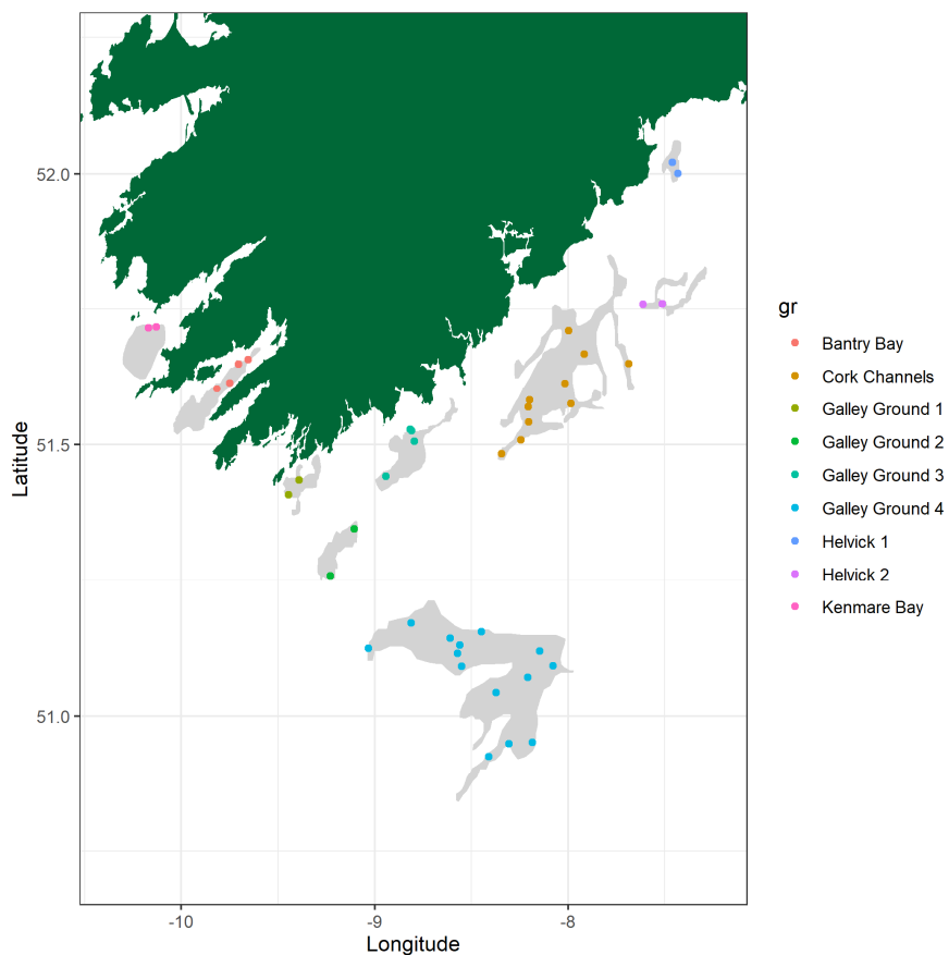
Figure 2: FU19 grounds: Stations planned and completed on the 2023 Nephrops UWTV survey by individual ground.
