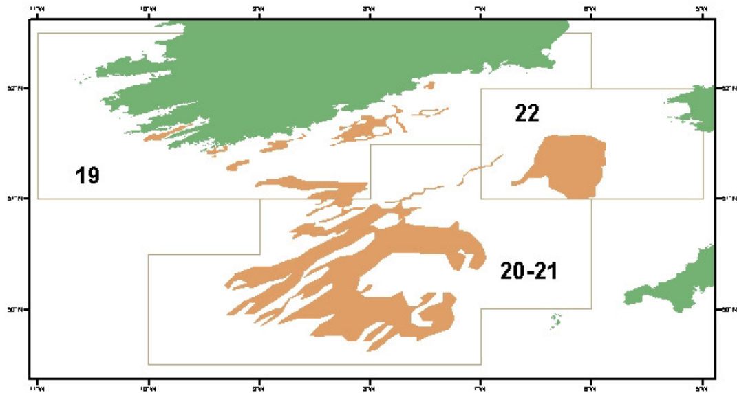
Figure 1: FU19 grounds: Nephrops Functional Units (FUs) and Nephrops grounds (area polygons) in the greater Celtic Sea.
