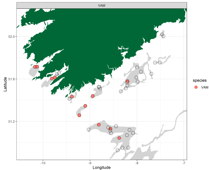
Figure 9: FU19 grounds: 2023 stations where Virgularia mirabilis (VAM) was identified and noted as present or absent. Closed circles indicated presence and open circles denote TV stations with no sea-pen observations.
