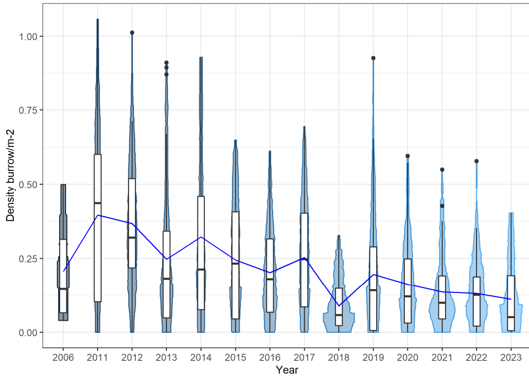
Figure 7: FU19 grounds: Combined violin and box plot of adjusted burrow density distributions by year for 2006-2023. The blue line indicates the mean density over time. The horizontal black lines represent medians, white boxes the inter quartile ranges, the black vertical lines the range and the black dots are outliers. No TV survey from 2007 – 2010.
