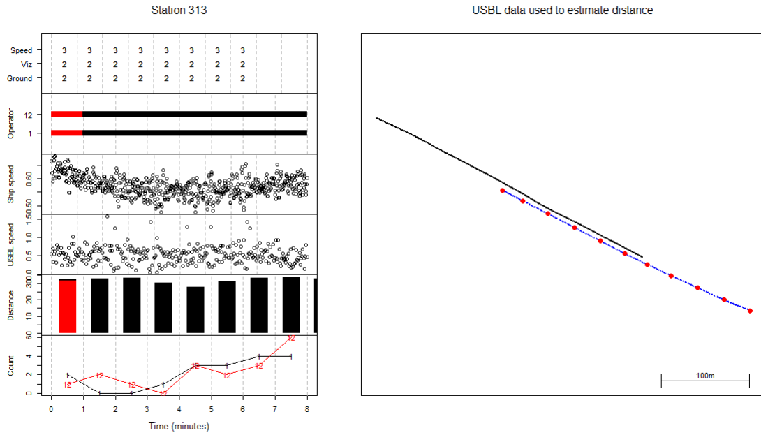
Figure 3: FU19 grounds: R - tool quality control plot for station 313 of the 2023 UWTV survey.
