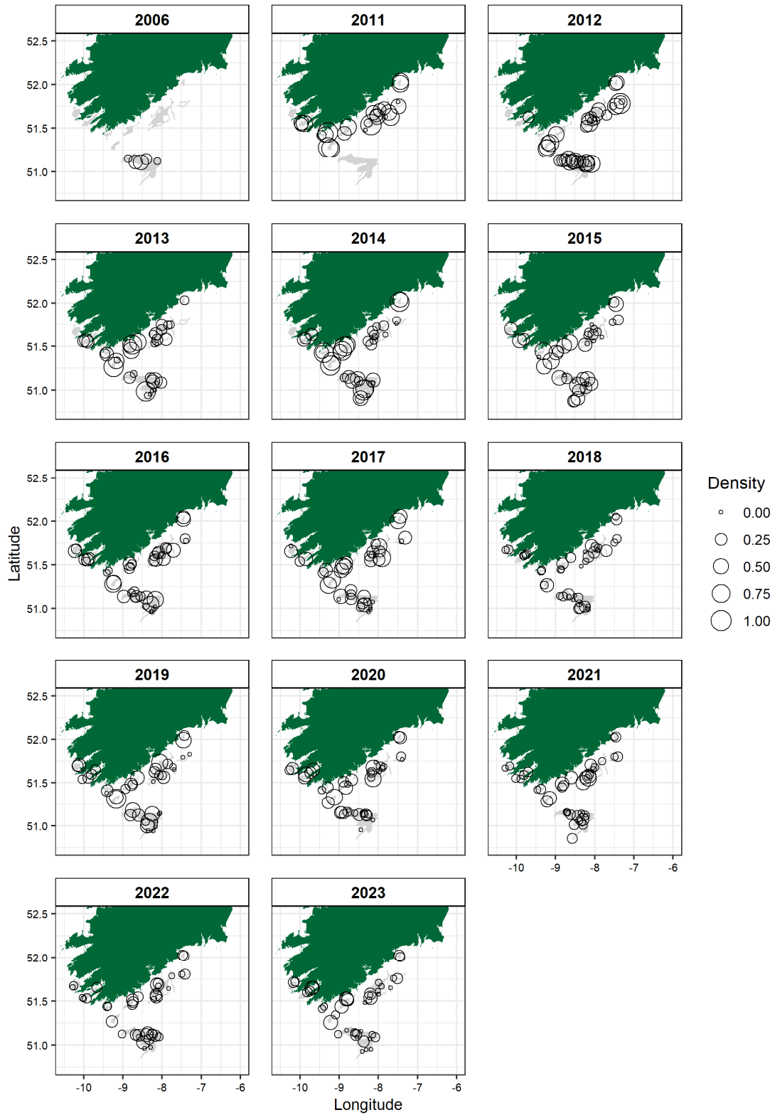
Figure 5: FU19 grounds: Bubble plot of the adjusted density (burrows/m 2 ) from 2006 to 2023.
