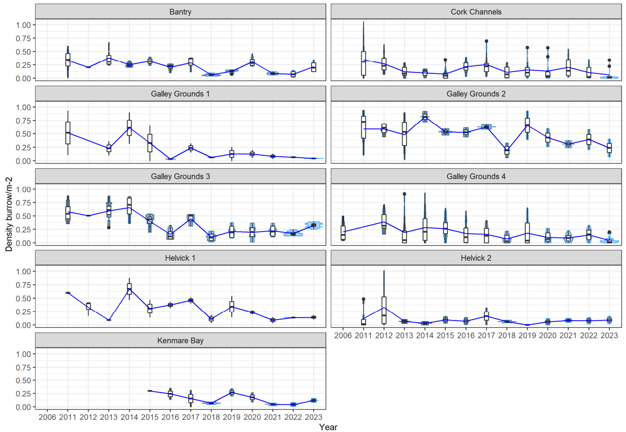
Figure 6: FU19 grounds: Violin and box plots of adjusted burrow density distributions by year for 2006-2023 for each ground. The blue line indicates the mean density over time. The horizontal black line represents the median, white box is the inter quartile range, the black vertical line is the range and the black dots are outliers. No TV survey from 2007 – 2010.
