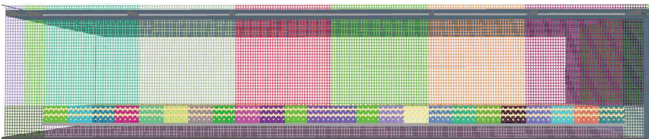
Figure 3. Grid cell resolution of the model: 15 mm × 15 mm × 17.5 mm per cell for the wood sticks at solid phase, 60 mm × 60 mm × 70 mm and 30 mm × 30 mm × 35 mm cell size at the gas phase, total number of cells ~8.3 million with 125 meshes.
