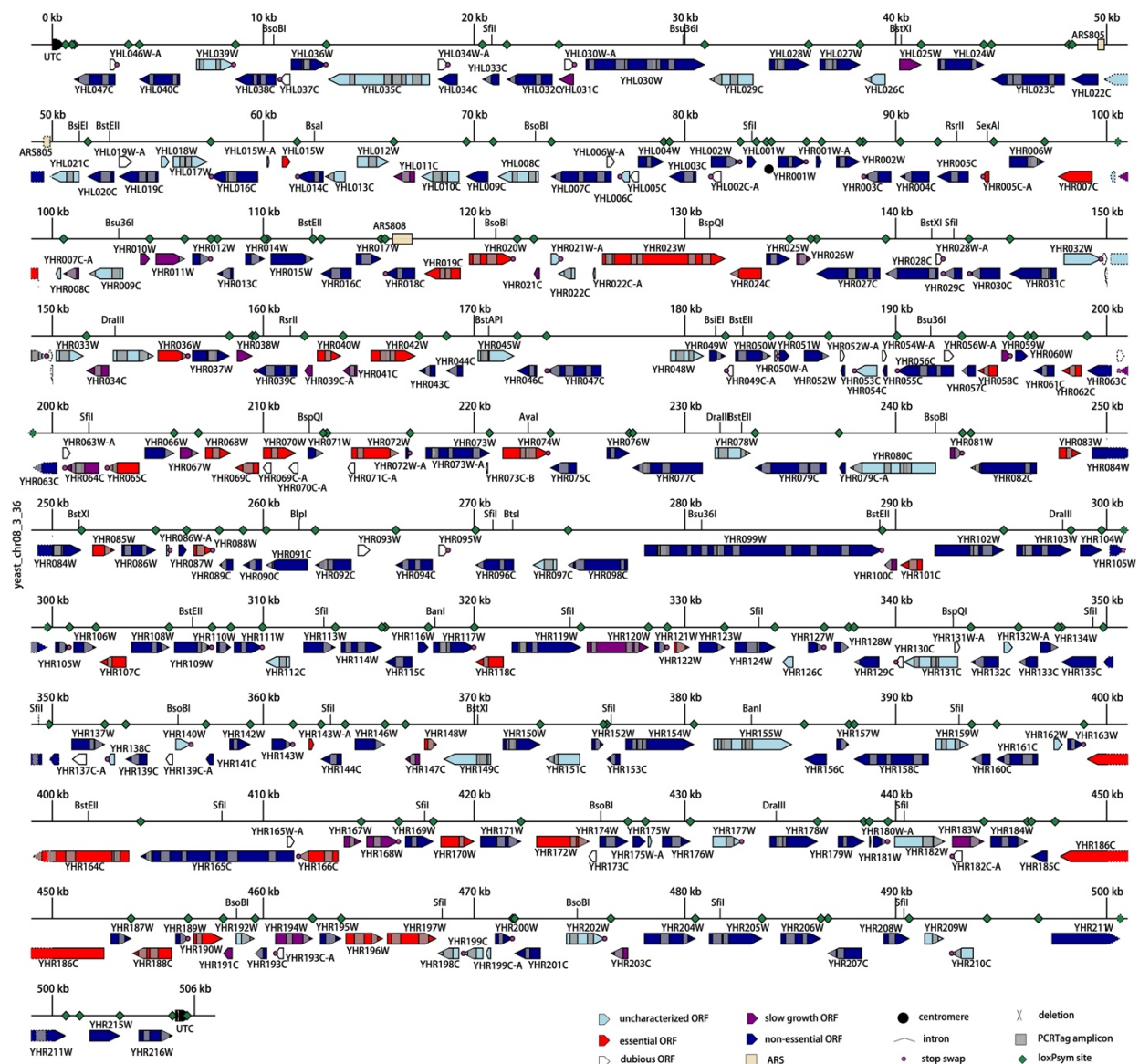
Fig. S1. Schematic illustration of the designed sequence for synthetic chromosome VIII ( synVIII ). Related to Figure 1. Each open reading frame (ORF) is depicted as designed, including the precise number of synonymously recoded PCRTags and loxPsyn sites that are present at the 3' end of every nonessential ORF. Also depicted are the locations of TAG stop codon swaps to TAA, the restriction enzyme sites used for ligation of synthetic chunks, and genomic features including centromeres and ARS.
