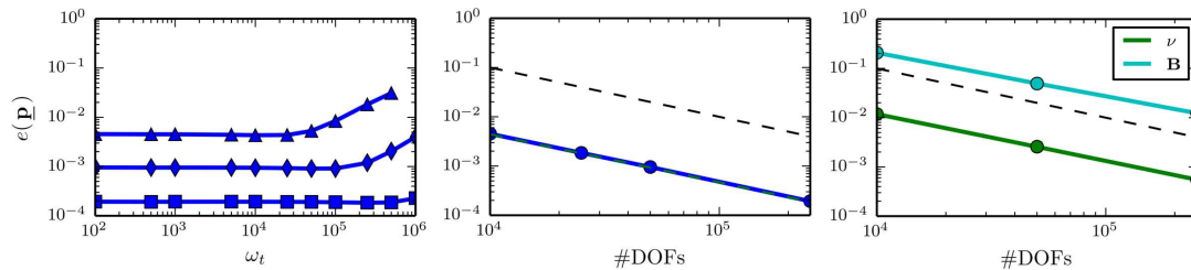
FIGURE 1. L^2 error (left) as function of \omega_t , with 10k (triangles), 50k (diamonds) and 250k (squares) DOFs. (middle) with numerically approximated surface quantities (solid) w.r.t. the number of DOFs for fixed \omega_t = 1000 . Dashed line indicates linear rate of convergence. (right) for numerical approximation of surface quantities w.r.t. the number of DOFs for fixed \omega_t = 1000 .
