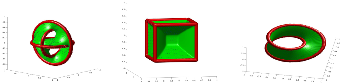
FIGURE 2. Numerical approximation of solutions to the Plateau problem based on the approach of [3].
