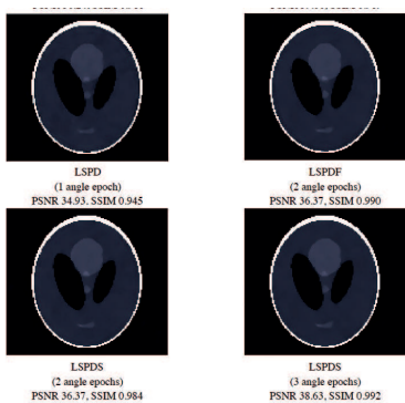
Fig 1. LSPD reconstructions from uniformly subsampled fixed 60 angles (over 180 degrees), grey level [0,1]
