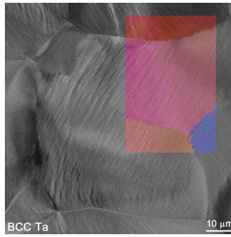
FIGURE 2. Example of grain boundaries in a pre-polished pure Ta sample with observed slip transfer in the middle grain boundary, and lack of slip transfer in boundaries at the top and bottom of the figure. The color overlay indicates grain orientations based upon a normal direction inverse pole figure map.
