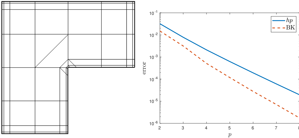
FIGURE 1. Left: geometric mesh \mathcal{T}_x that is anisotropically refined towards the edges and isotropically towards the vertices. Right: error versus polynomial degree p for s = 0.8 for the Galerkin method (3) (solid line) and Balakrishnan formula (9) (dashed line). \text{error} = \int_{\Omega} f(u - u_N) . For (3), q = p \sim L_x \sim L_y \sim \mathcal{Y} ; for (9) p \sim L_x \sim M . \Omega is shown on the left, f \equiv 1 .
