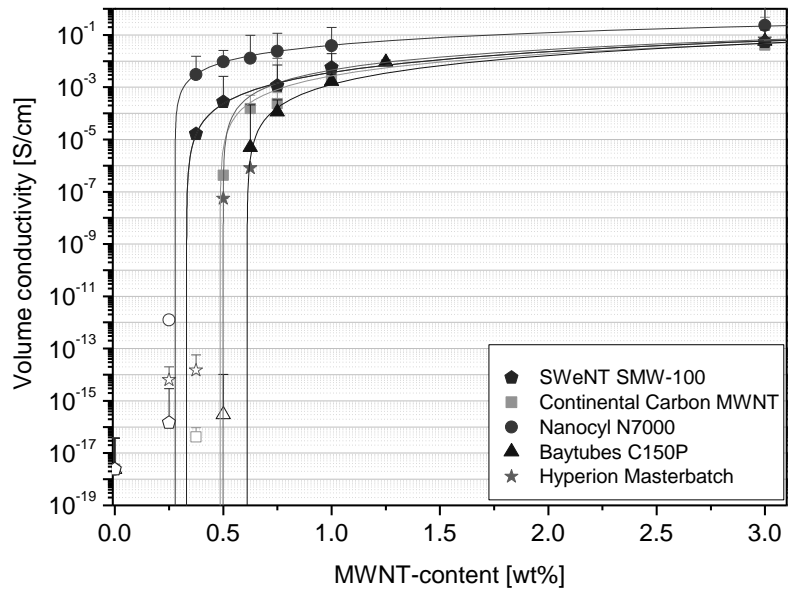
Figure 2: Electrical volume conductivity of polycarbonate composites containing different MWNTs and fitted curves according to equ. (2).
