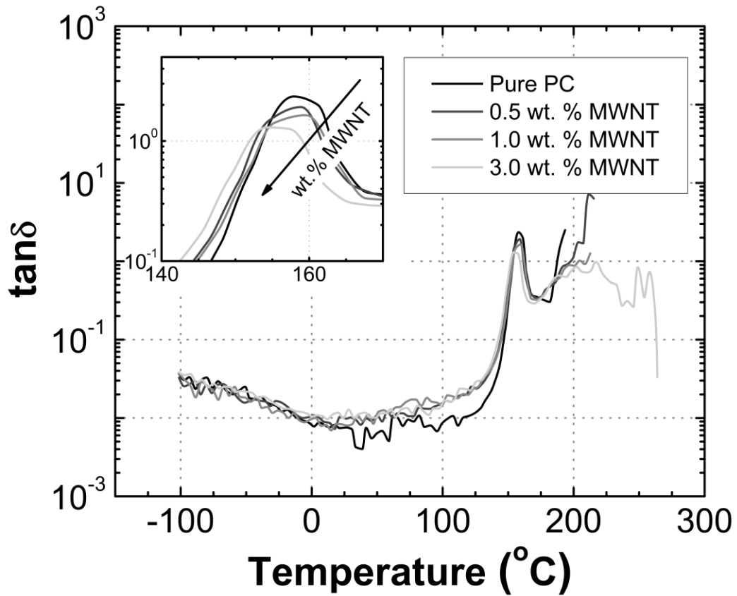
Figure 8: Loss factor ( \tan\delta ) vs. Temperature of pure polycarbonate and its composites with Nanocyl TM NC7000 with MWNT content of 0.5, 1.0 and 3.0 wt. %
