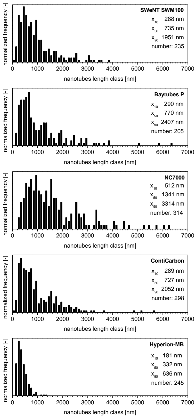
Figure 1: Length distributions of the nanotubes materials as measured by TEM, the number of measured tubes is named
