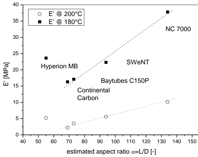
Figure 6: Storage modulus E' versus estimated mean aspect ratio, the lines were drawn to guide the eyes
