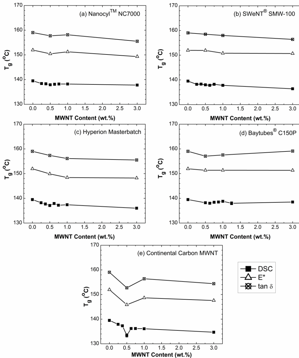
Figure 7: Glass transition temperature determined by DSC, E'' and \tan \delta , as a function of MWNT content for polycarbonate composites with different carbon nanotubes. Error bars were calculated from multiple measurements on the same sample for DSC measurements and are the same size as the symbols so are not discernible; no duplicates were run for the DMA data.
