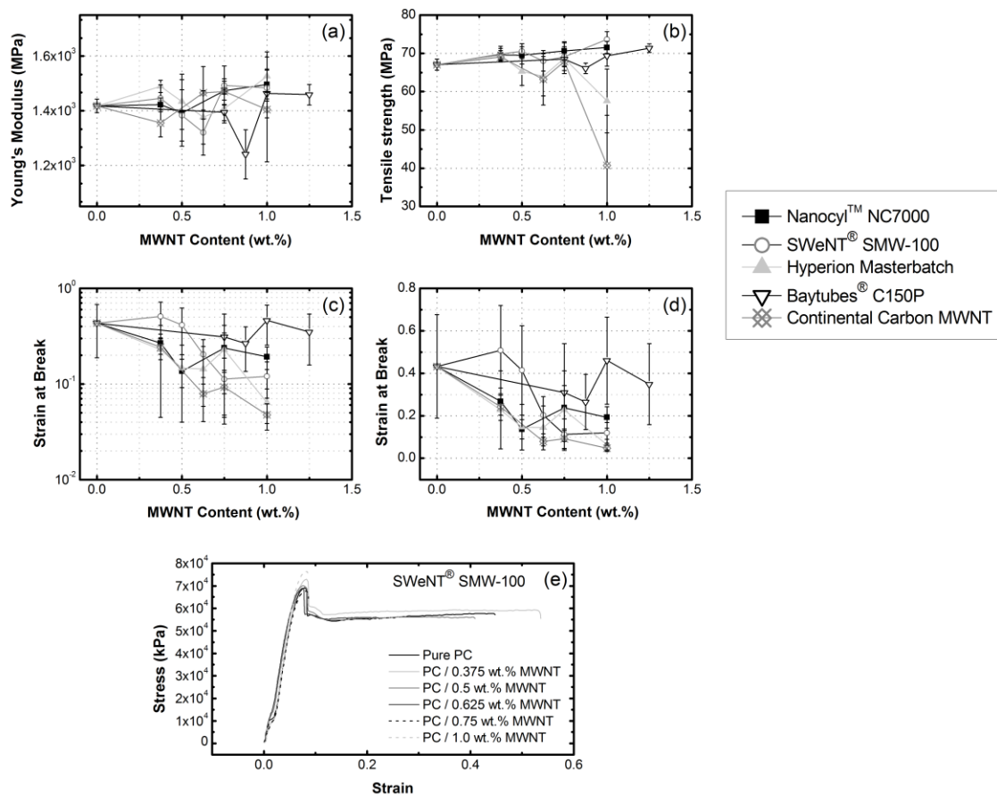
Figure 4: Young's Modulus (a) , tensile strength (b) and strain at break (c and d) vs. MWNT content of pure polycarbonate and its composites with Nanocyl™ NC7000, SWeNT® SMW-100, Hyperion Masterbatch, Baytubes® C150P and Continental Carbon MWNT. Graph (e) shows representative stress-strain curves for pure polycarbonate and composites made with SWeNT® SMW-100 at various weight fractions of nanotubes.
