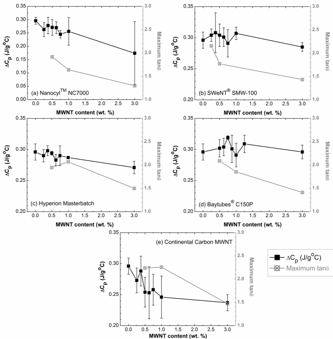
Figure 9: Change in heat capacity ( \Delta C_p ) and loss factor ( \tan\delta ) at glass transition peak versus MWNT content for pure polycarbonate and its composites with different multi-wall carbon nanotubes. Error bars were calculated from multiple measurements on the same sample; no duplicates were run for the DMA data.
