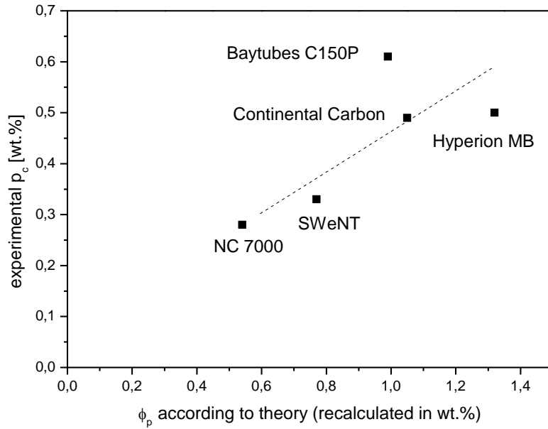
Figure 3: Experimental percolation concentration of different MWNTs in polycarbonate versus the calculated percolation concentration (according to equation (1)), the line was drawn to guide the eyes
