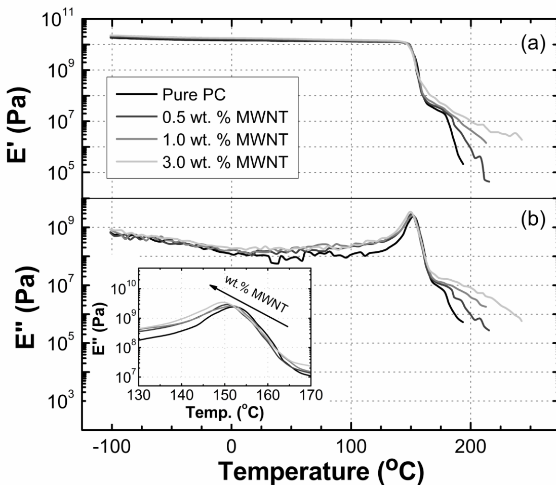
Figure 5: Storage (a) and Loss Moduli (b) of pure polycarbonate and its composites with Nanocyl ™ NC7000 with MWNT content of 0.5, 1.0 and 3.0 wt.%. The inset shows T_g determination from the maximum in E'' .
