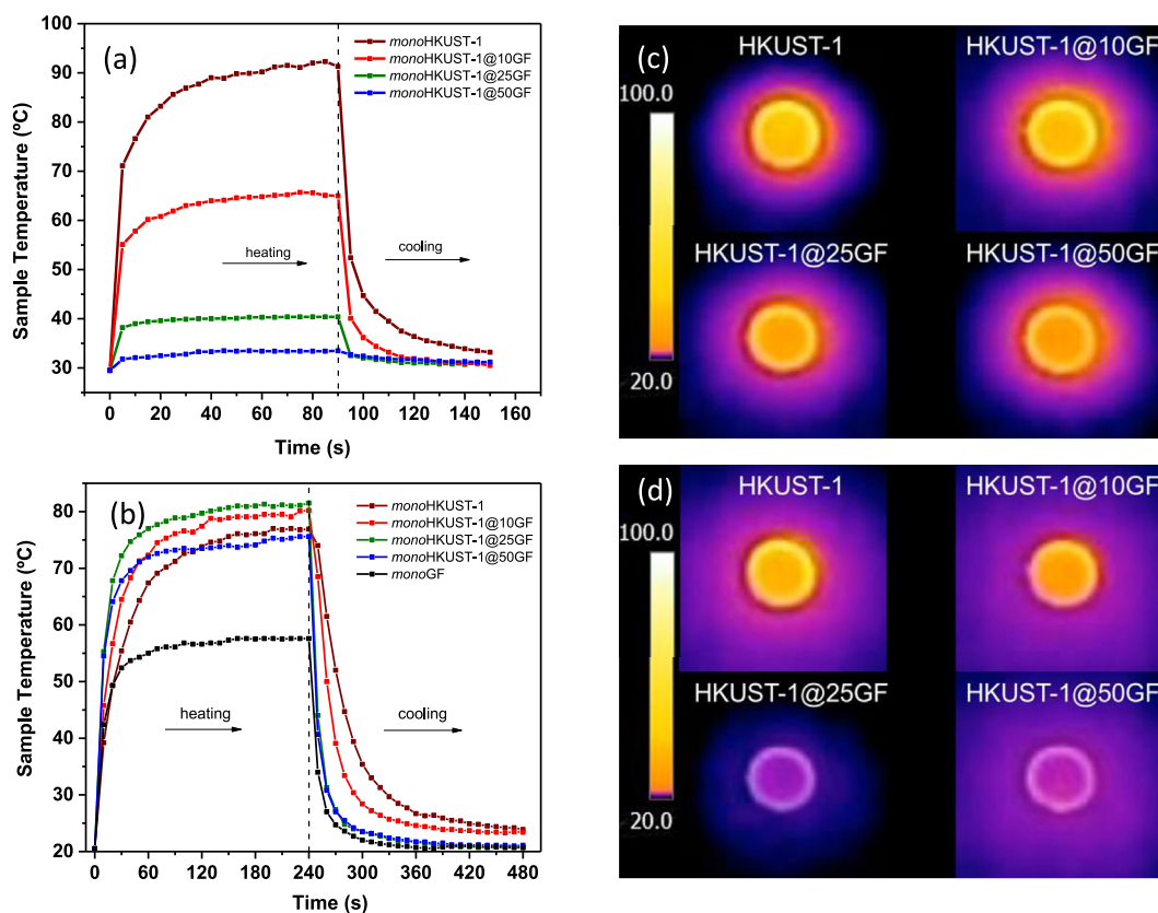
Fig. 5 – (a) Heating-cooling curves for samples monoHKUST-1 ; monoHKUST-1@10GF ; monoHKUST-1@25GF and monoHKUST-1@50GF upon irradiation with NIR laser irradiation (808 nm wavelength and 0.6 \text{ W cm}^{-2} of power irradiation), (b) Heating-cooling curves upon thermal heating on a ceramic surface at 90^\circ \text{C} , (c–d) Snapshots of the thermogravimetric camera in the cooling process at (c) t = 0 and (d) t = 10 \text{ s} (complete video is provided as a complementary material).
