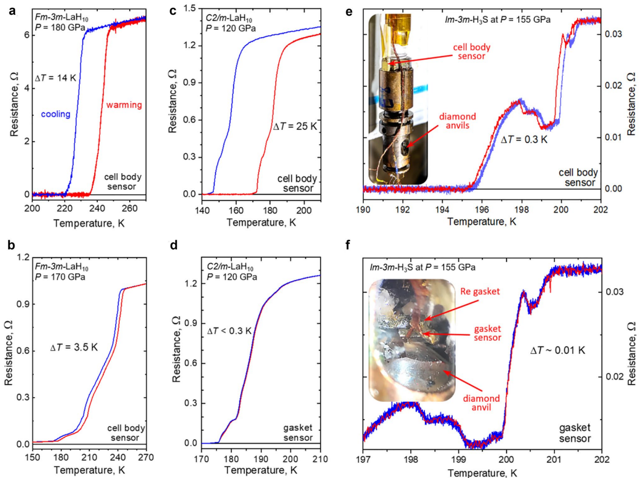
Fig. 1 The superconducting transitions in \text{LaH}_{10} and \text{H}_3\text{S} compounds detected through the temperature dependence of the electrical resistance upon cooling (blue curves) and warming (red curves). a, b R(T) measurements of the \text{Fm-3m-LaH}_{10} phase residing in a large DAC with an outer diameter of 33 mm. The temperature sweep dT/dt is \sim 1 \text{ K min}^{-1} upon cooling and \sim 0.3 \text{ K min}^{-1} upon warming. a The temperature sensor is attached to the body of DAC, leading to a hysteresis of \sim 14 \text{ K} . b The sensor is attached to the body of DAC and carefully insulated from the cooling gas. In this case, the hysteresis is significantly lower \sim 3.5 \text{ K} . c, d R(T) measurements of the \text{C2/m-LaH}_{10} phase in the miniature DAC with an outer diameter of
