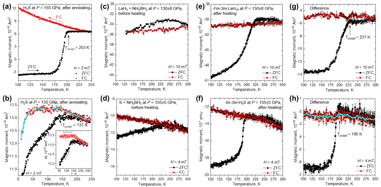
Fig. 5 Magnetization measurements under high pressures using the miniature DAC. a M(T) measurements of \text{H}_2\text{S} at 155 GPa (taken from Ref. [1]). b More typical, the smaller magnetic signal is registered from the \text{H}_2\text{S} sample at a pressure of 135 GPa. The measurements of the same sample in another run are shown in the inset. c–h The recent improved measurements of M(T) under high pressure with accurate background subtraction (taken from Ref. [55]). c, e, g M(T) data of the Fm\text{-}3m\text{-LaH}_{10} at 130 \pm 8 GPa under magnetic field H = 10
