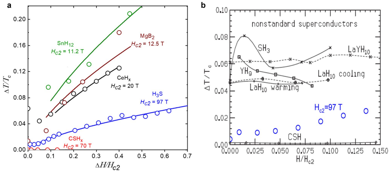
Fig. 4 Broadening of the superconducting transition under external magnetic fields in different superconducting compounds: a SnH 12 [68], MgB 2 [53], CeH x [69], H 3 S [41], C-S-H [24]. The related coordinates are chosen for easier comparison. The solid lines are a guide
