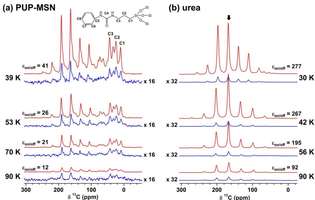
Fig. 1. DNP-enhanced ^{13}\text{C}\{^1\text{H}\} CPMAS spectra of PUP-MSN (a) and urea (b) obtained at indicated sample temperatures and \nu_R = 6 kHz. Red and blue lines represent the spectra taken with and without microwave irradiation, respectively. In (a), the resolved peaks are labeled in accordance with the molecular structure shown. In (b) the arrow marks the centerband.
