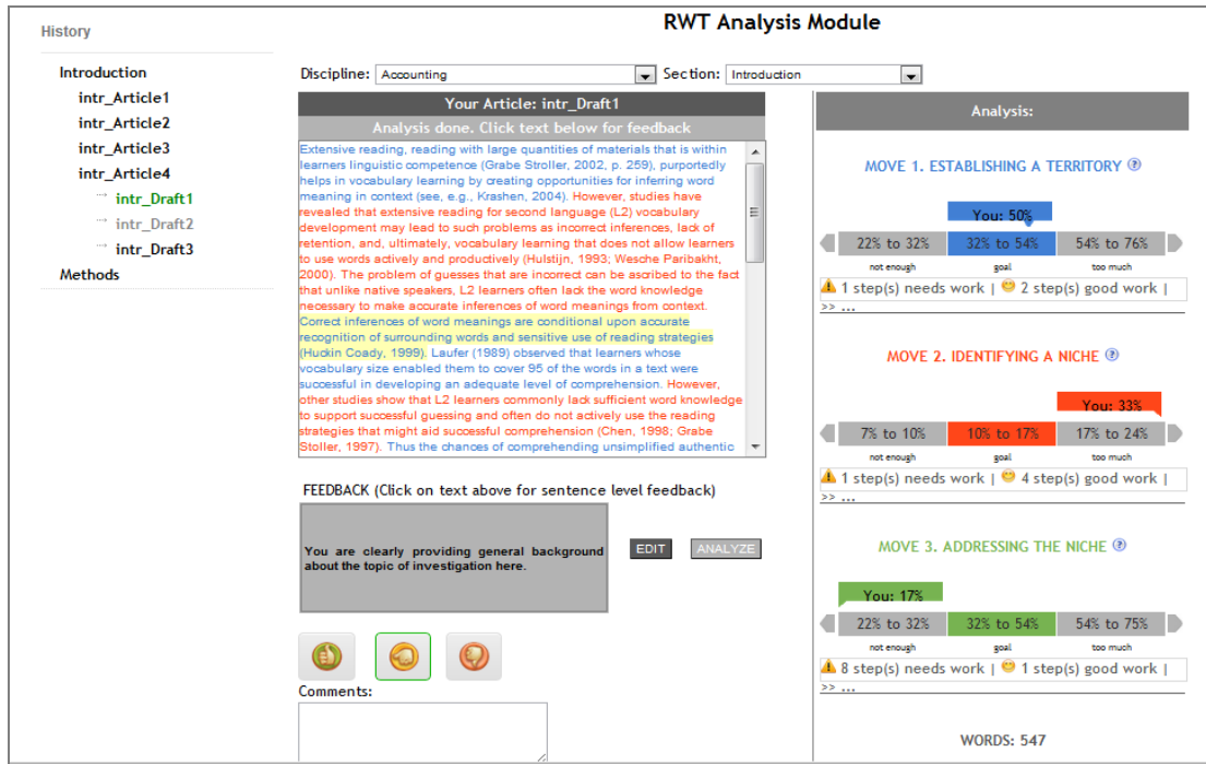
Figure 3.2: Analysis Module of RWT
