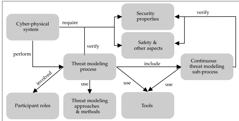
FIG.2: Model of the threat modeling concepts and the relationships among these concepts.
