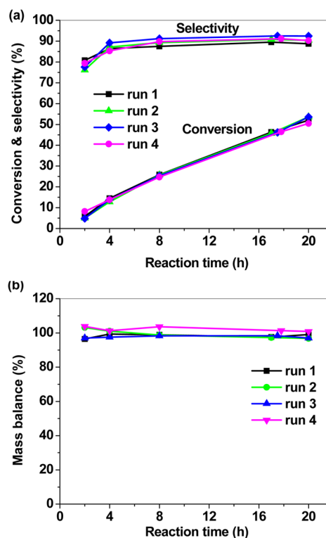
Figure 8. Kinetic studies of 10.7%Pt@UiO-66-NH 2 in cinnamaldehyde hydrogenation during recycle experiment: (a) conversion and selectivity to cinnamyl alcohol (CALC); (b) mass balance. Reaction conditions: 10 mL of methanol, 1 mL of NET 3 , 50 \mu L of mesitylene, 40 bar H 2 , 800 rpm, rt.
