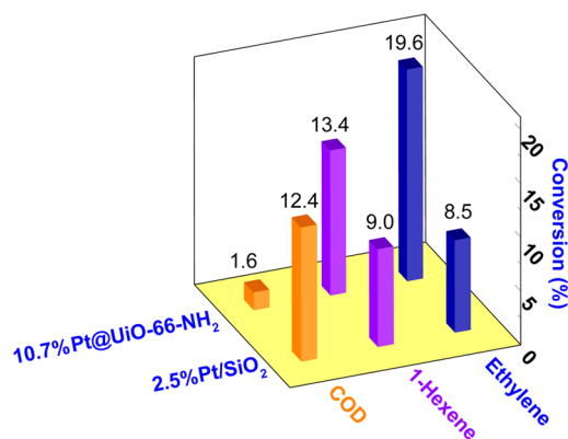
Figure 6. Comparison of 10.7%Pt@UiO-66-NH 2 (inside) and 2.5% Pt/SiO 2 in the hydrogenation of ethylene, 1-hexene and 1,3-cyclooctadiene (COD). Reaction conditions: C 2 H 4 /H 2 /He = 1.2/12/77 mL/min; 1-hexene/H 2 /He = 2.5/11/87 mL/min; COD/H 2 /He = 0.15/12/75 mL/min. The conversion was measured at −30 °C (ethylene), −10 °C (1-hexene), and 10 °C (COD), respectively. The same amount of Pt metal was used in the experiments.
