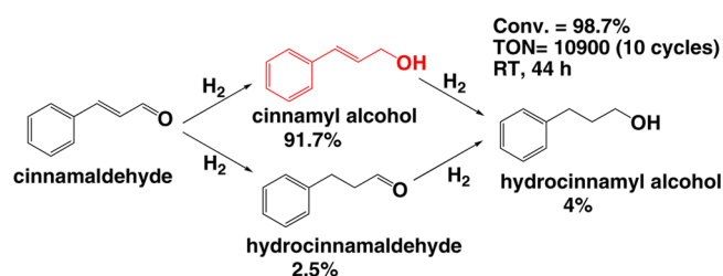
Scheme 1. Hydrogenation of Cinnamaldehyde a
