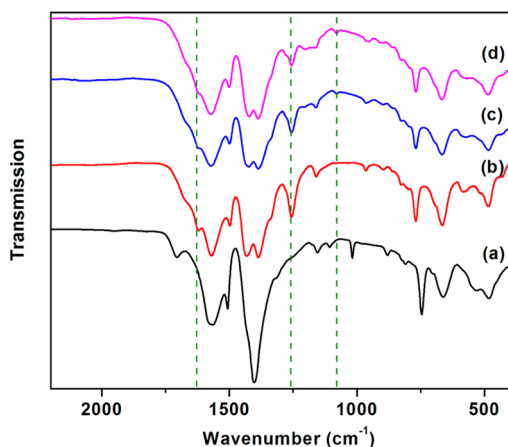
Figure 1. FT-IR spectra of (a) UiO-66, (b) UiO-66- \text{NH}_2 , (c) 10.7% Pt@UiO-66- \text{NH}_2 before reduction, and (d) 14.4%Pt@UiO-66- \text{NH}_2 before reduction.
