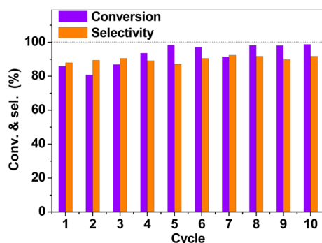
Figure 7. Recycle experiment of selective hydrogenation of cinnamaldehyde. Reaction conditions: 5.0 mg of 10.7%Pt@UiO-66-NH 2 , 10 mL of methanol, 1 mL of triethylamine, 400 \mu L of cinnamaldehyde, 20 \mu L of mesitylene, 40 bar H 2 , 25 ^{\circ} C, reaction time of 44 h (42 h for the first three runs).
