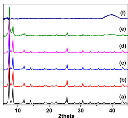
Figure 5. Powder XRD patterns of 10.7%Pt@UiO-66-NH 2 (a) before reduction, and after 1 h reduction at (b) 100 °C, (c) 150 °C, (d) 200 °C, (e) 250 °C, and (f) 300 °C.
