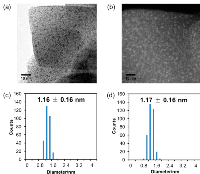
Figure 3. (a) Bright field TEM and (b) HAADF-STEM images of 10.7%Pt@UiO-66-NH 2 . (c) And (d) histogram of the size distribution of Pt NCs measured from the bright field TEM and the HAADF-STEM images of Pt NCs, respectively.
