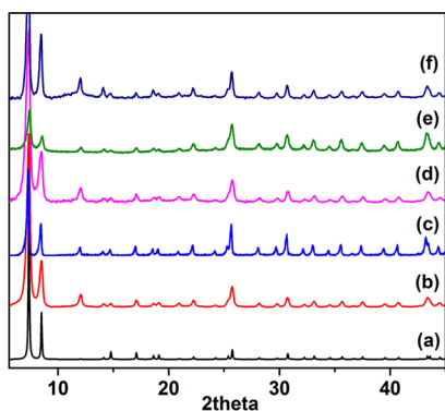
Figure 4. Powder XRD patterns of (a) simulated UiO-66, (b) as-synthesized UiO-66, (c) as-synthesized UiO-66-NH 2 , (d) 0.6%Pt@UiO-66 after reduction, (e) 3.6%Pt@UiO-66-NH 2 after reduction, and (f) 10.7%Pt@UiO-66-NH 2 after reduction.
