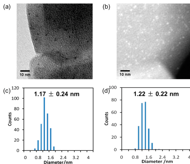
Figure 2. (a) Bright field TEM and (b) HAADF-STEM images of Pt NCs synthesized inside the cages of UiO-66- \text{NH}_2 , 0.97%Pt@UiO-66- \text{NH}_2 . (c) and (d) histogram of the size distribution of Pt NCs measured from the bright field TEM and the HAADF-STEM images of Pt NCs, respectively.
