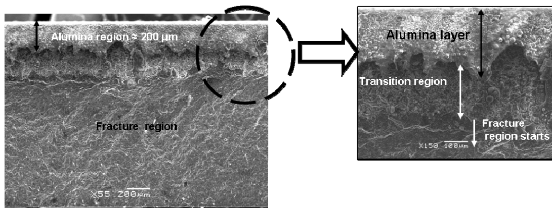
Figure 6.5: Single pass LWJ cut of 1.6mm thick CBN
