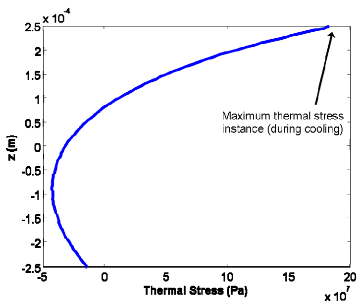
Figure 5.9: Stress distribution across the thickness for laser and LWJ machining
