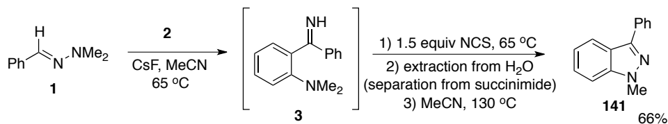
Scheme 25. Optimized of the Synthesis of Indazoles from Ketimines.
