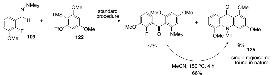
Scheme 11. Synthesis of a Naturally-occurring Acridone.
