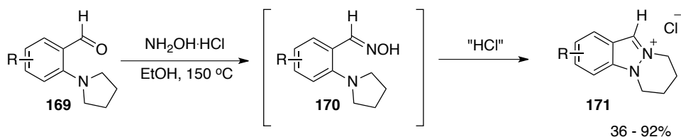
Scheme 26. Synthesis of Indazoles by Rebek.
