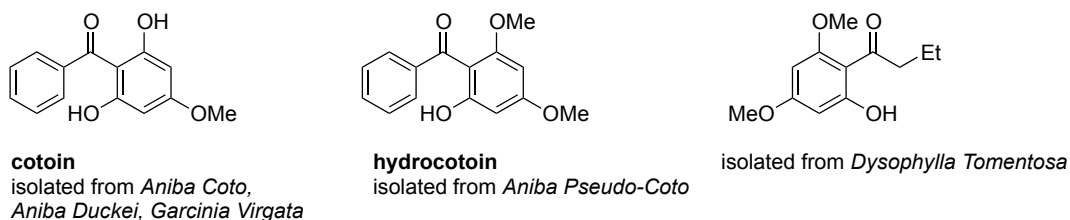
Scheme 4. Examples of Naturally-occurring o -Hydroxyaryl Ketones.
