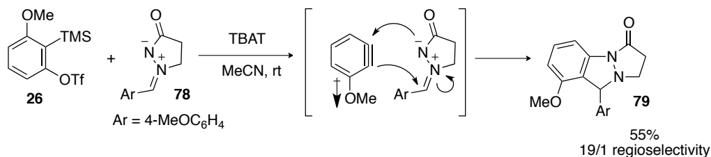
Scheme 28. Reaction with 3-Methoxybenzyne.
