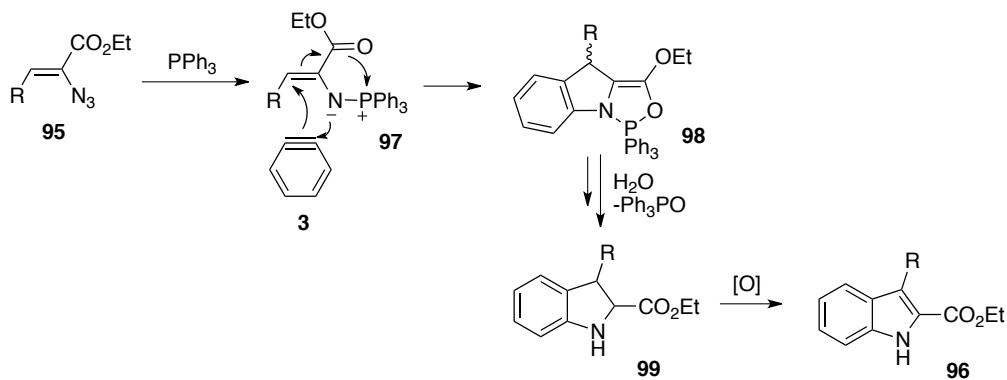
Scheme 35. Plausible Mechanism for the Coupling of Azo-ylides and Arynes.
