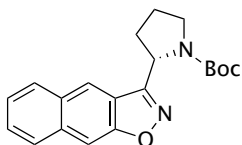
(S)-3-(N-Boc-pyrrolidin-2-yl)naphtho[2,3]isoxazole (59). This
