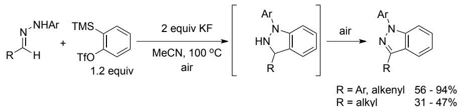
Scheme 20. Alternative Reported Route to 1-Arylidazoles.
