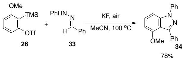
Scheme 13. Reaction with 3-Methoxybenzyne.
