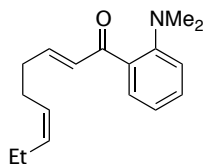
(2E,6Z)-1-[2-(Dimethylamino)phenyl]nona-2,6-dien-1-one (50). This
