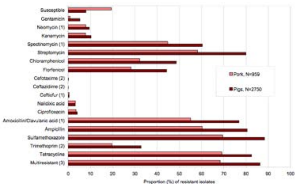
Fig. 3: Resistance of S. Typhimurium from pigs and pork in Germany to selected antimicrobials (2000 – 2009)
