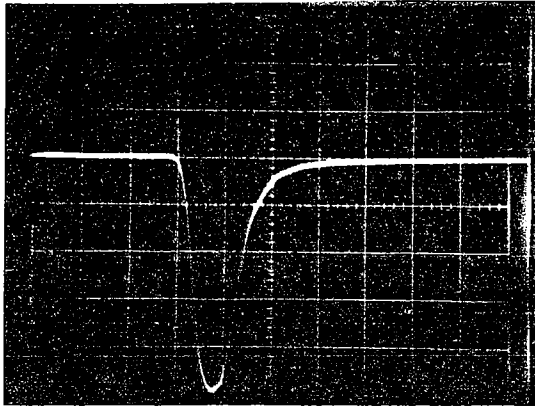
Fig. 9. Oscilloscope of voltage impulse employed to excite source transducer. Vertical - 50 V/div. Horizontal - 50 nsec/div.
