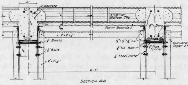
Fig. 22. Details of steel roof forms.
