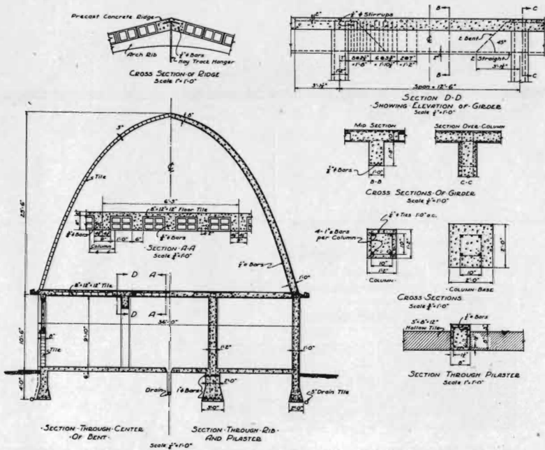
Fig. 18. Cross section and typical details of the experimental barn.
