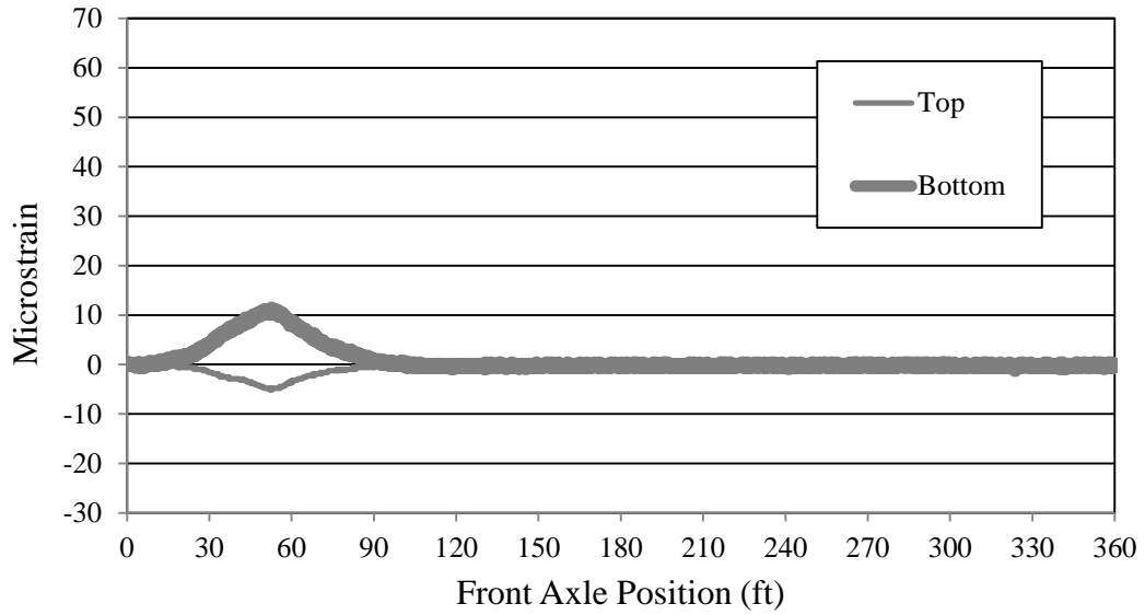
Figure 7.13. Bridge 309 inner diaphragm strain (LP2)
