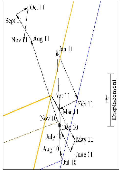
Figure 6.87. Bridge 2208 movement at south pier west and east reflectors
