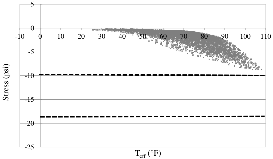
Figure 6.51. Southeast abutment backwall pressure versus effective temperature
