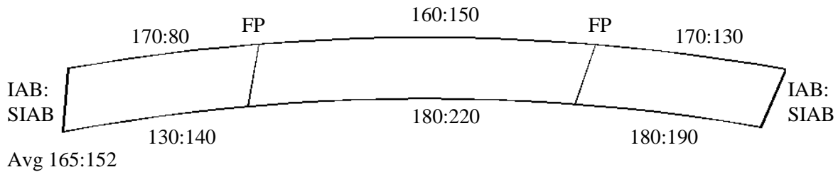
Figure 6.19. Bridge 309:2308 axial strain range
