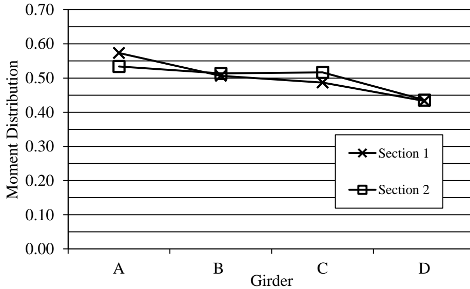
Figure 7.36. Bridge 309 maximum moment distribution factors
