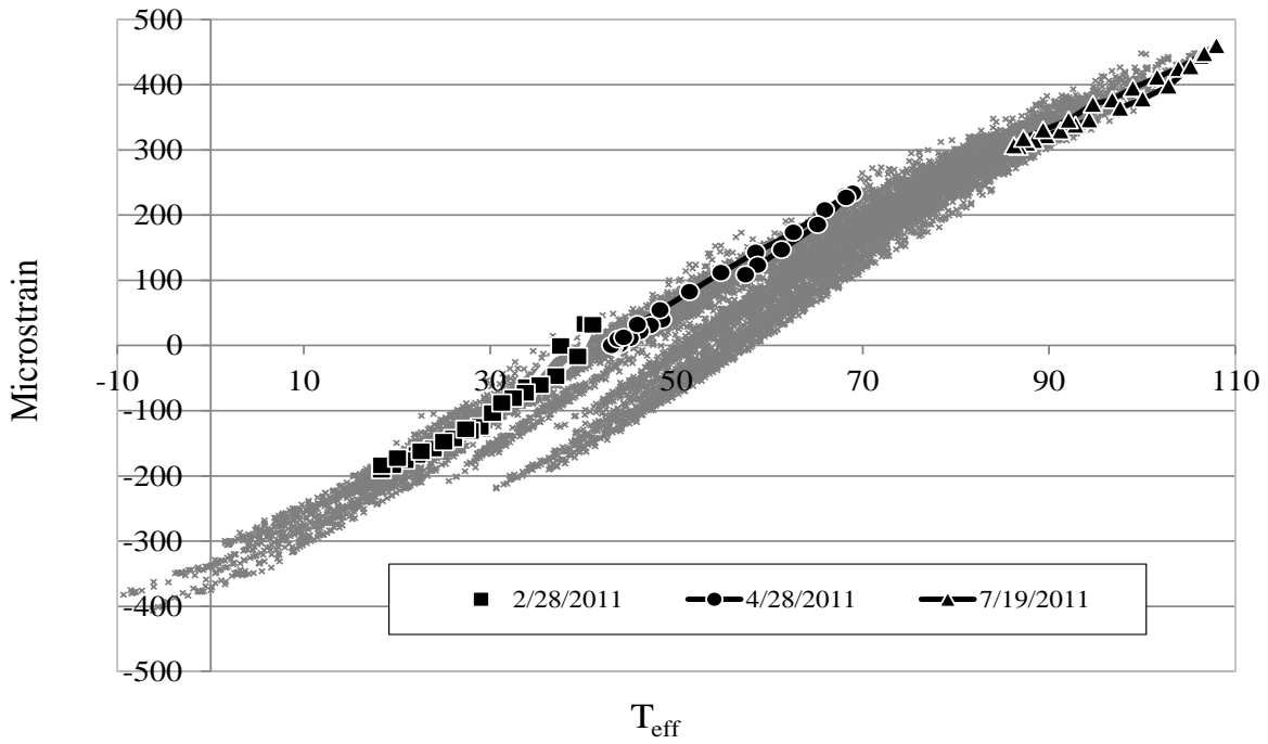
Figure 6.46. Typical internal minor axis bending strain
