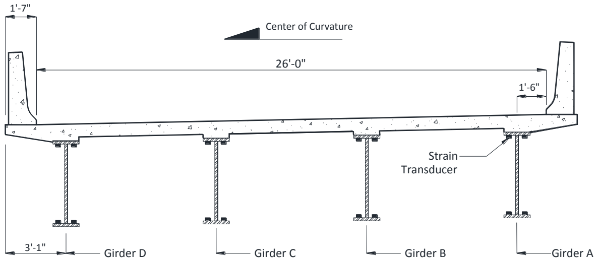
Figure 5.35. Section 1 strain transducer locations
