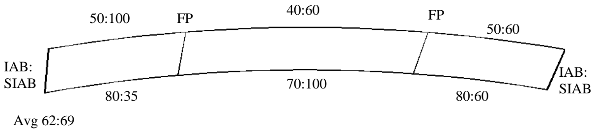
Figure 6.22. Bridge 309:2308 strong axis bending strain range
