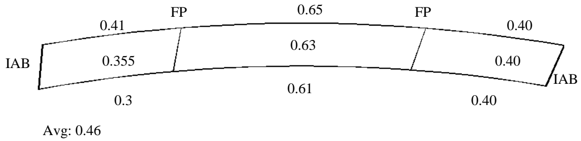
Figure 6.62. Bridge 309 change in length per span
