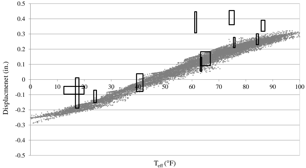
Figure 6.99. Expansion pier displacement
