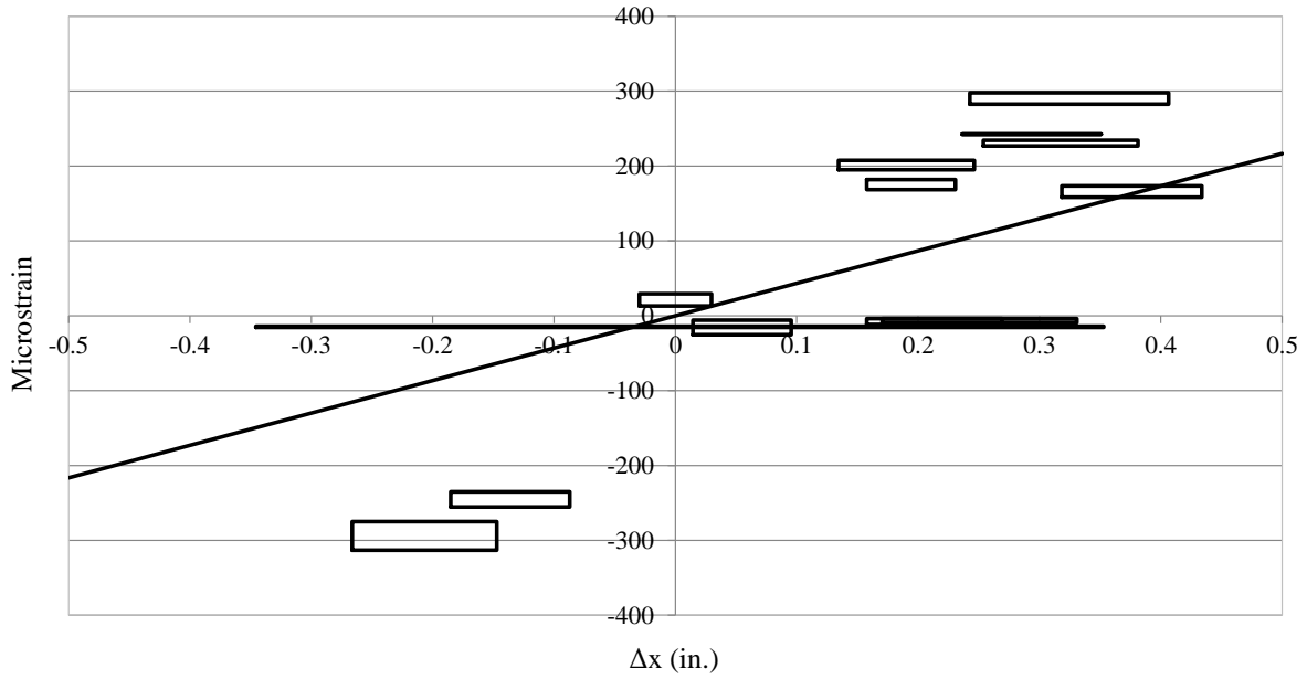
Figure 6.103. SAHP6 weak axis bending strain versus displacement
