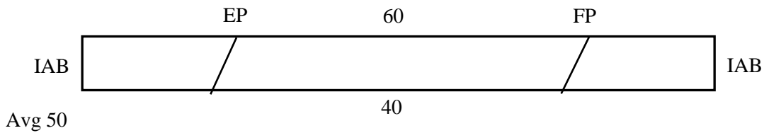
Figure 6.27. Bridge 109 lateral bending strain top flange
