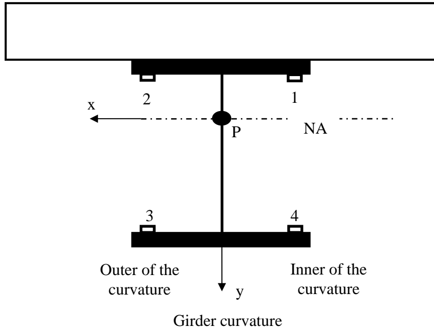
Figure 9.2. Stress points in girder section
