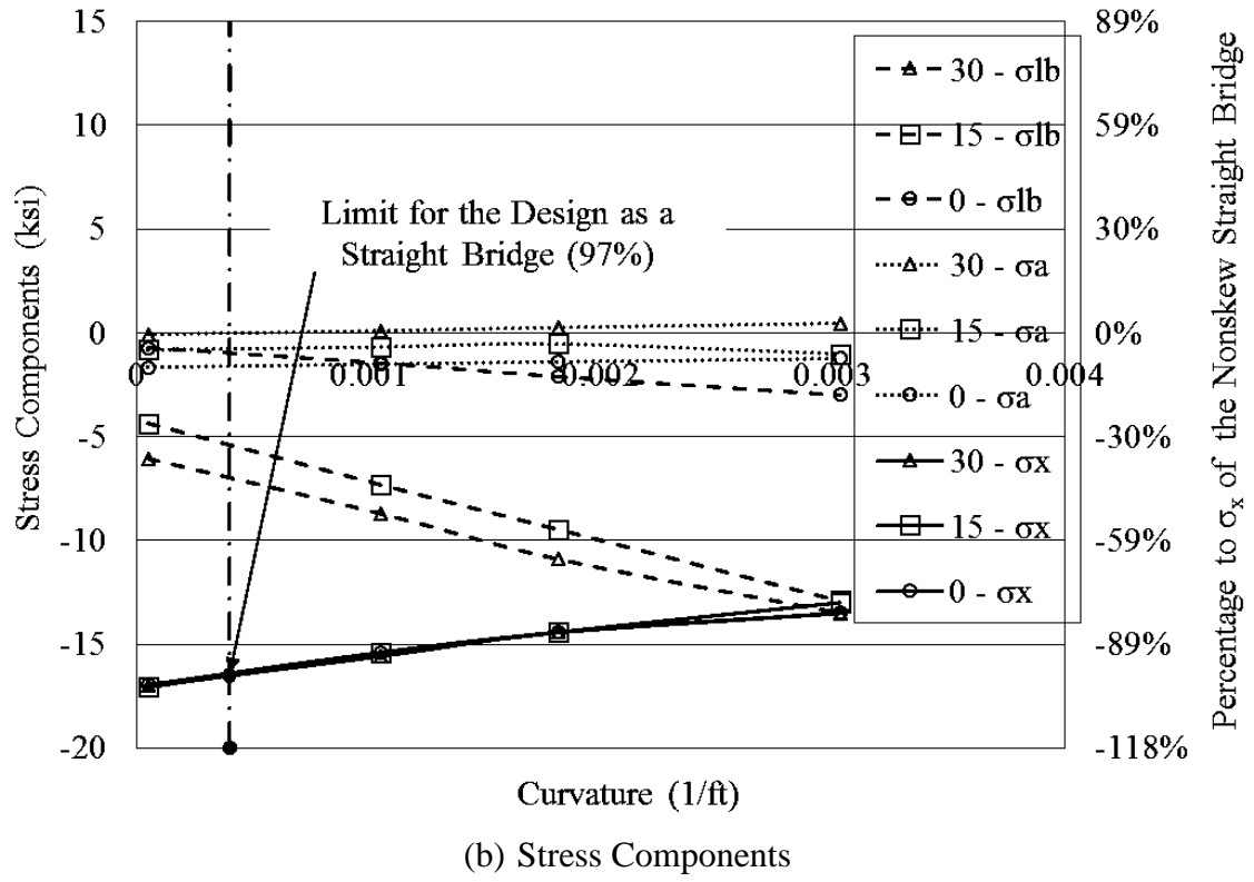
Figure 9.11. Total and component stresses in Girder D at north pier due to DL+LL+T(+)
