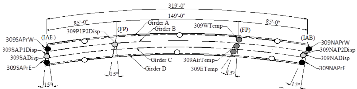
Figure 5.23. Bridge 309 instrumentation
