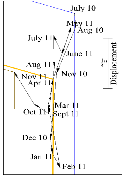
Figure 6.81. Bridge 309 movement at north abutment west and east reflectors
