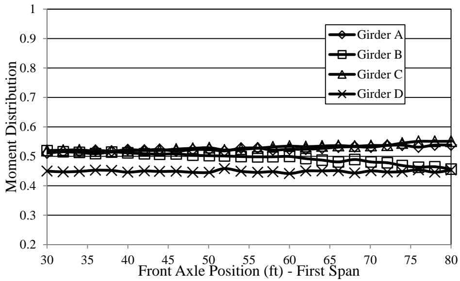
Figure 7.35. Bridge 309-S2 moment distributions versus truck position
