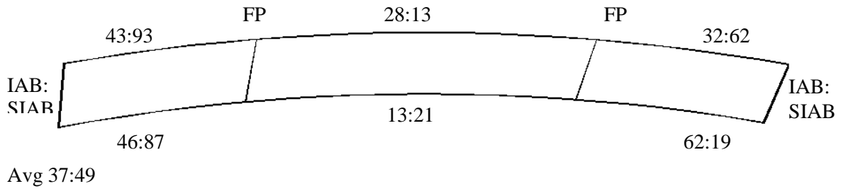
Figure 6.37. Bridge 309:2308 lateral bending moment top flange
