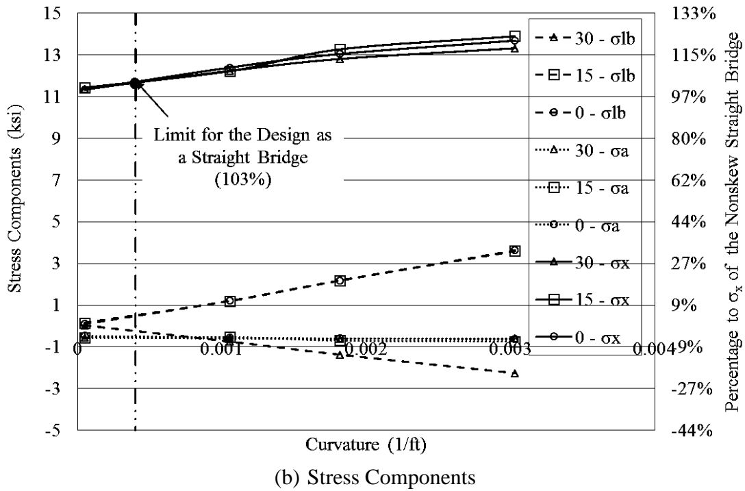
Figure 9.9. Total and component stresses in Girder A at mid-center span due to LL
