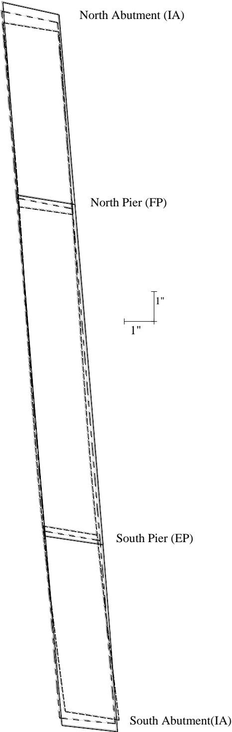
Figure 6.67. Bridge 109 deflected shape
