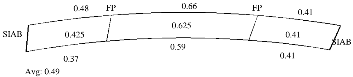
Figure 6.64. Bridge 2308 change in length per span
