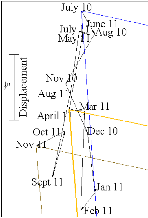
Figure 6.73. Bridge 109 movement at north abutment west and east reflectors
