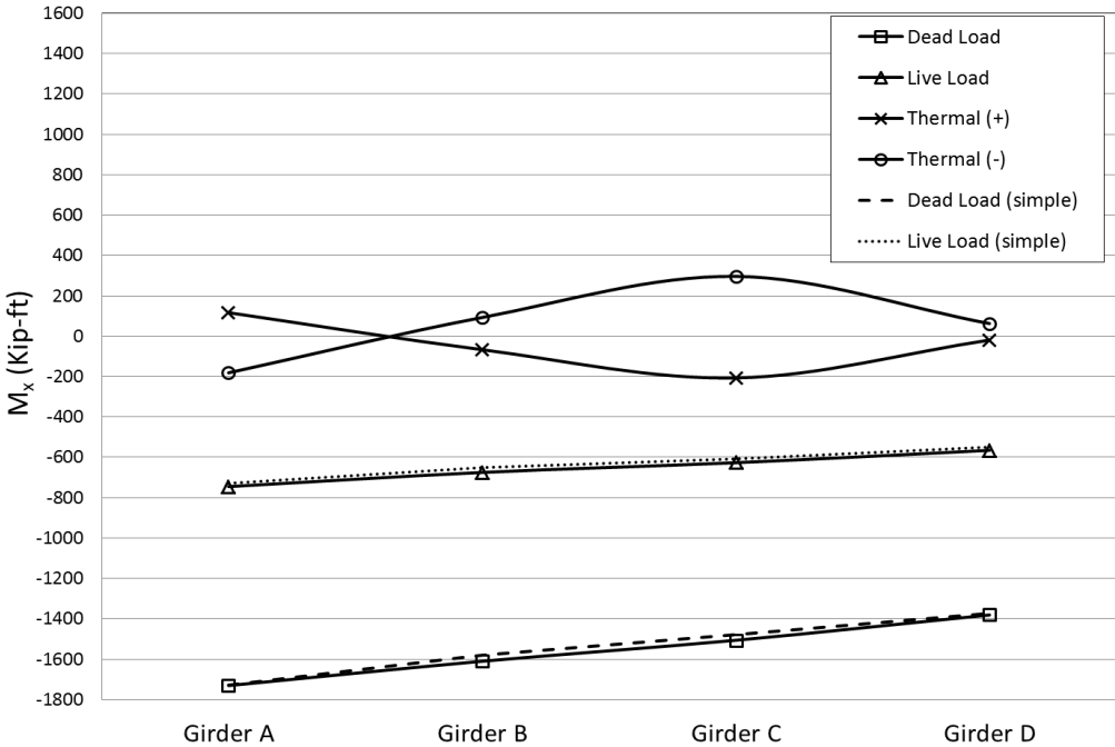
Figure 8.26. North pier Service I loads
