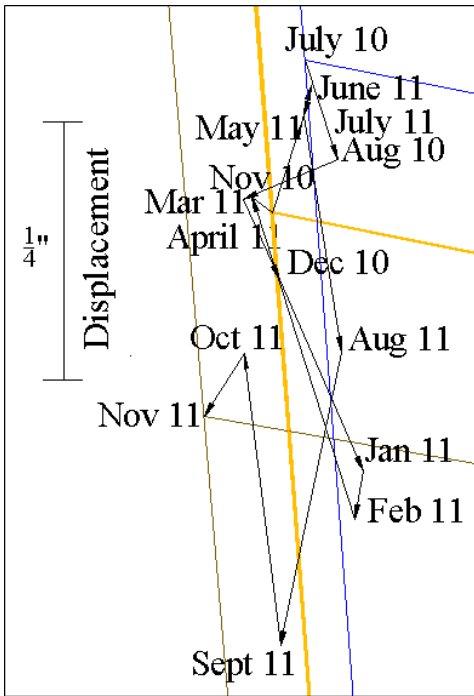
Figure 6.74. Bridge 109 movement at north pier west and east reflectors
