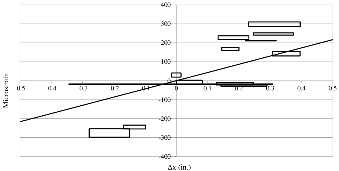
Figure 6.106. NAHP6 weak axis bending strain versus displacement
