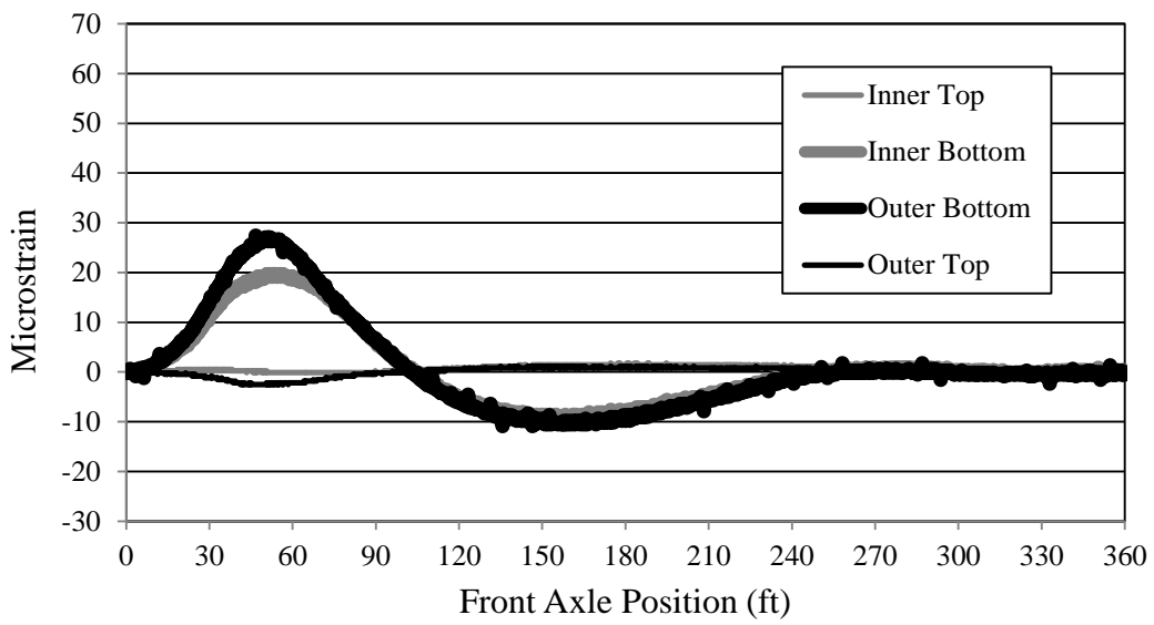
Figure 7.5. Bridge 309-S2 Girder A strain (LP2)
