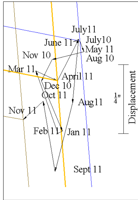
Figure 6.74. Bridge 109 movement at north pier west and east reflectors
