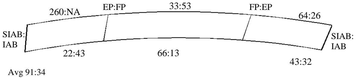
Figure 6.38. Bridge 209:2208 lateral bending moment top flange
