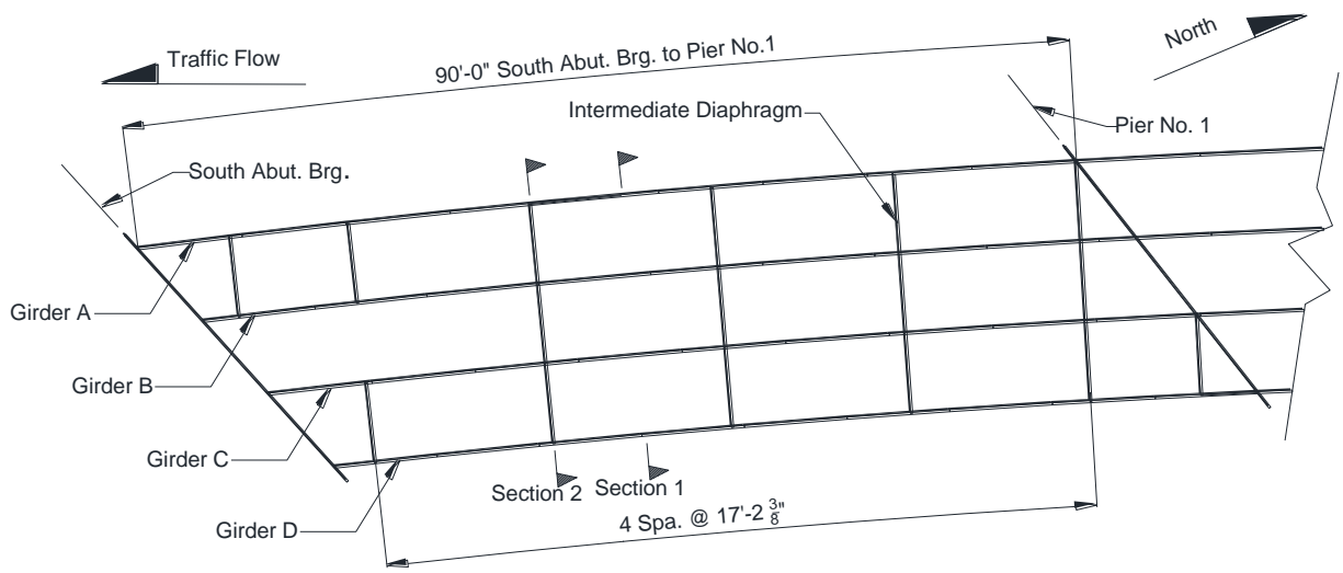
Figure 5.31. Bridge 209 plan view
