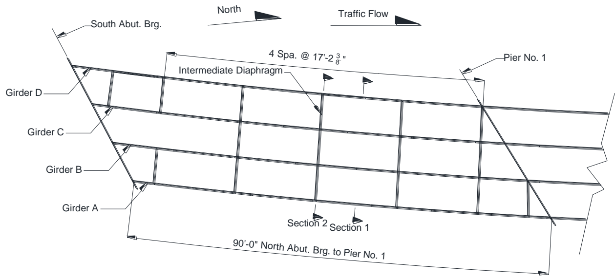
Figure 5.32. Bridge 2208 plan view
