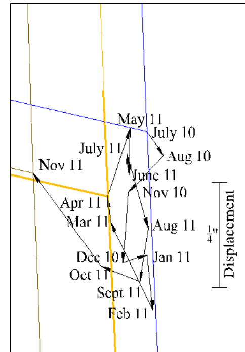
Figure 6.82. Bridge 309 movement at north pier west and east reflectors
