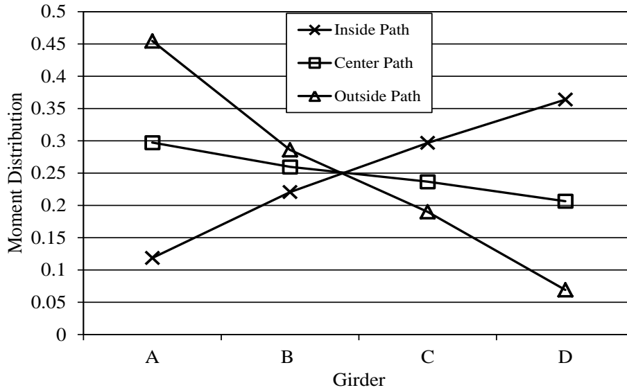
Figure 7.32. Bridge 309-S1 single lane moment distributions for three truck lanes
