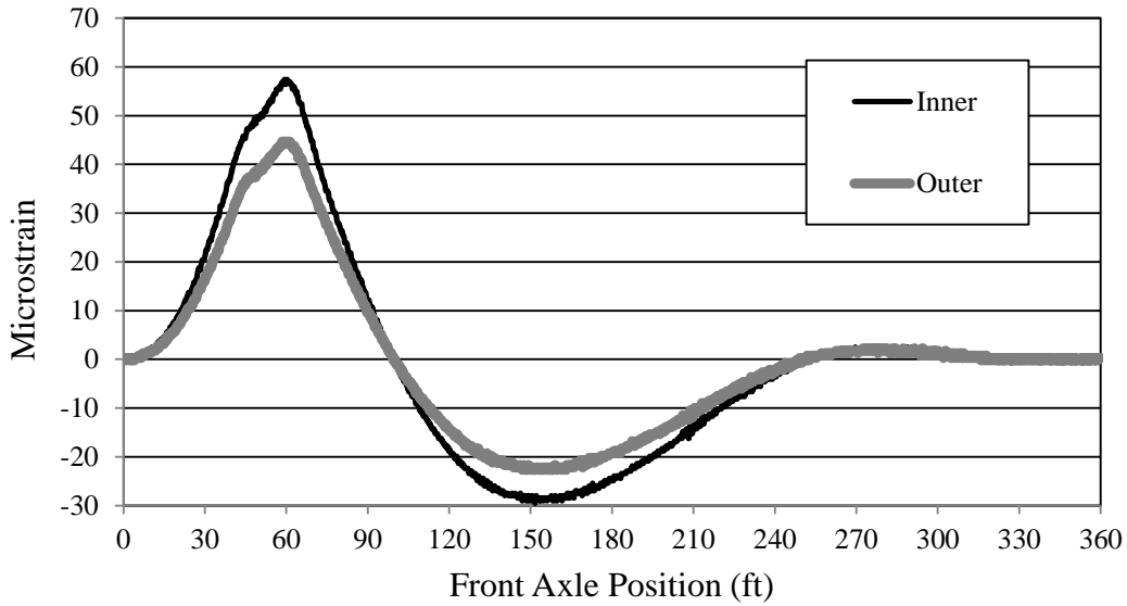
Figure 7.9. Bridge 309-S1 Girder A bottom flange strain (LP3)
