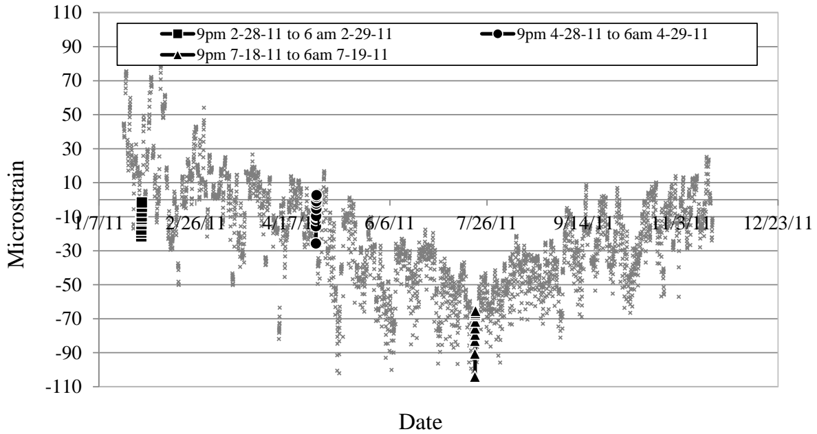
Figure 6.10. Axial strain versus time
