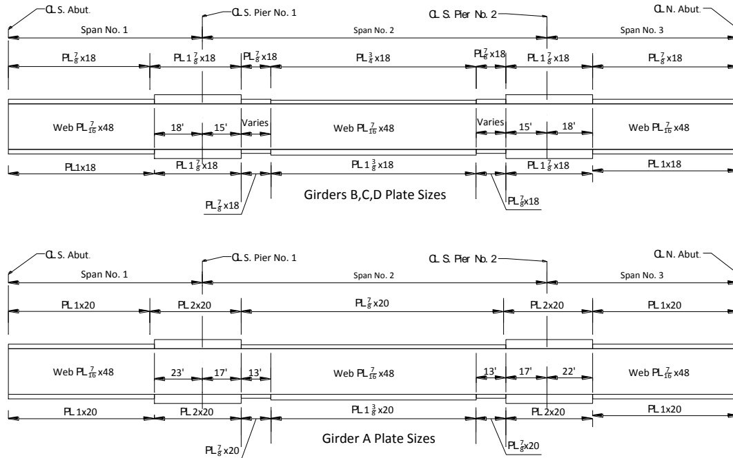
Figure 8.2. Plate girder sizes elevation view
