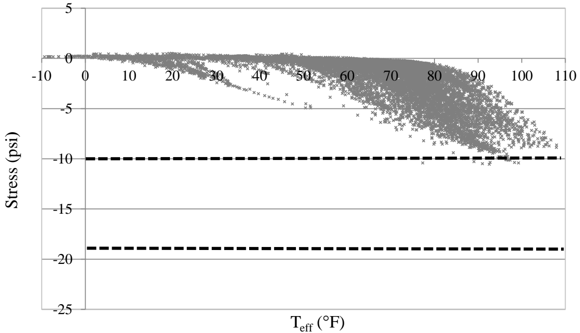
Figure 6.50. Southwest abutment backwall pressure versus effective temperature
