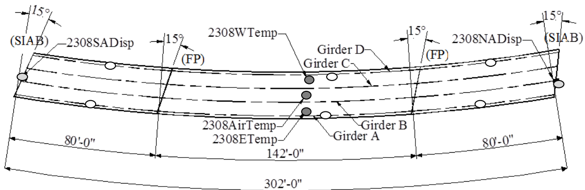
Figure 5.25. Bridge 2308 instrumentation
