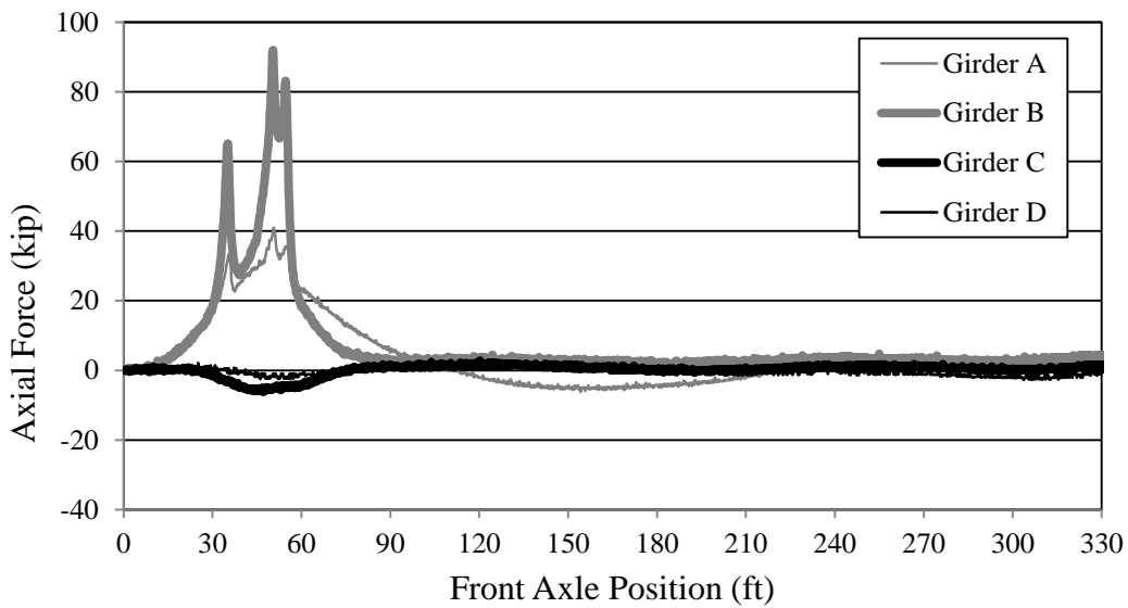
Figure 7.28. Bridge 309-S2 axial forces in girders (LP3)
