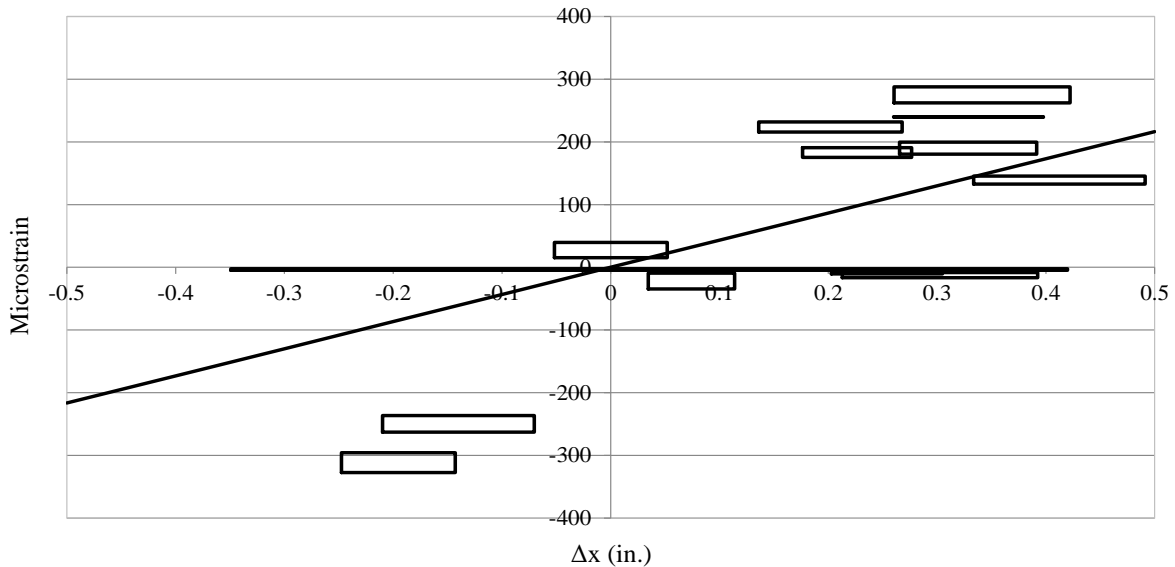
Figure 6.102. SAHP4 weak axis bending strain versus displacement
