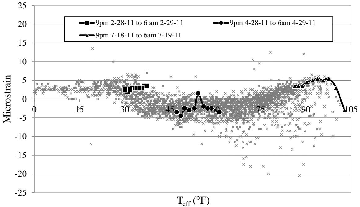
Figure 6.16. Top flange lateral bending versus T_{eff}
