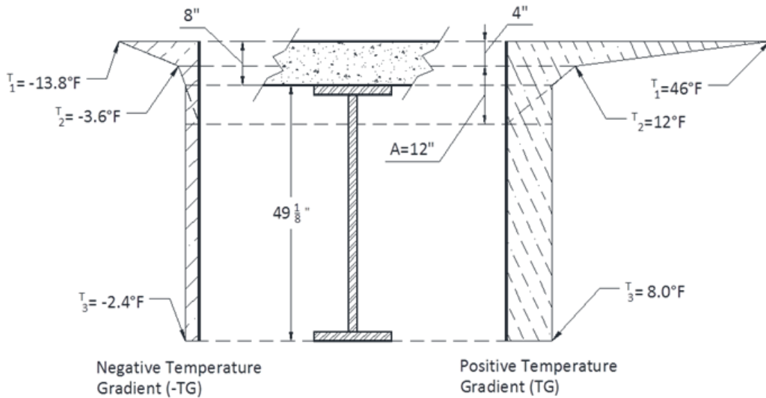
Figure 8.25. Temperature gradient
