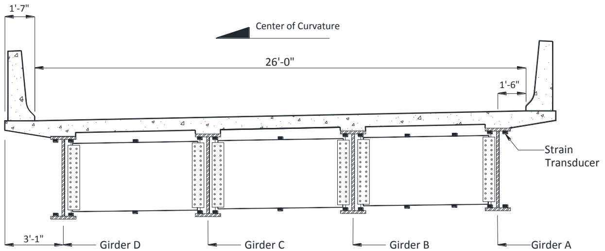
Figure 5.36. Section 2 strain transducer locations
