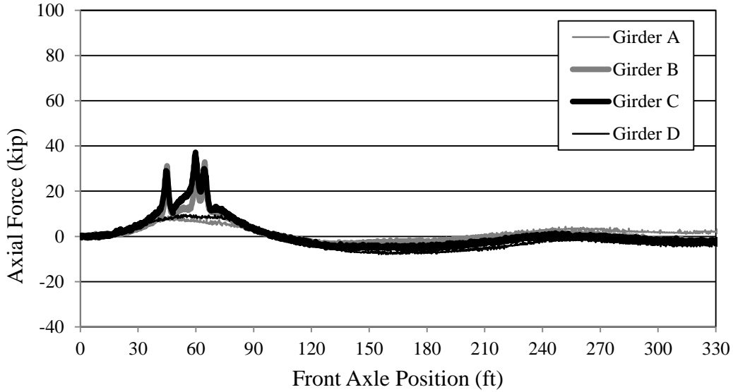
Figure 7.27. Bridge 309-S1 axial forces in girders (LP3)
