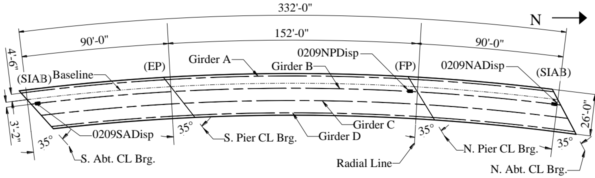
Figure 5.3. Bridge 209 plan view
