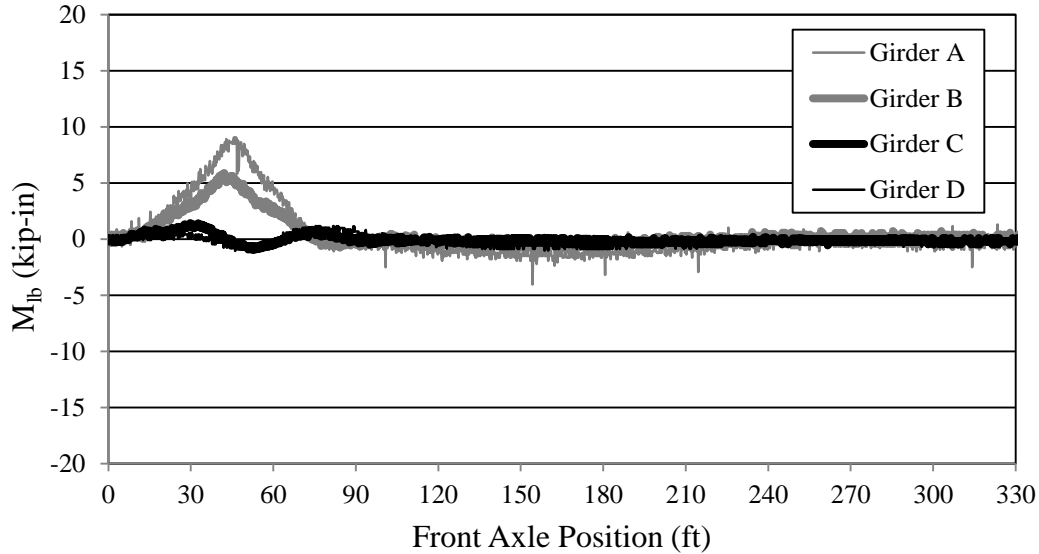
Figure 7.25. Bridge 309-S2 lateral bottom flange moments (LP3)
