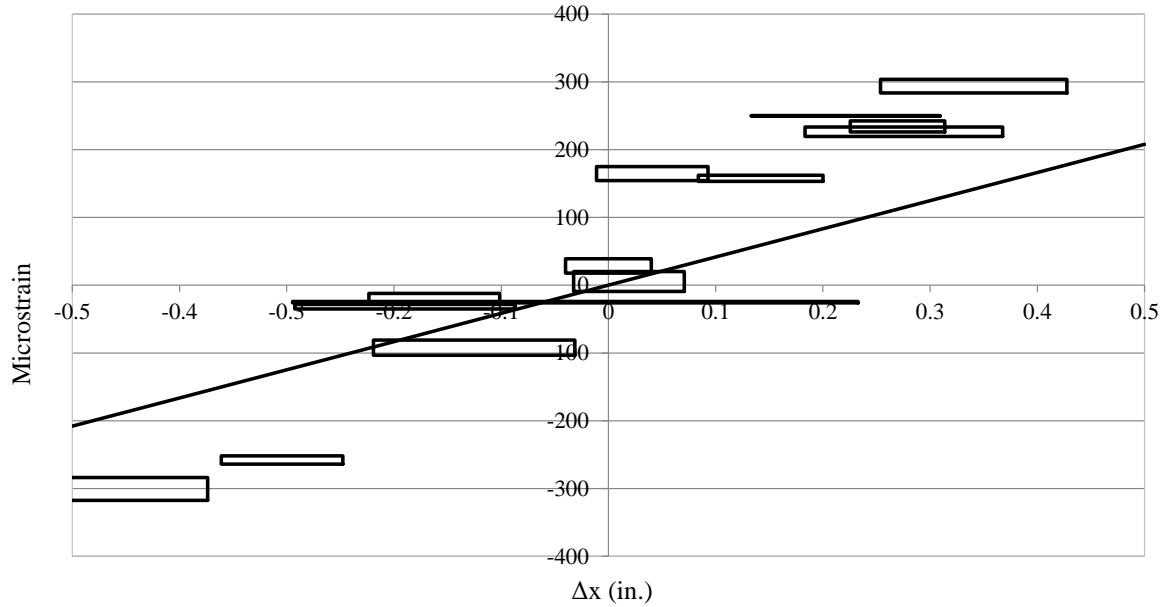
Figure 6.105. NAHP4 weak axis bending strain versus displacement
