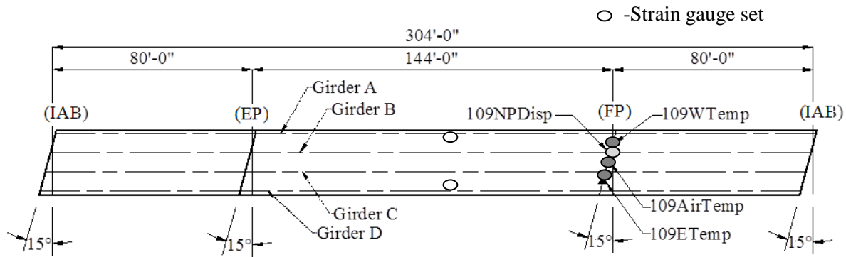
Figure 5.21. Bridge 109 instrumentation
