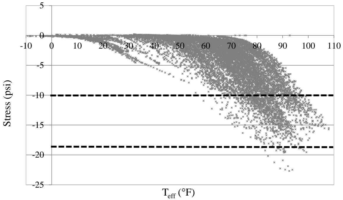
Figure 6.49. Northeast abutment backwall pressure versus effective temperature
