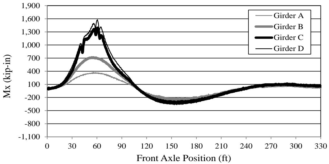
Figure 7.21. Bridge 309-S1 strong axis moments in girders (LP1)
