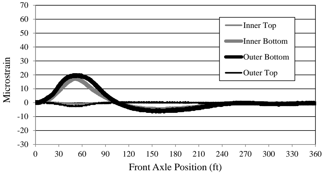
Figure 7.8. Bridge 309-S2 Girder D strain (LP2)
