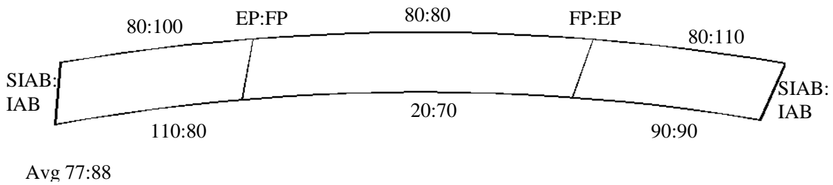
Figure 6.23. Bridge 209:2208 strong axis bending strain range
