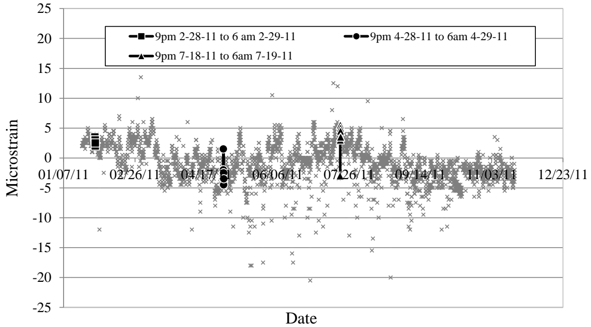
Figure 6.12. Top flange lateral bending versus time
