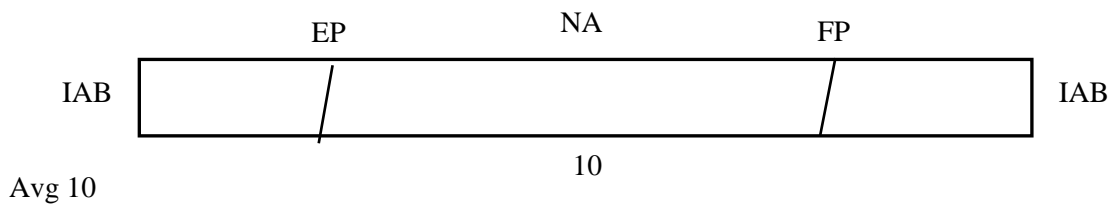
Figure 6.30. Bridge 109 lateral bending strain bottom flange
