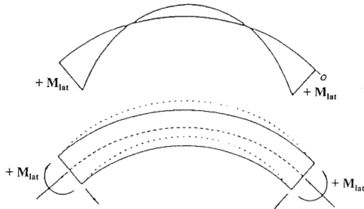
Figure 2.4. Lateral flange bending (from Figure A-1 Hall et al. 1999)
