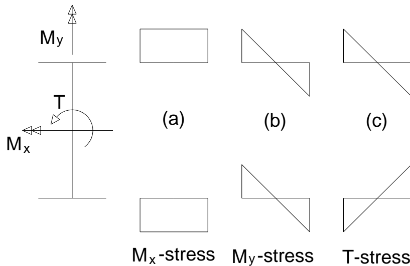
Figure 2.2. Normal stress in flanges due to three moment components
