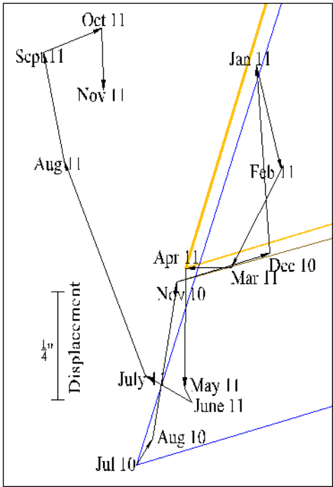
Figure 6.88. Bridge 2208 movement at south abutment west and east reflectors
