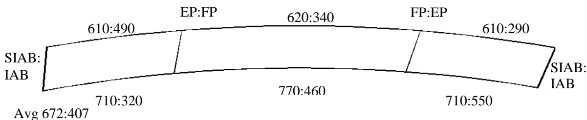
Figure 6.32. Bridge 209:2208 axial force range
