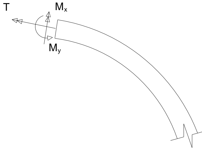
Figure 2.1. Three moment components in a single curved girder
