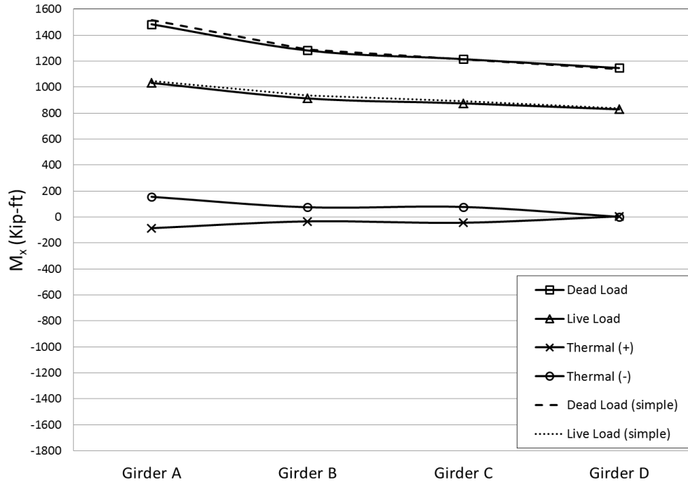
Figure 8.27. Center span Service I loads
