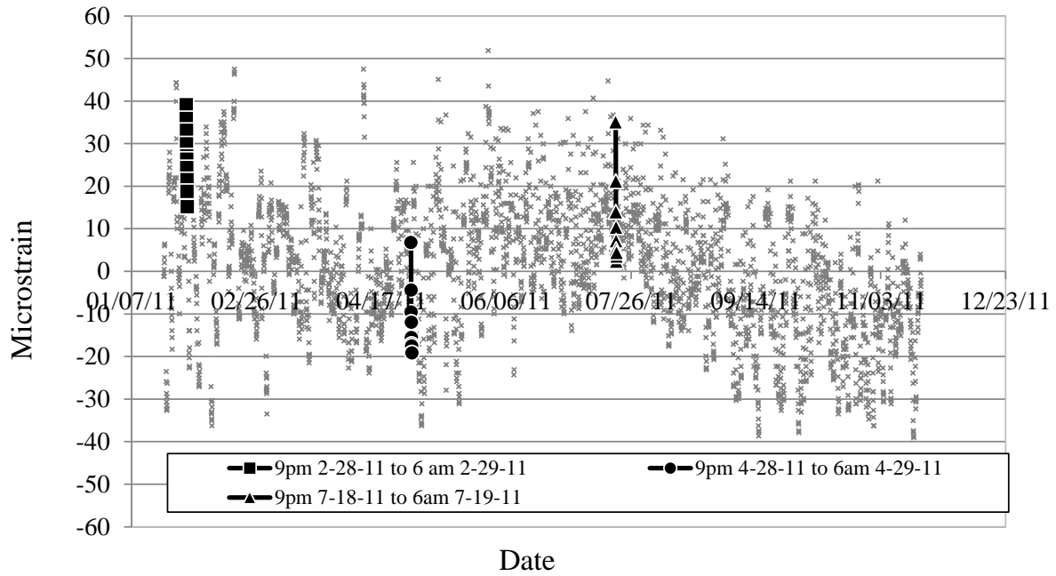
Figure 6.11. Major axis bending versus time
