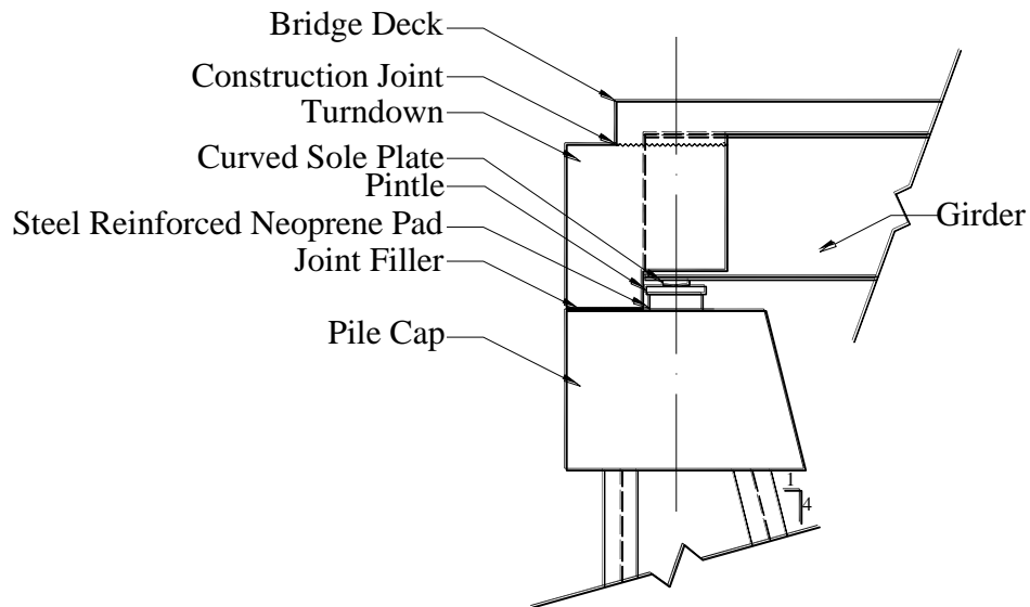
Figure 5.15. Semi-integral abutment Section A-A
