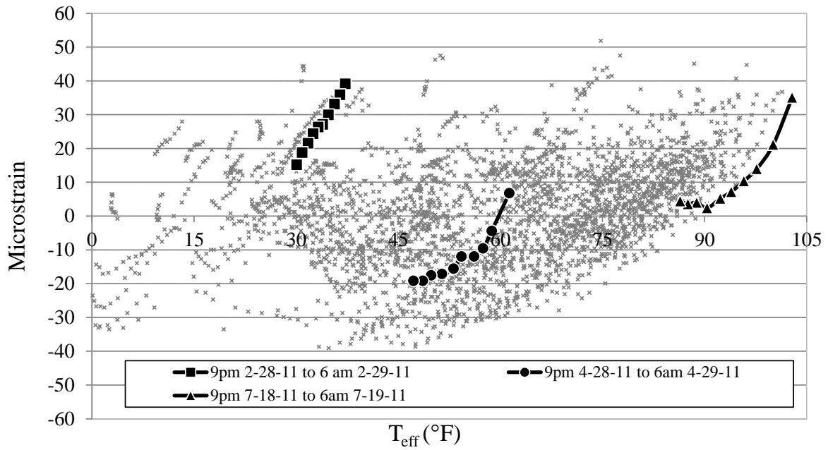
Figure 6.15. Major axis bending versus T_{eff}
