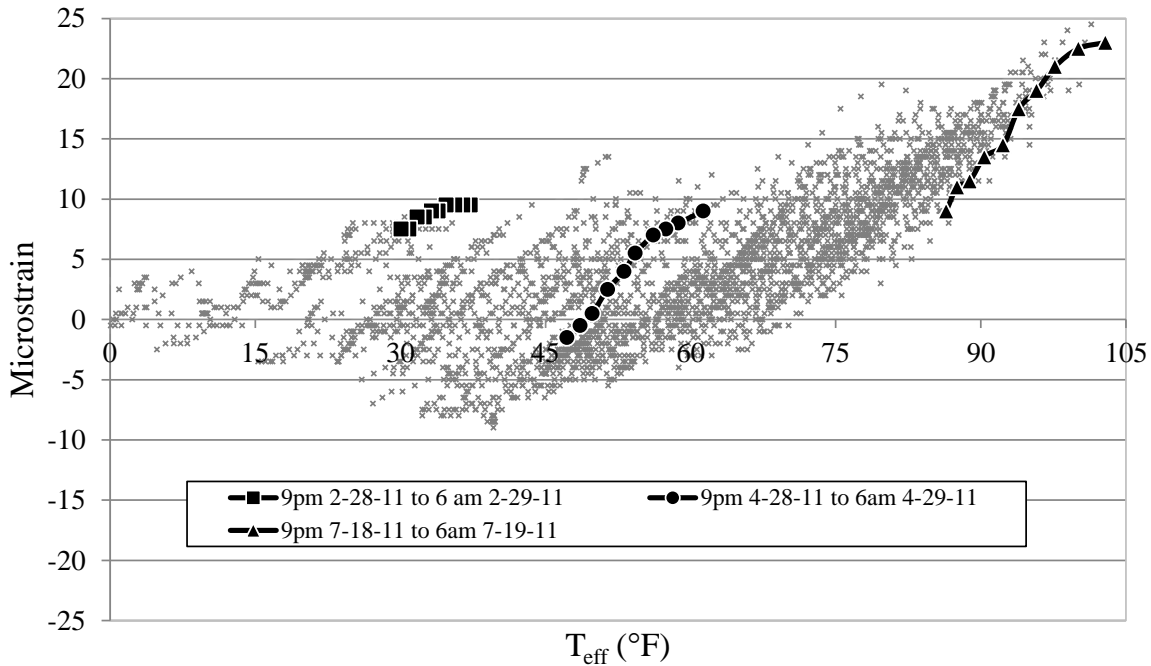
Figure 6.17. Bottom flange lateral bending versus T eff
