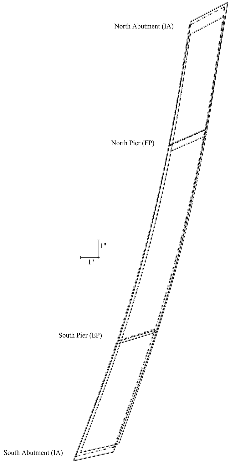
Figure 6.70. Bridge 2208 deflected shape
