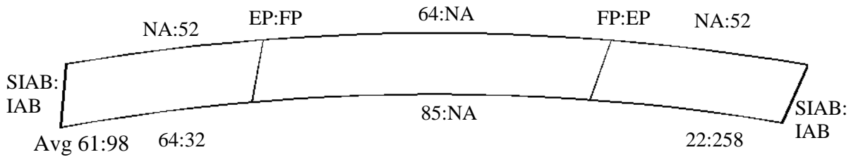
Figure 6.41. Bridge 209:2208 lateral bending strain bottom flange
