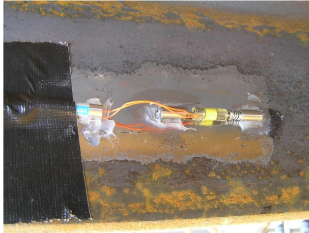
Figure 5.17. Vibrating-wire strain gauge
