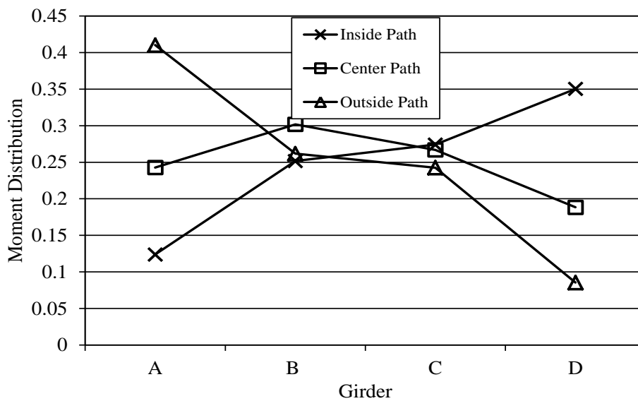
Figure 7.33. Bridge 309-S2 single lane moment distributions for three truck lanes
