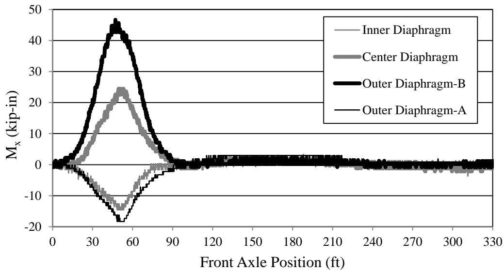
Figure 7.29. Bridge 309 strong axis moments in diaphragms (LP3)
