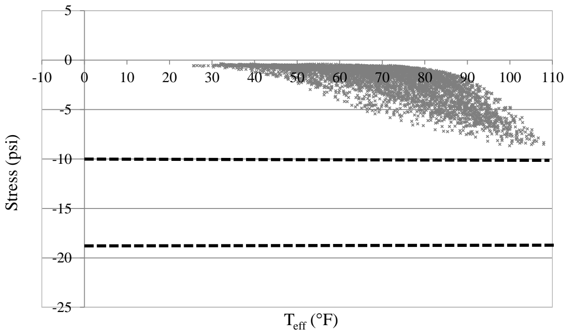
Figure 6.48. Northwest abutment backwall pressure versus effective temperature
