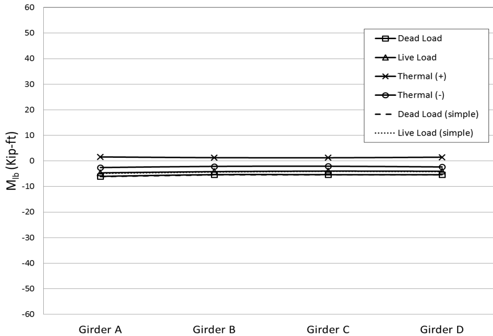
Figure 8.29. Center span Service I loads
