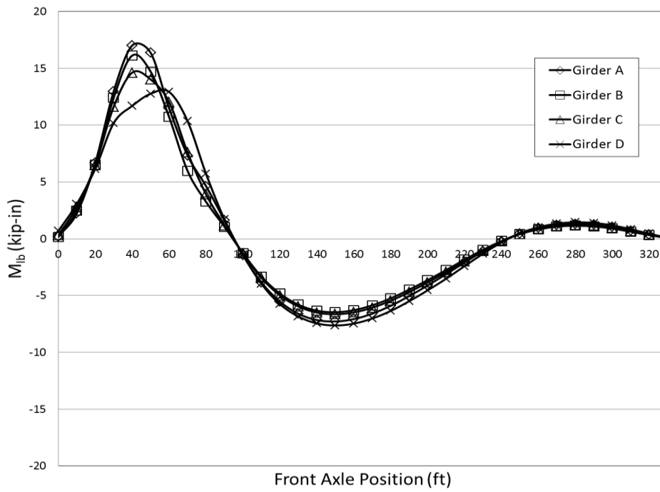
Figure 8.20. FEM center path at Section 2
