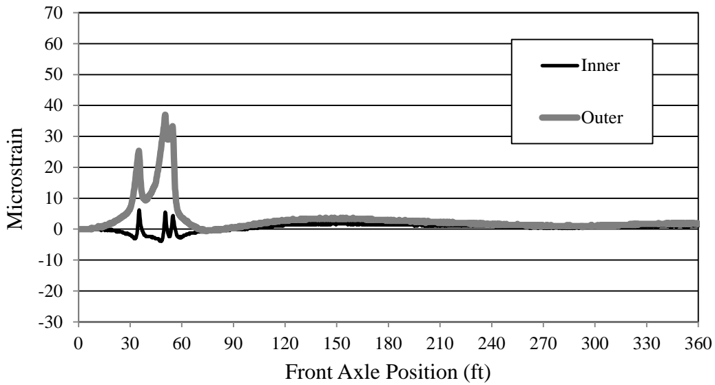
Figure 7.12. Girder B-S2 top flange strain (LP3)
