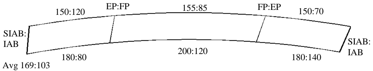
Figure 6.20. Bridge 209:2208 axial strain range
