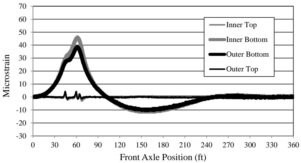
Figure 7.3. Bridge 309-S1 Girder C strain (LP2)
