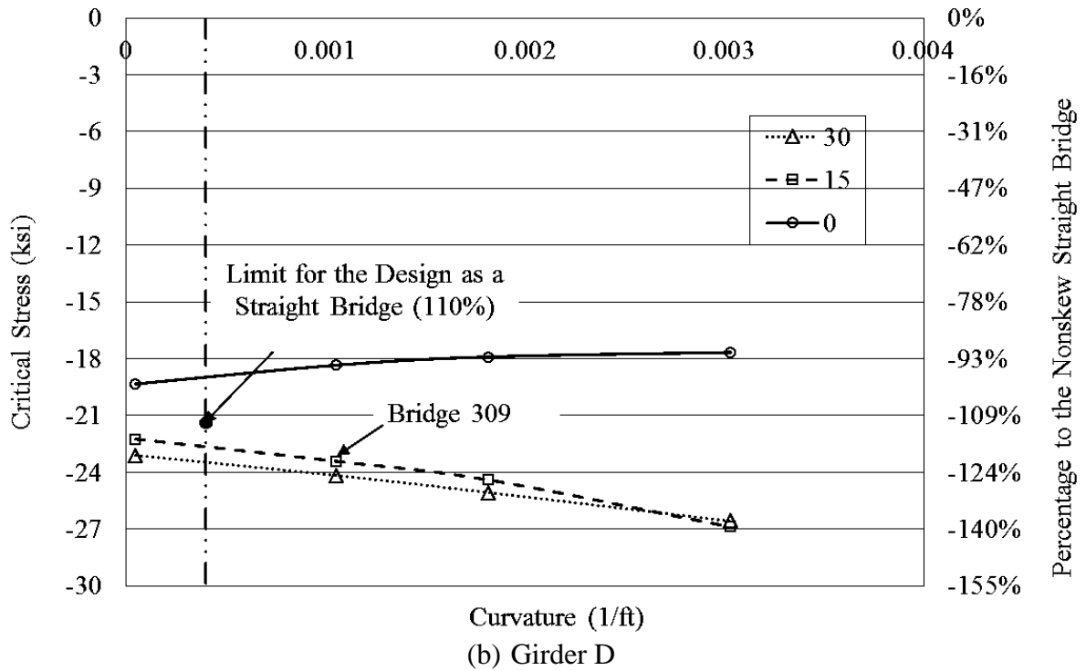
Figure 9.4. Critical stresses in Girder A and D at north pier with varying skew and curvature
