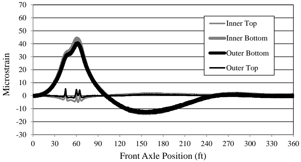
Figure 7.2. Bridge 309-S1 Girder B strain for (LP2)
