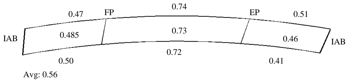
Figure 6.63. Bridge 2208 change in length per span
