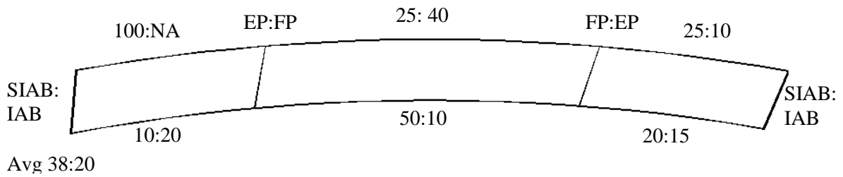
Figure 6.26. Bridge 209:2208 lateral bending strain top flange
