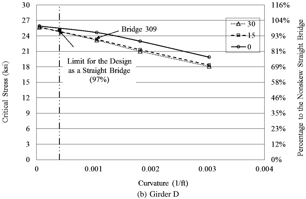
Figure 9.3. Critical stresses in Girder A and D at mid-center span with varying skew and curvature
