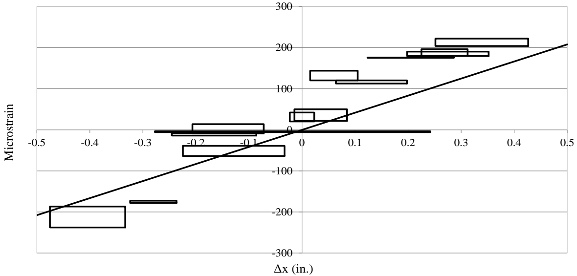
Figure 6.101. SAHP1 weak axis bending strain versus displacement
