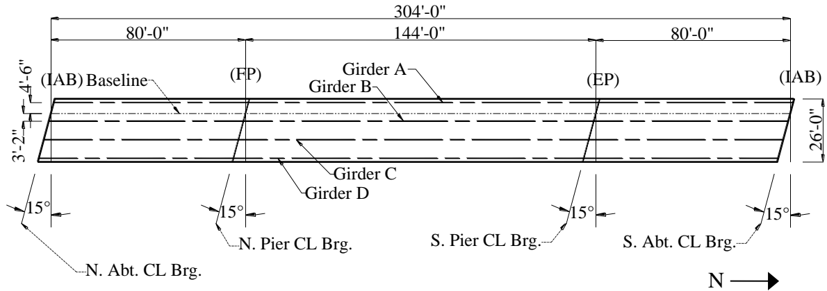
Figure 5.7. Bridge 2408 plan view
