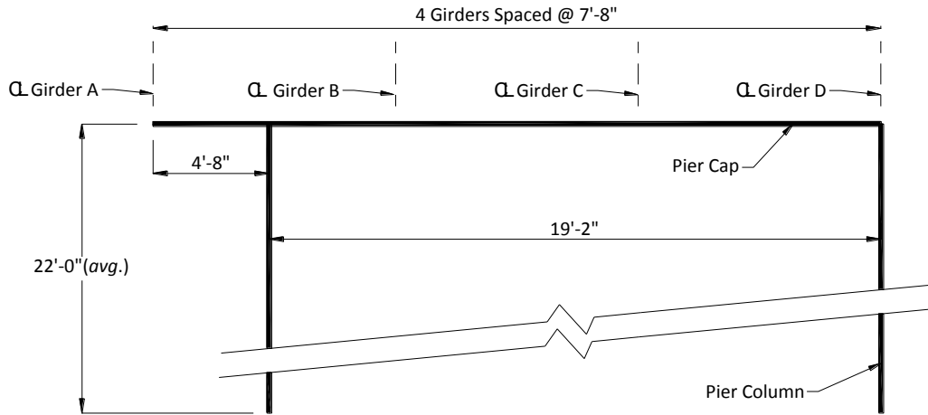
Figure 8.3. Typical pier geometry
