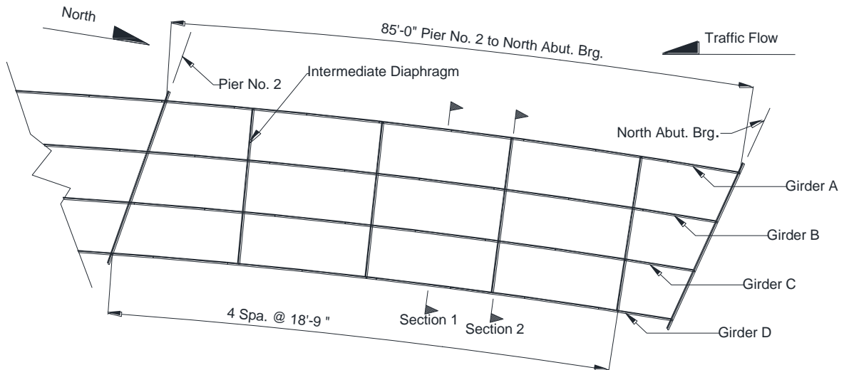
Figure 5.30. Bridge 309 plan view
