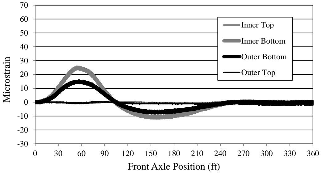
Figure 7.4. Bridge 309-S1 Girder D strain (LP2)
