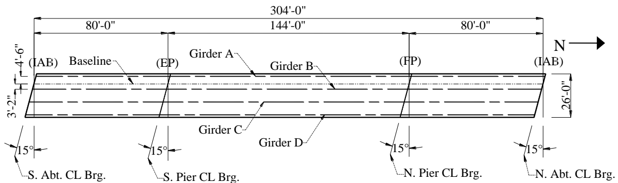
Figure 5.2. Bridge 109 plan view
