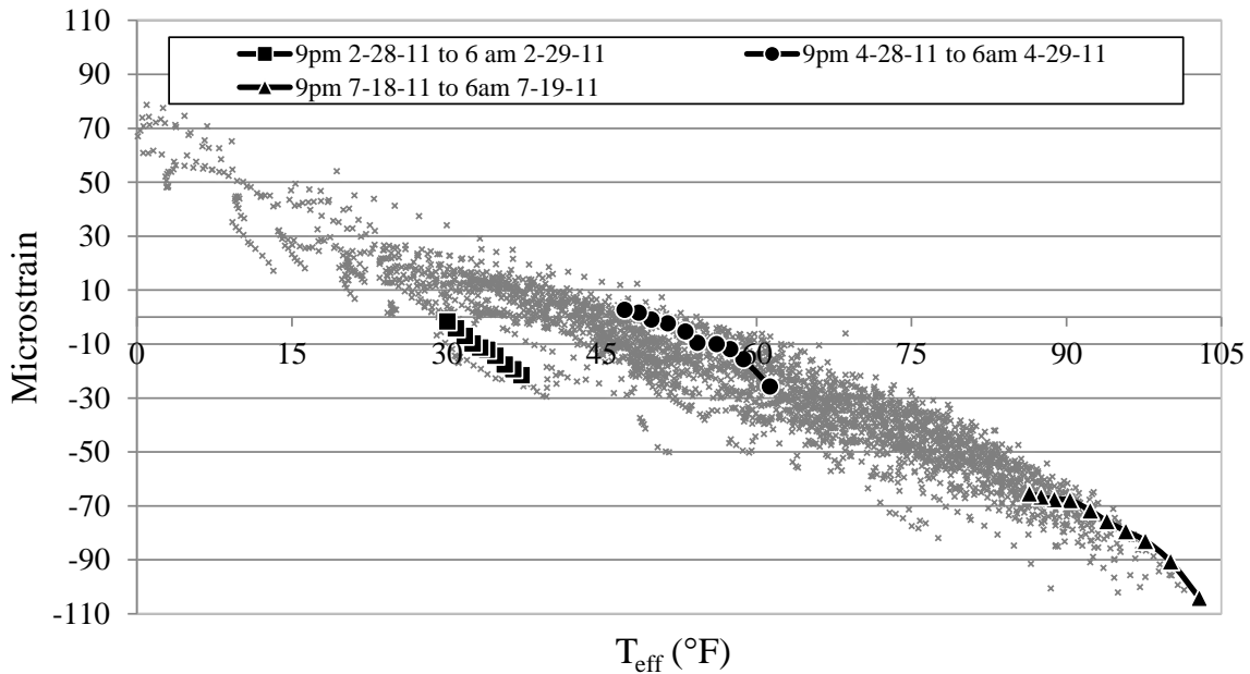
Figure 6.14. Axial strain versus T_{eff}
