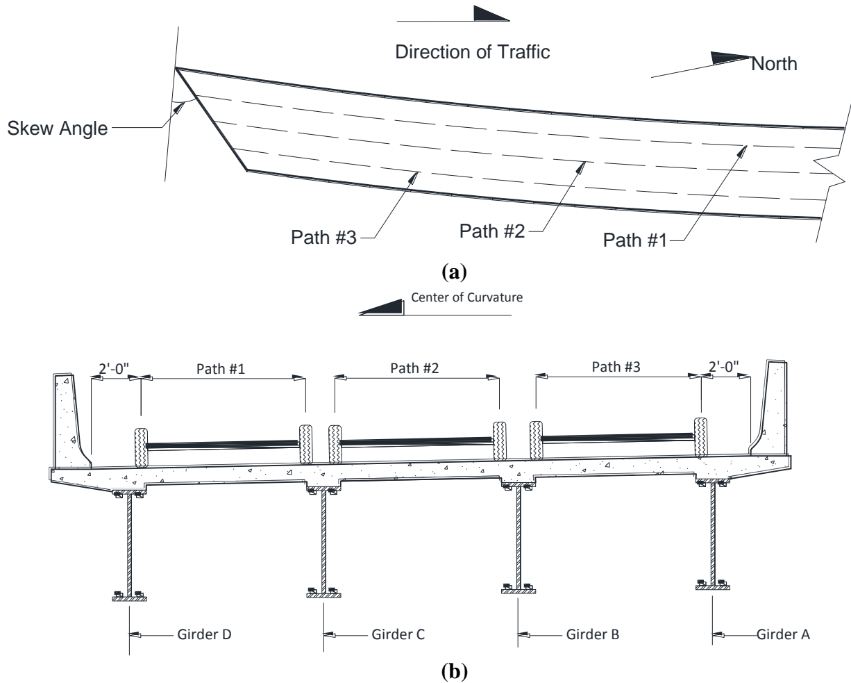
Figure 5.39. (a) Plan view and (b) cross section view of load path placement
