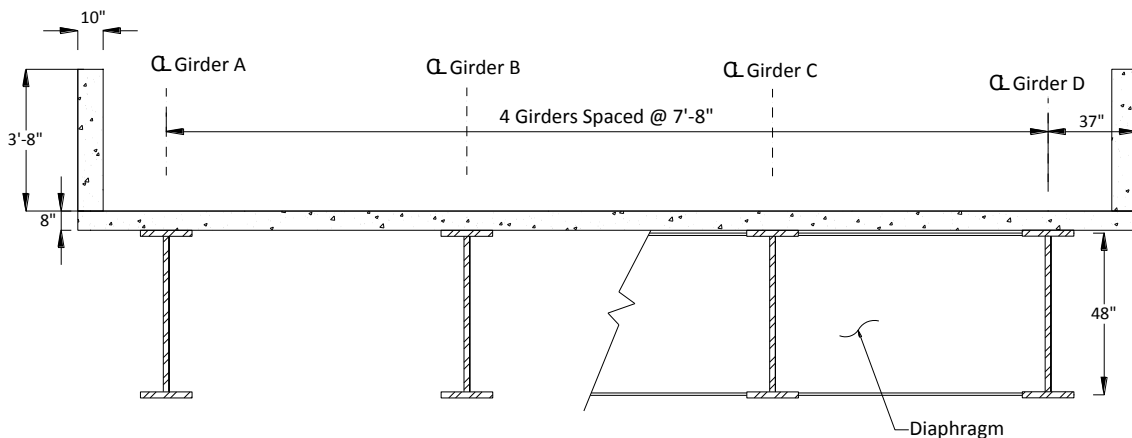
Figure 8.1. Model superstructure cross section
