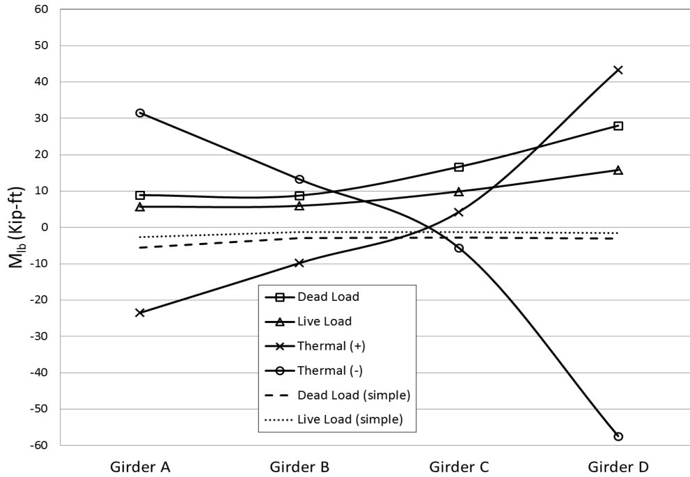
Figure 8.28. North pier Service I loads
