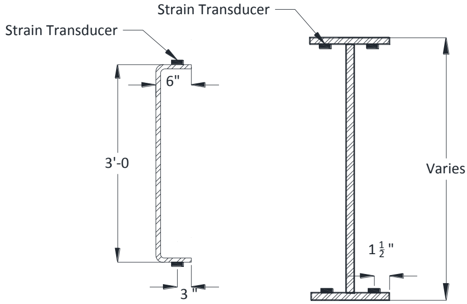
Figure 5.37. I-girder and diaphragm strain transducer detail
