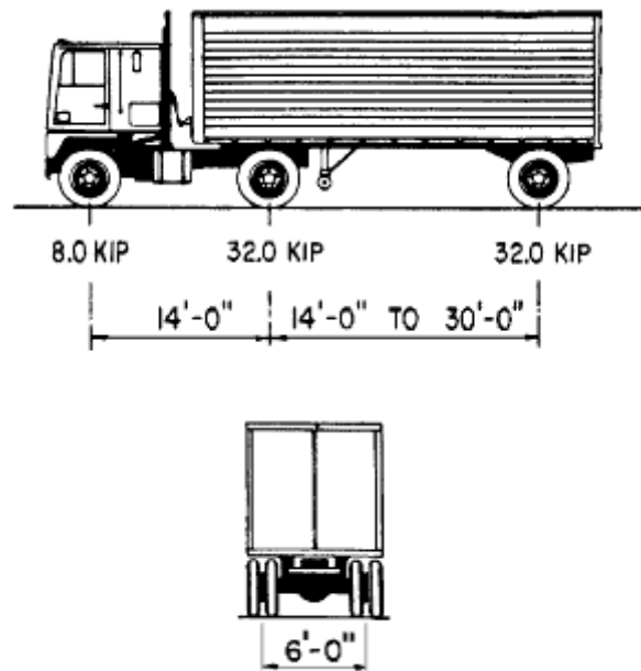
Figure 8.23. Design truck specifications (from Figure 3.6.1.2.2-1 AASHTO 2010)
