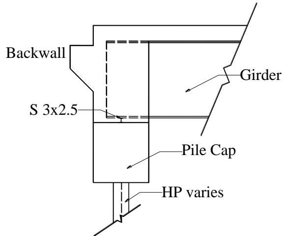
Figure 5.13. Integral abutment Section A-A
