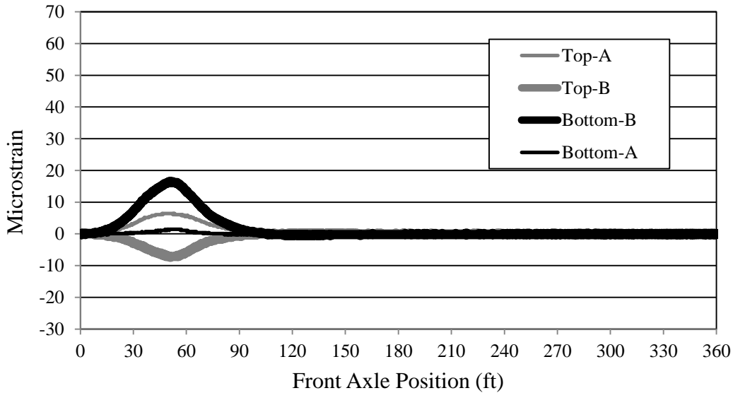
Figure 7.15. Bridge 309 outer diaphragm strain (LP2)
