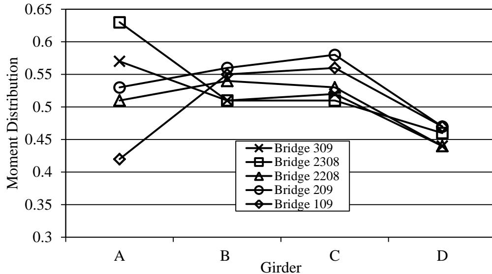
Figure 7.37. Maximum moment distribution factors in bridges
