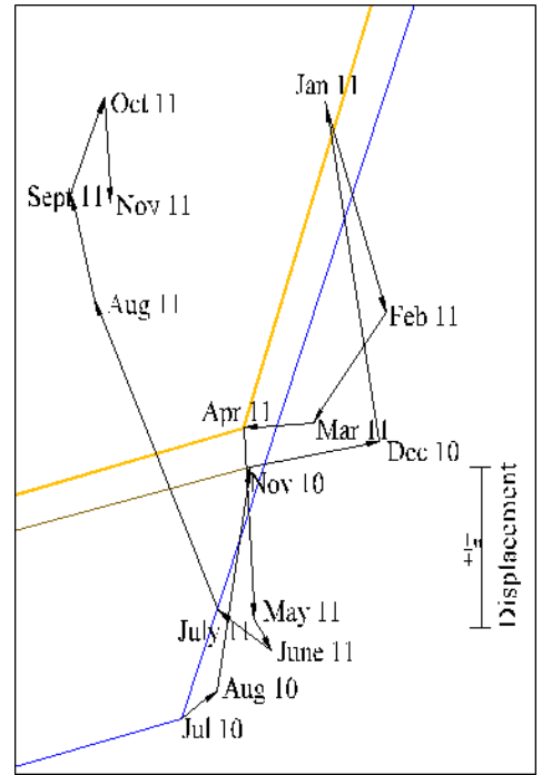
Figure 6.88. Bridge 2208 movement at south abutment west and east reflectors
