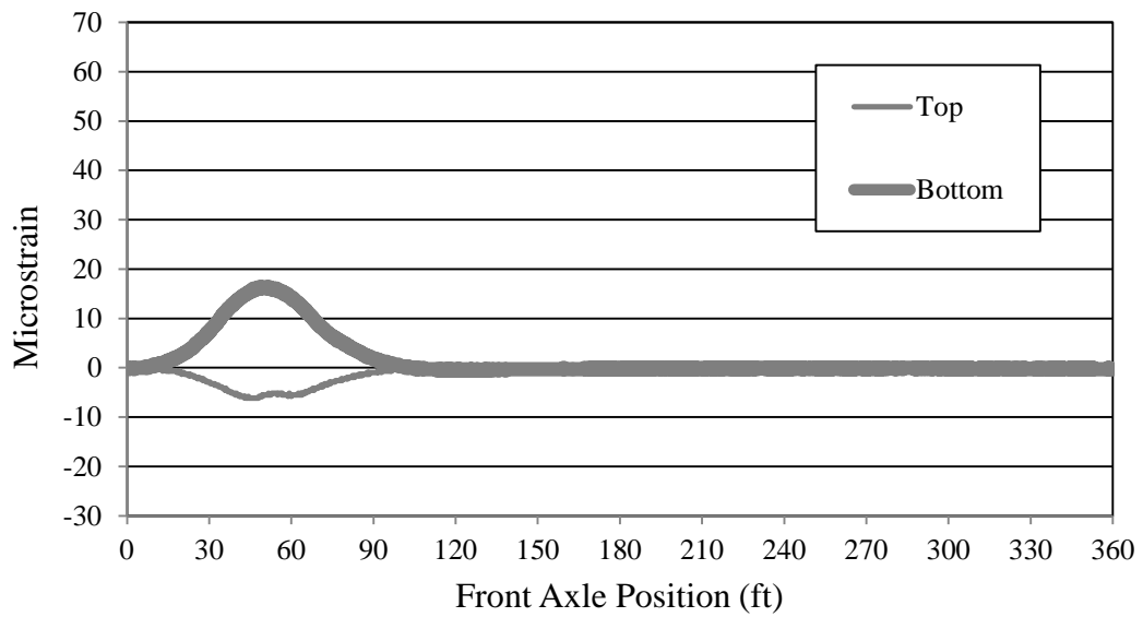
Figure 7.14. Bridge 309 center diaphragm strain (LP2)
