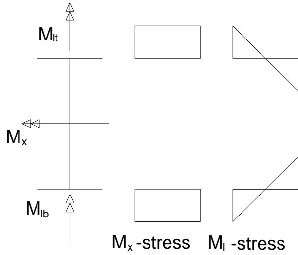
Figure 2.3. Normal stress in flanges due to major axis bending and lateral bending
