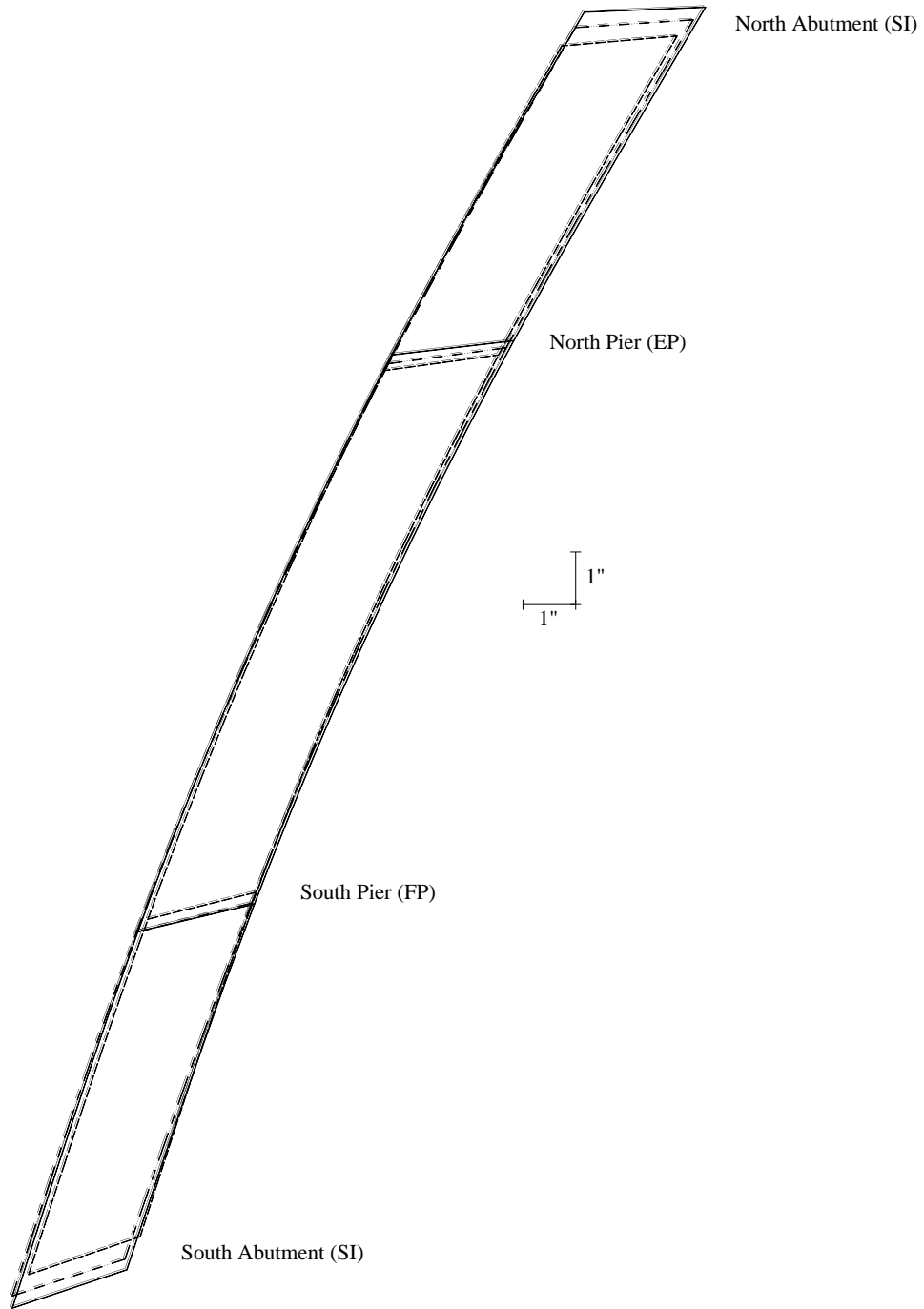
Figure 6.68. Bridge 209 deflected shape
