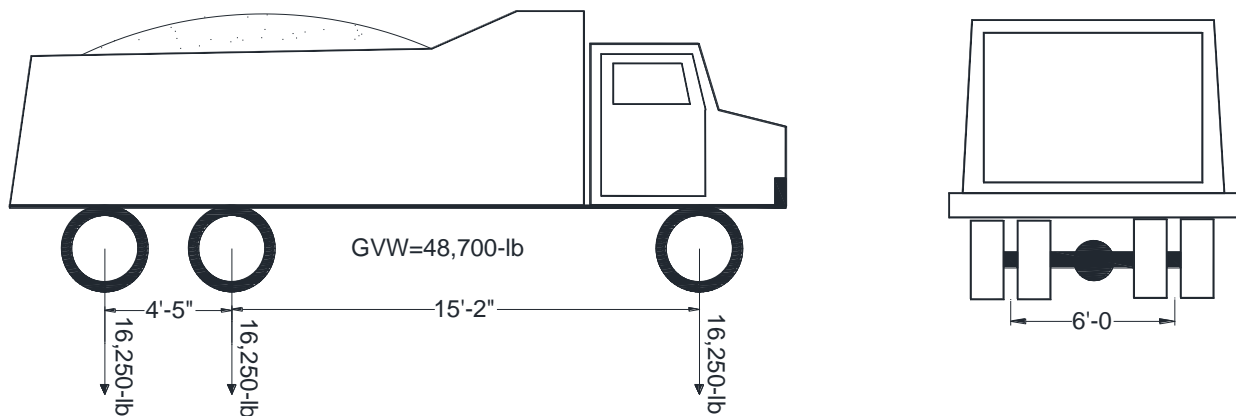
Figure 5.38 Truck configuration and loading
