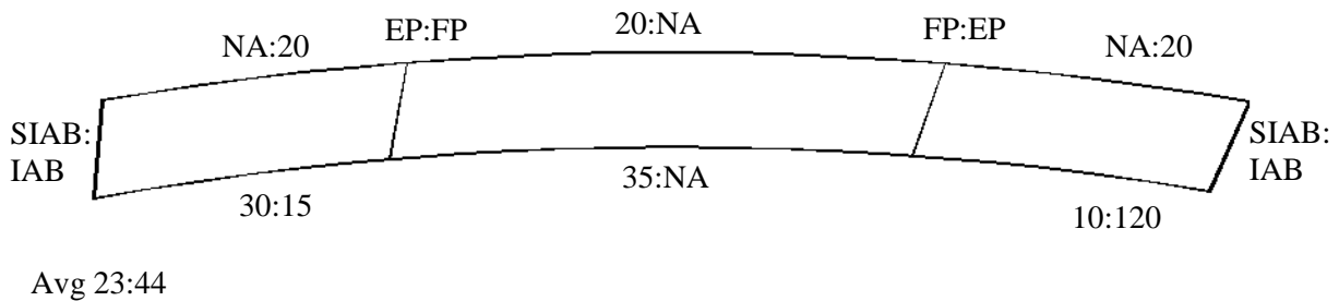
Figure 6.29. Bridge 209:2208 lateral bending strain bottom flange
