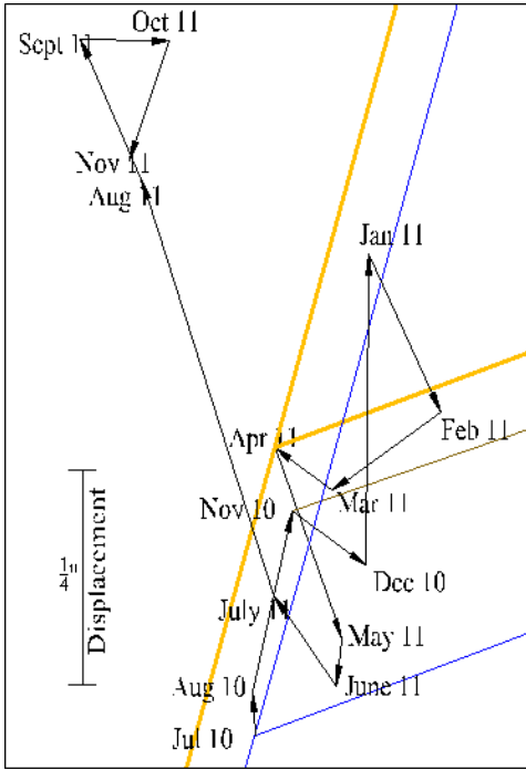
Figure 6.87. Bridge 2208 movement at south pier west and east reflectors
