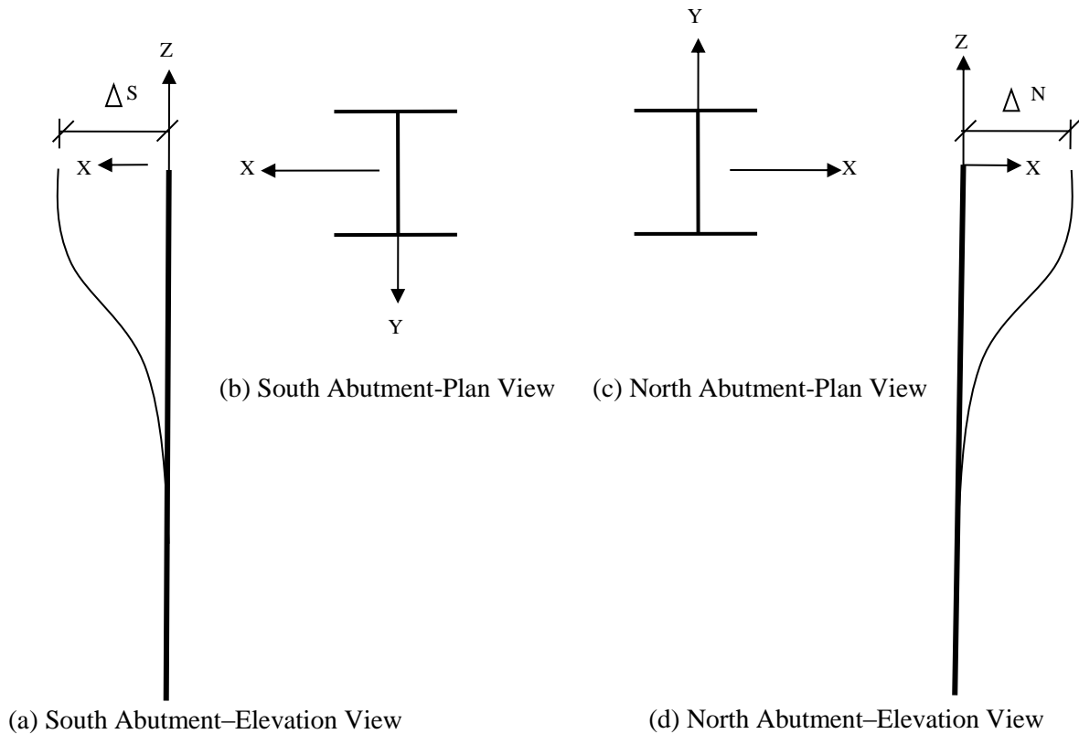
Figure 5.16. Integral Abutment pile coordinate system for Bridge 309
