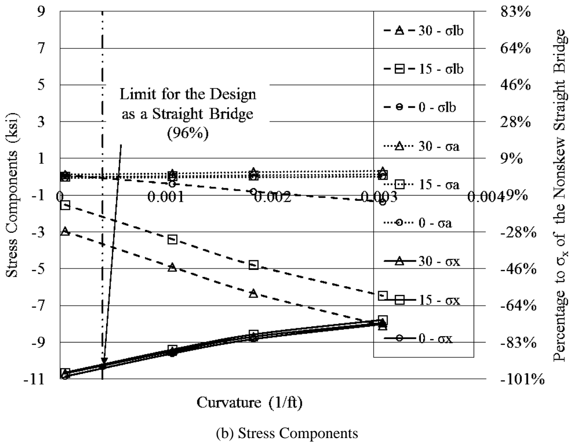
Figure 9.12. Total and component stresses in Girder D at north pier due to DL
