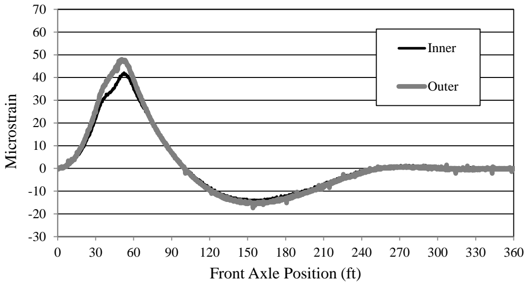
Figure 7.10. Bridge 309-S2 Girder A bottom flange strain (LP3)
