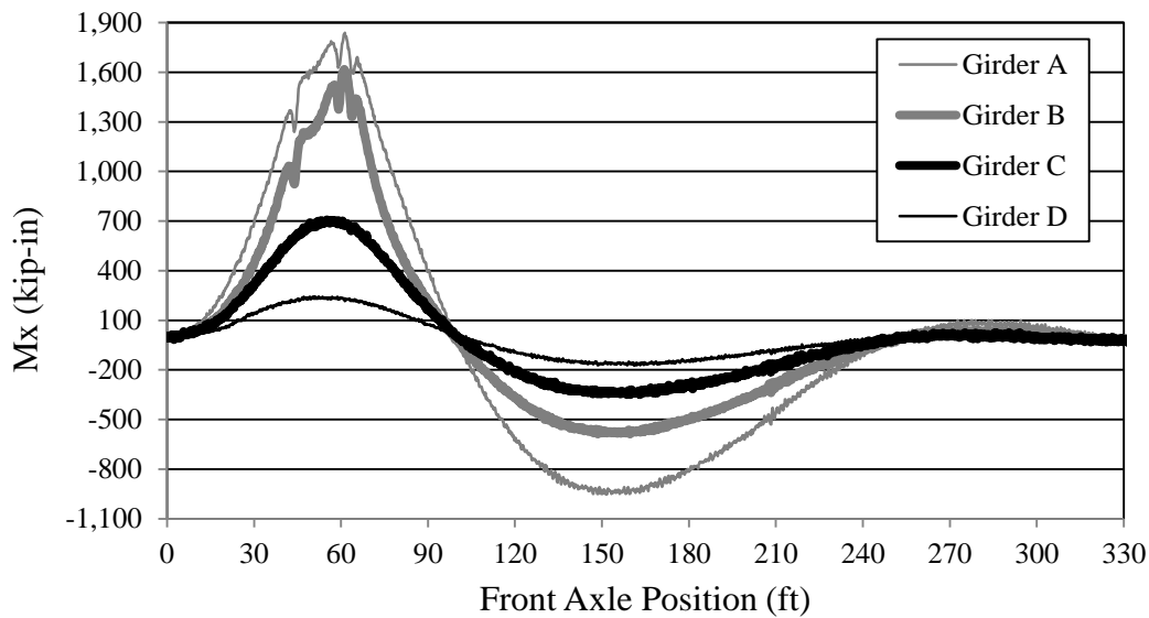
Figure 7.23. Bridge 309-S1 strong axis moments in girders (LP3)
