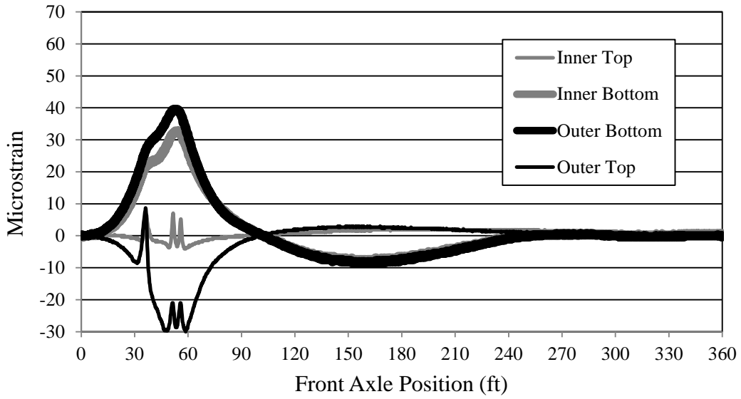
Figure 7.6. Bridge 309-S2 Girder B strain (LP2)
