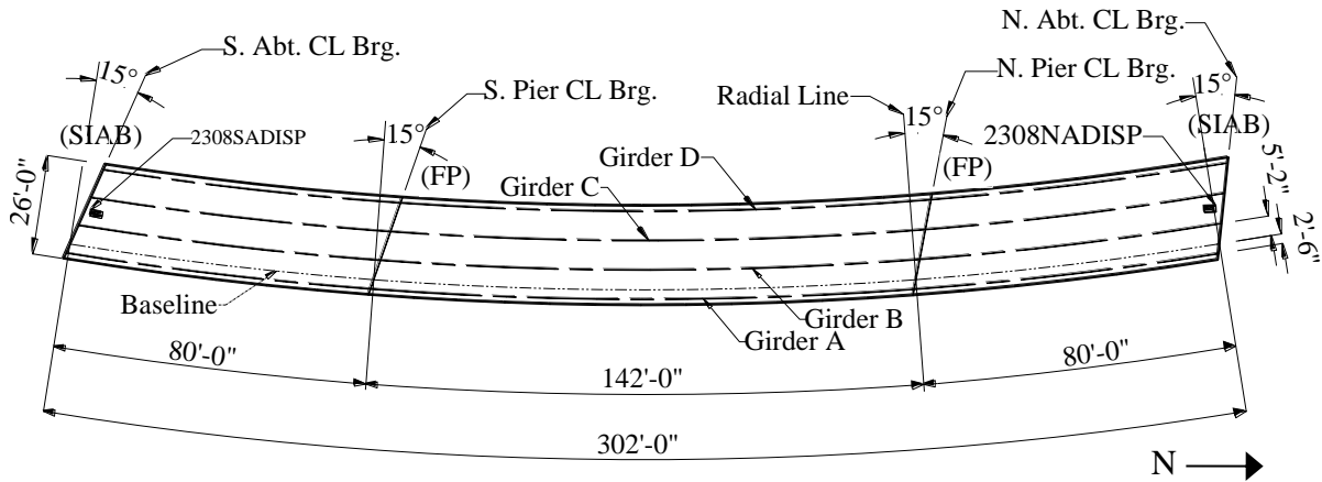
Figure 5.6. Bridge 2308 plan view
