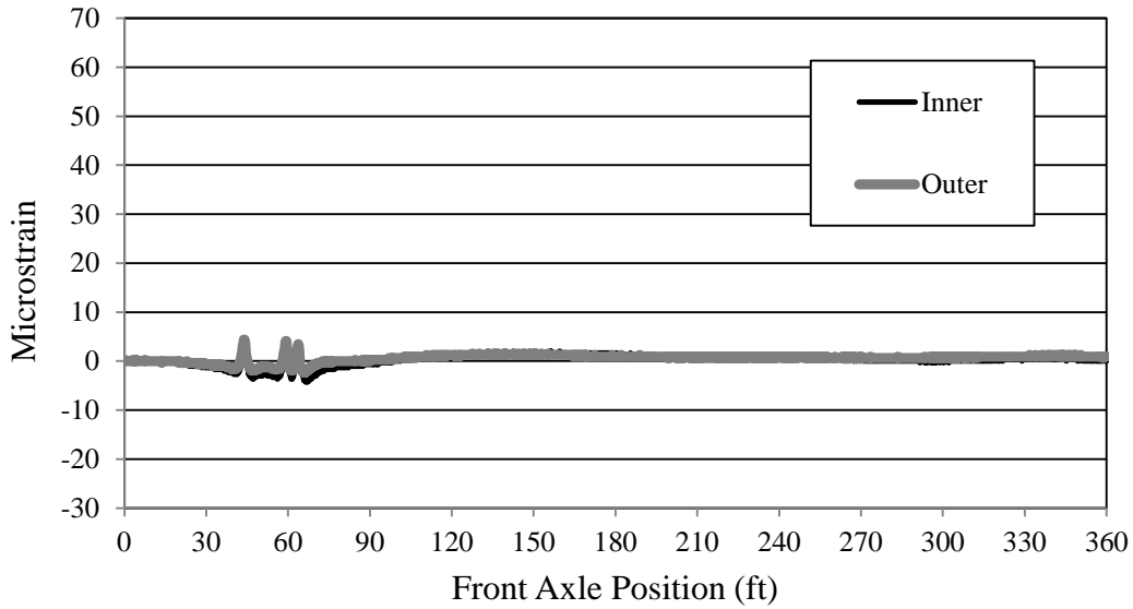
Figure 7.11. Bridge 309-S1 Girder B top flange strain (LP3)
