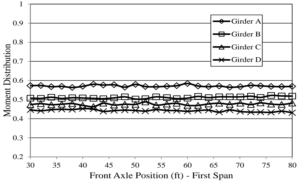
Figure 7.34. Bridge 309-S1 moment distributions versus truck position
