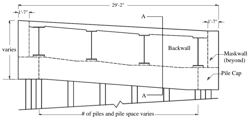
Figure 5.12. Integral abutment – front elevation
