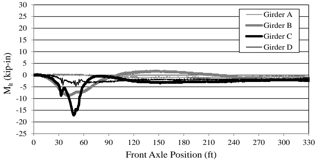
Figure 7.26. Bridge 309-S2 lateral top flange moments (LP3)
