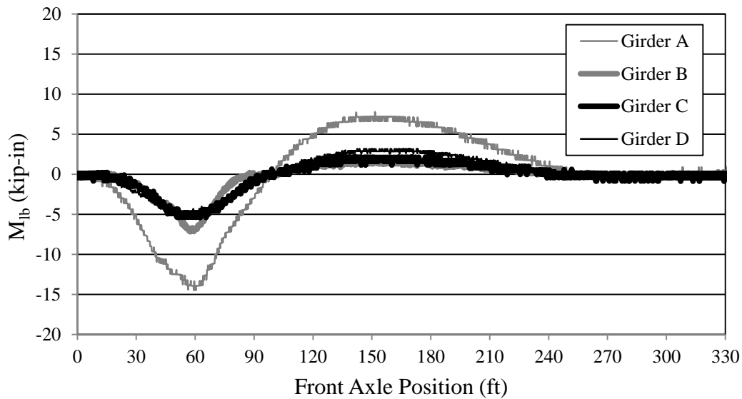
Figure 7.24. Bridge 309-S1 lateral bottom flange moments (LP3)
