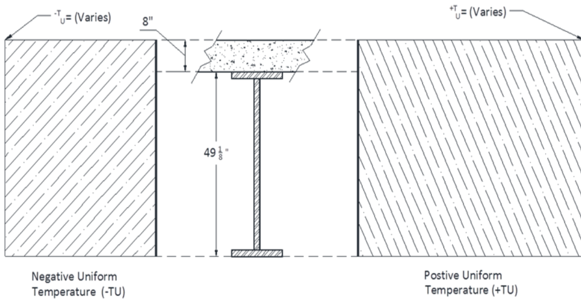
Figure 8.24. Uniform temperature distribution
