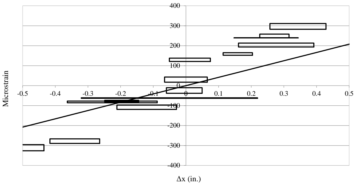
Figure 6.104. NAHP1 weak axis bending strain versus displacement
