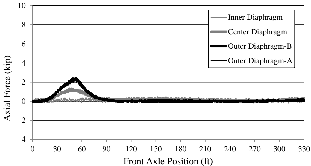
Figure 7.30. Bridge 309 axial forces in diaphragms (LP3)
