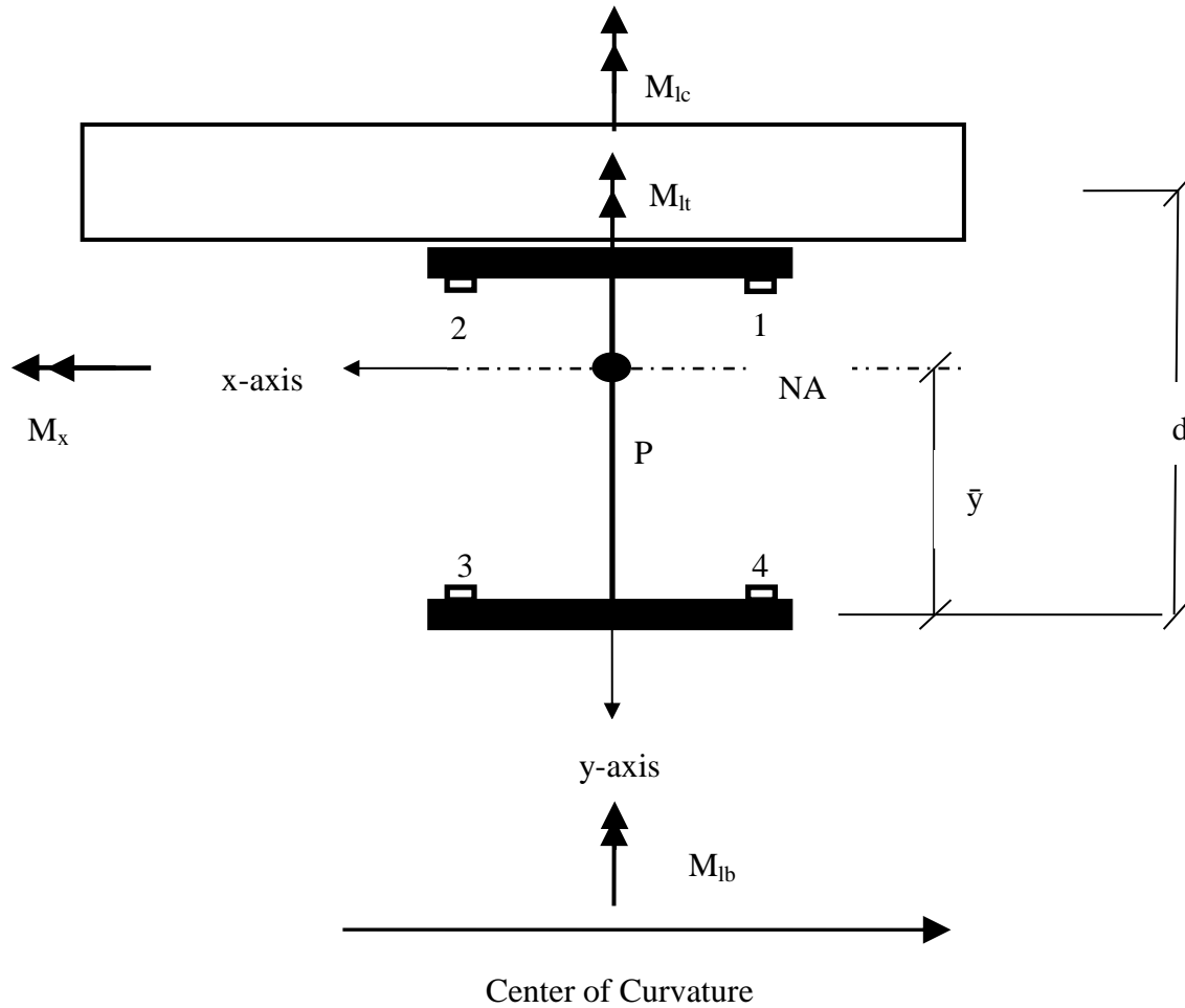
Figure 6.4. Resolved girder forces
