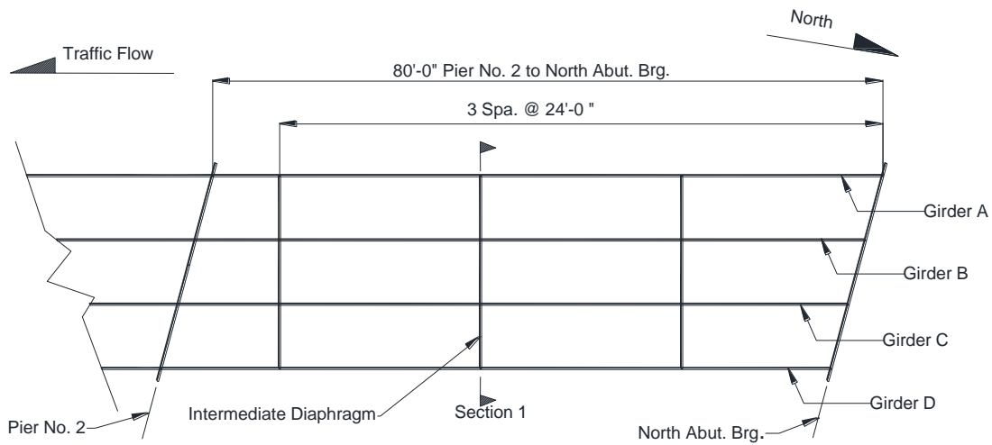
Figure 5.34. Bridge 109 plan view
