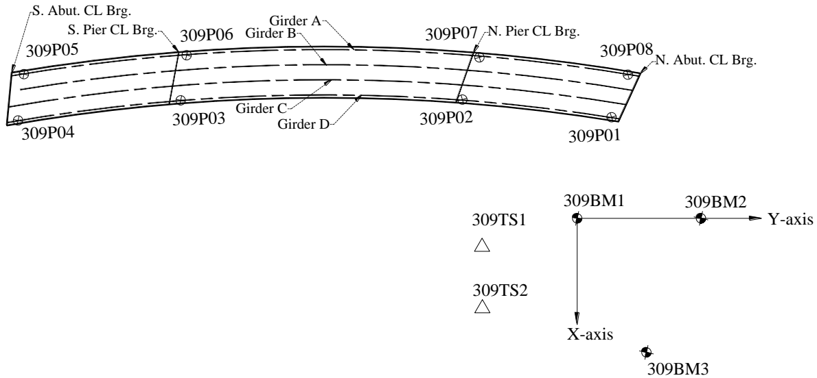
Figure 5.28. Bridge 309 reflector, TS, and BM locations
