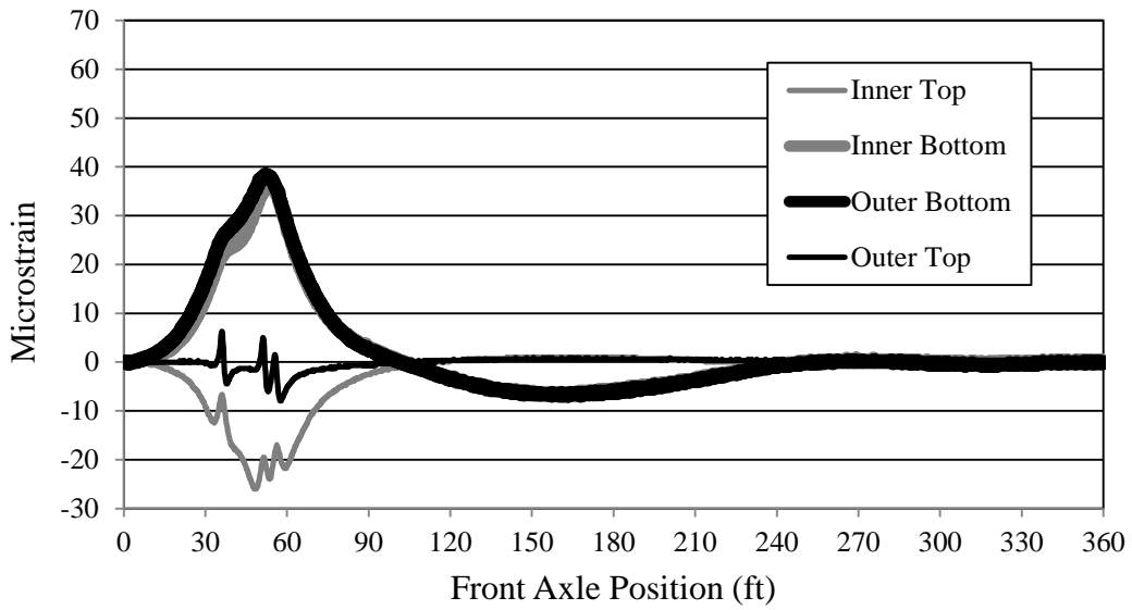
Figure 7.7. Bridge 309-S2 Girder C strain (LP2)
