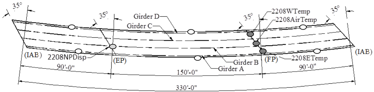
Figure 5.24. Bridge 2208 instrumentation
