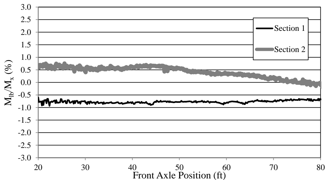
Figure 7.38. Bridge 309 Girder A ratio of M_{lb}/M_x
