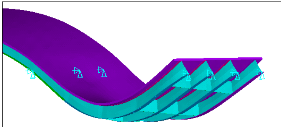
Figure 8.17. Deflected shape for center truck position
