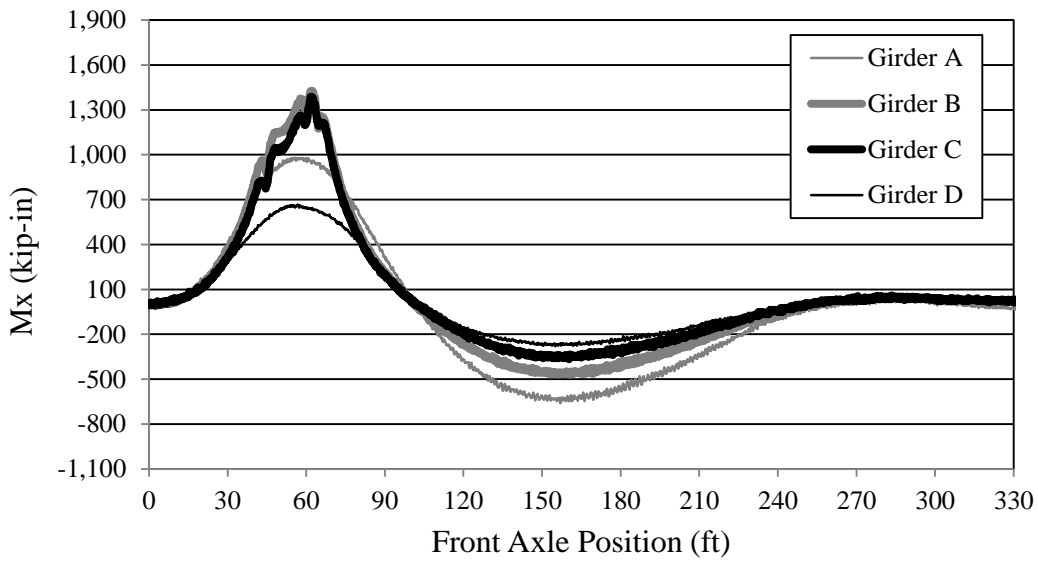
Figure 7.22. Bridge 309-S1 strong axis moments in girders (LP2)
