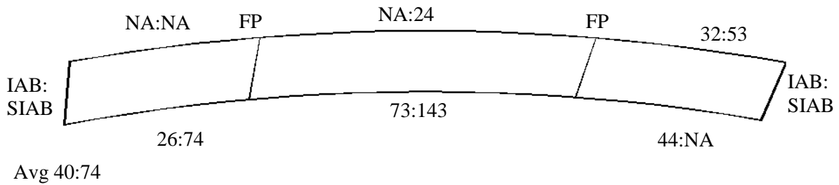
Figure 6.40. Bridge 309:2308 lateral bending strain bottom flange
