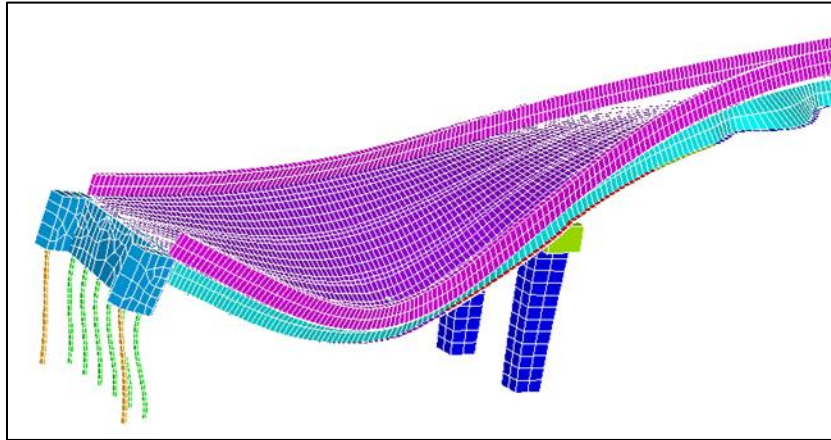
Figure 8.13. Deflected shape for outer truck position
