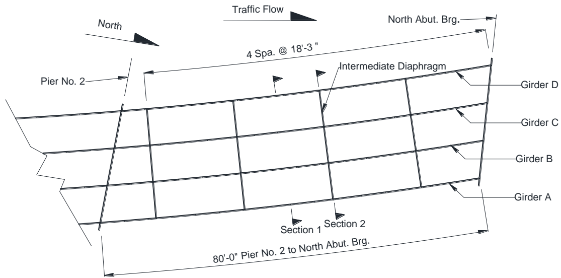
Figure 5.33 Bridge 2308 plan view
