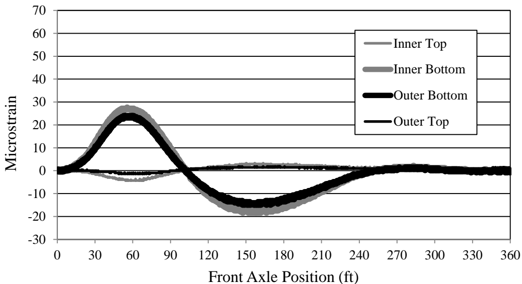
Figure 7.1. Bridge 309-S1 Girder A strain (LP2)
