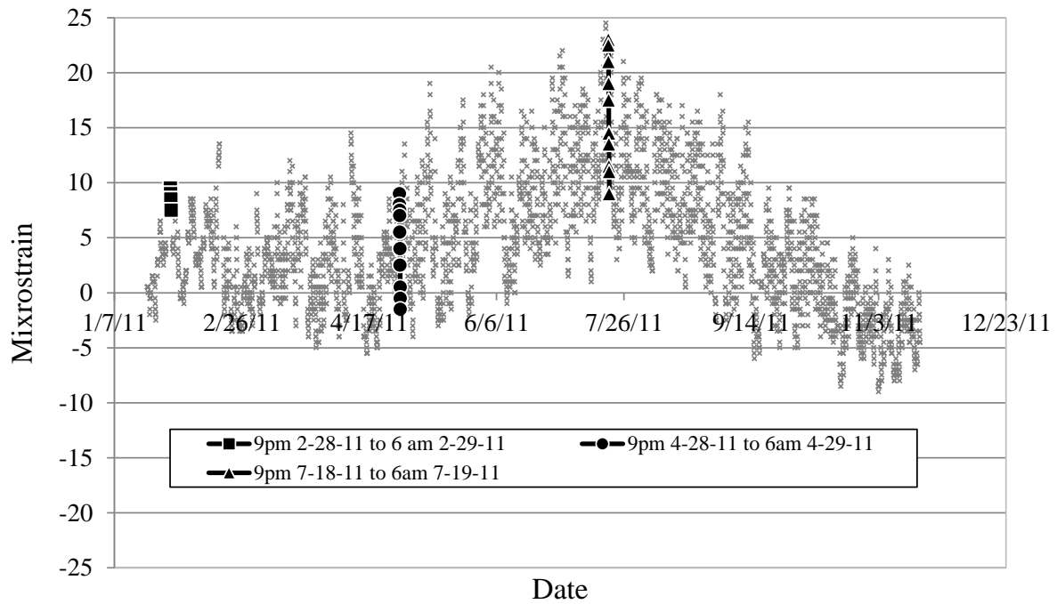
Figure 6.13. Bottom flange lateral bending versus time
