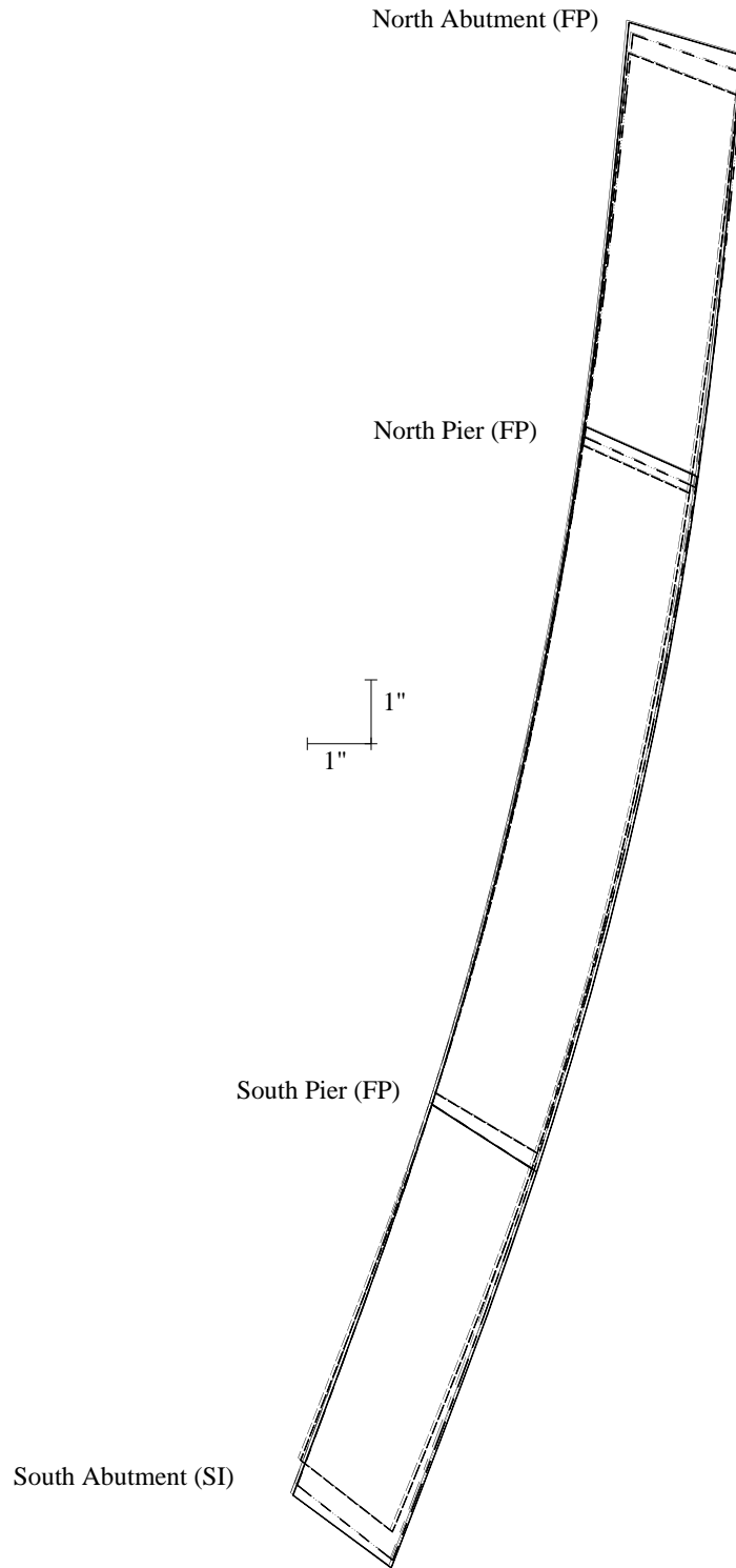
Figure 6.71. Bridge 2308 deflected shape
