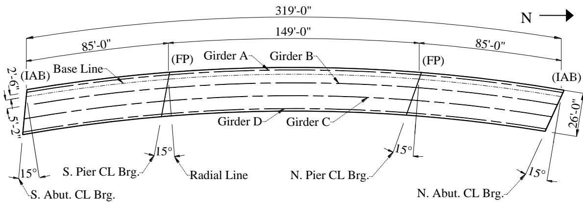
Figure 5.4. Bridge 309 plan view
