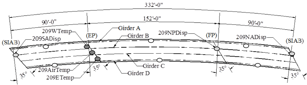
Figure 5.22. Bridge 209 instrumentation
