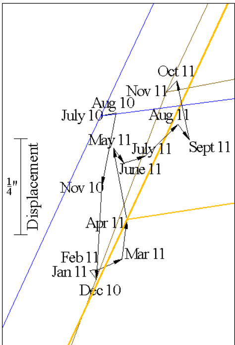
Figure 6.78. Bridge 209 movement at north pier west and east reflectors
