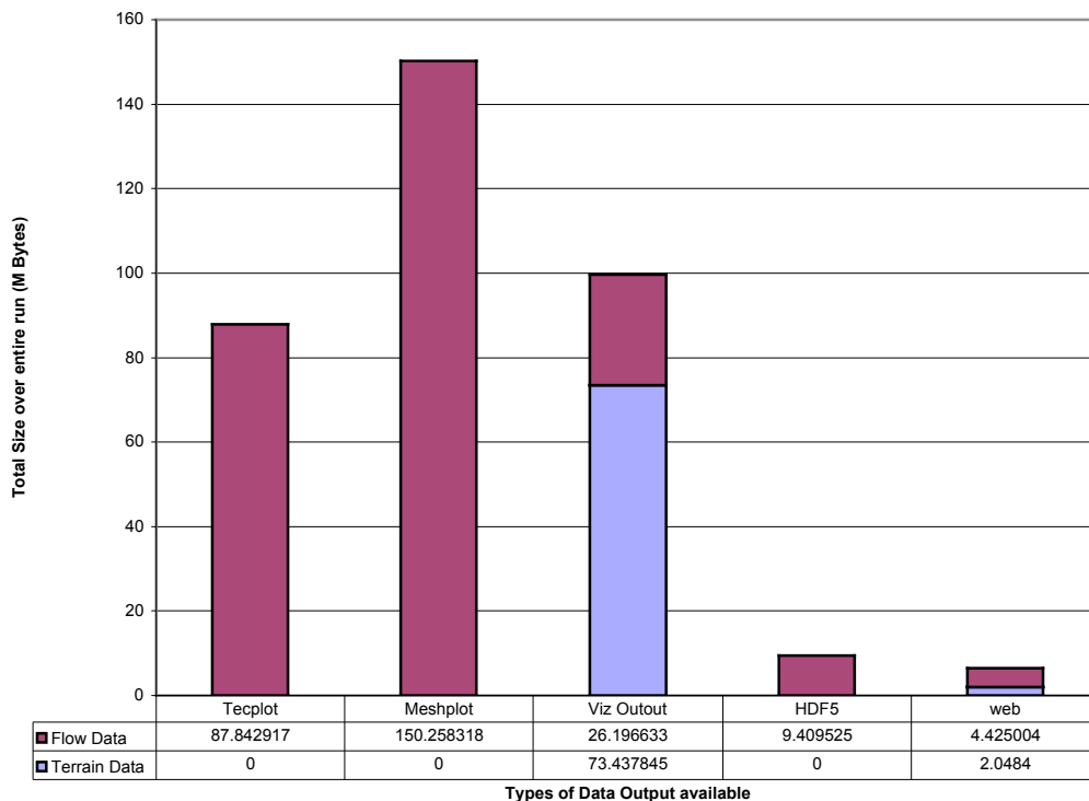
Figure 6 - Comparison of total size of output generated by each type.
