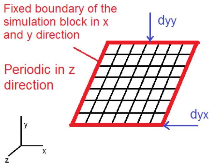
Figure 7.9. Indentation loading
